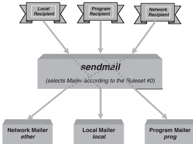
FIGURE 20.3 Sendmail vs. mailers relations.
