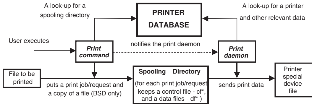
FIGURE 10.1 Functional diagram of a printing subsystem.
