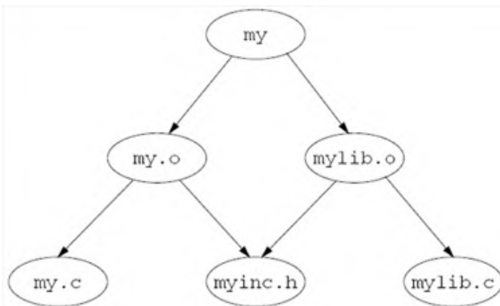
Figure A.2. A dependency graph for the makefile of Example A.18 .
