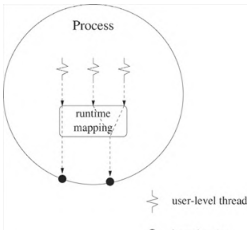
Figure 12.5. Hybrid model has two levels of scheduling, with user-level threads mapped into kernel entities.
