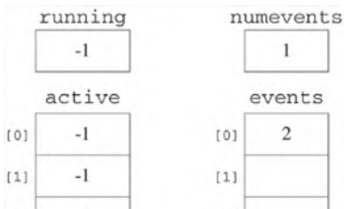
Figure 10.4. The timers data structure after timer [2] expires.
