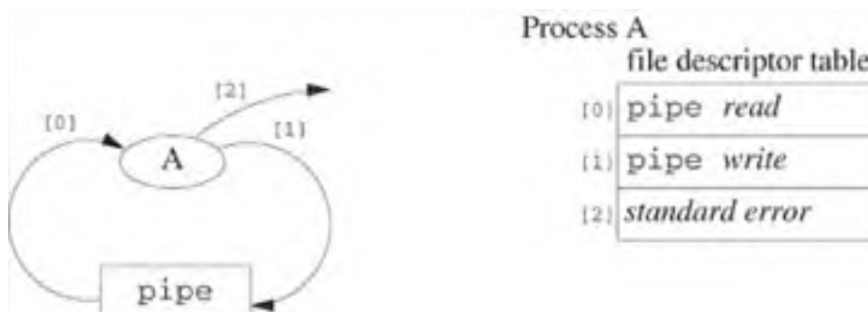
Figure 7.4. Status of the process at the end of Example 7.1 .
