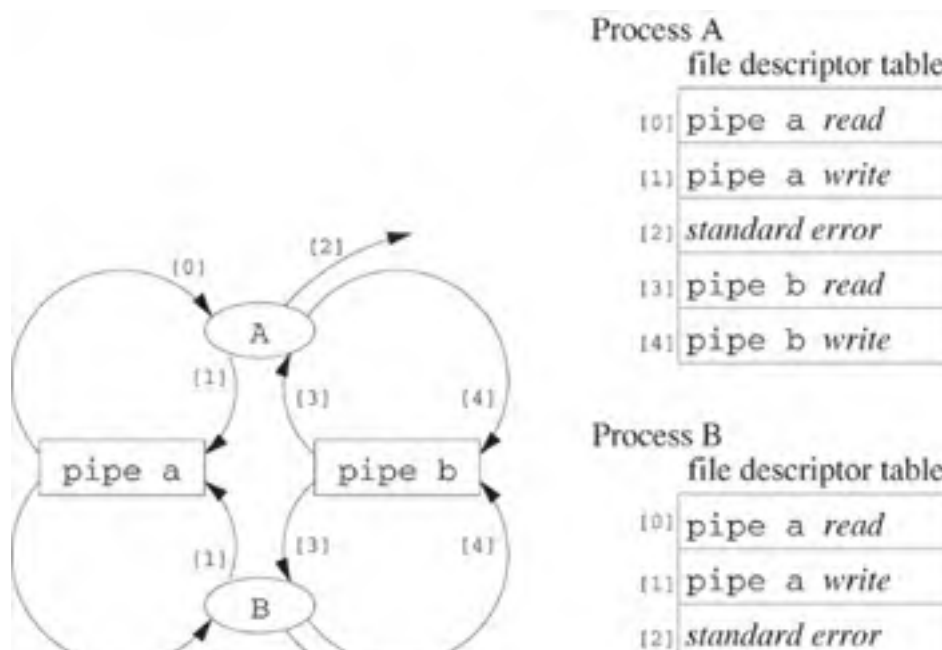
Figure 7.6. Connections of the processes of Example 7.5 after the fork . Process A is the parent and process B is the child.
