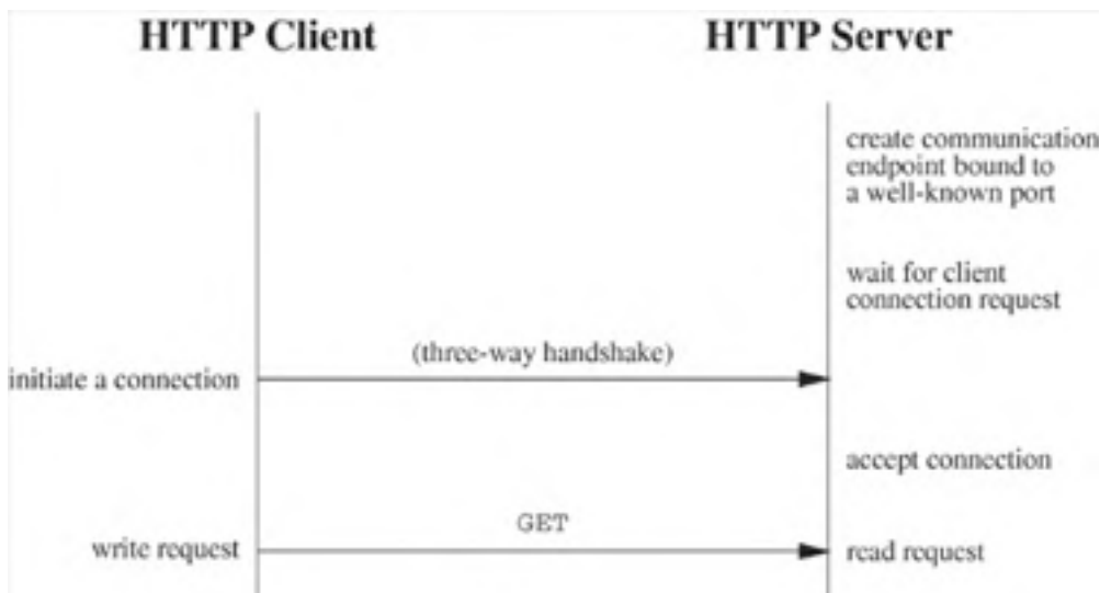
Figure 19.3. Sequence of steps in HTTP 1.0 communication.
