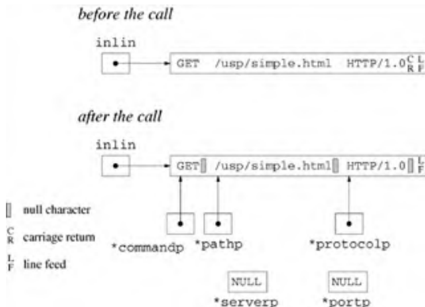
Figure 19.10. The parse function parses an absolute path form of the initial line in place.
