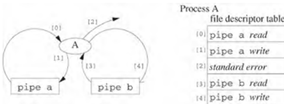
Figure 7.5. Connections to the parent process of Example 7.5 after the second pipe(fd) call executes.
