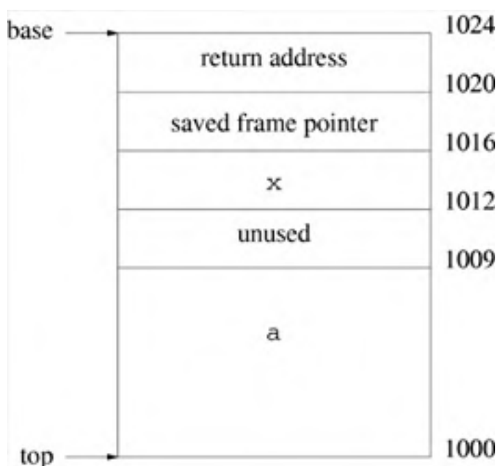
Figure 1.1. Possible stack layout for the checkpass function of Program 1.1.
