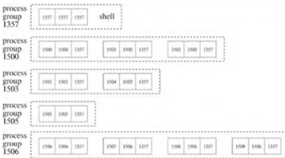
Figure 11.1. Five process groups for session 1357.
