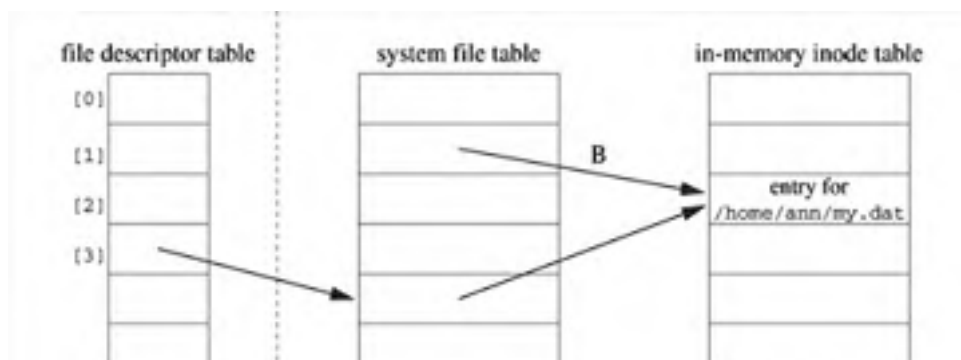
Figure 4.2. Schematic diagram of the relationship between the file descriptor table, the system file table and the in-memory inode table in a UNIX-like operating system after the code of Example 4.20 executes.
