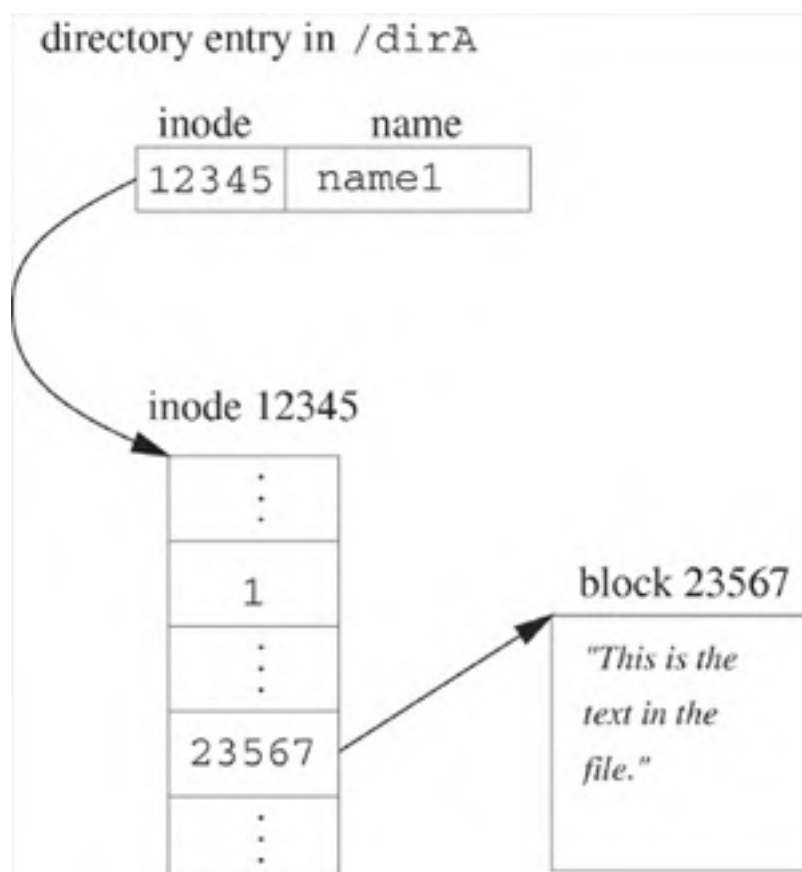
Figure 5.4. Directory entry, inode and data block for a simple file.
