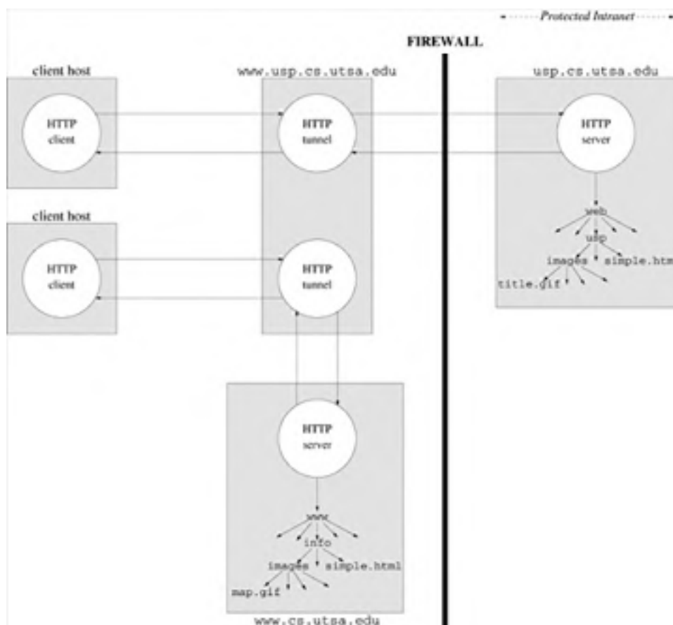
Figure 19.9. The server www.usp.cs.utsa.edu acts as a gateway for servers inside and outside the firewall.
