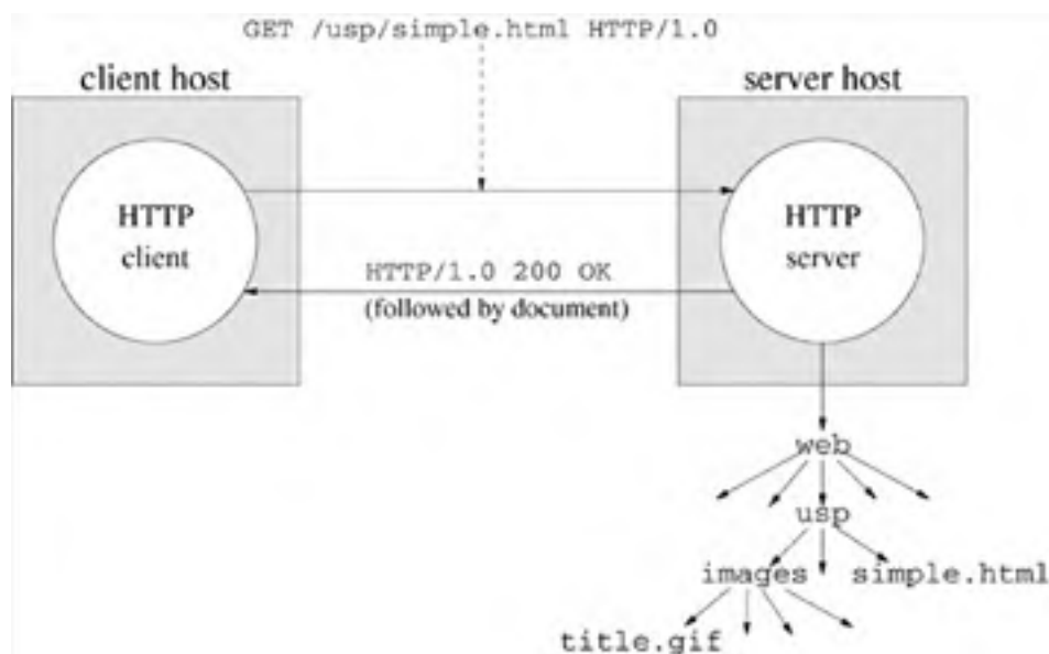
Figure 19.2. Schematic of an HTTP 1.0 transaction.
