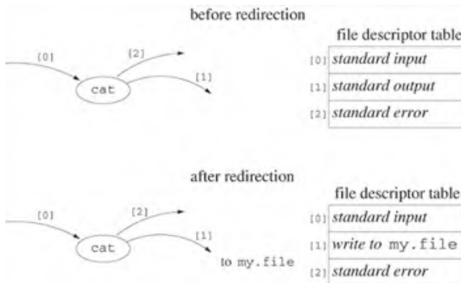
Figure 4.6. Status of the file descriptor table before and after redirection for the process that is executing cat > my.file .
