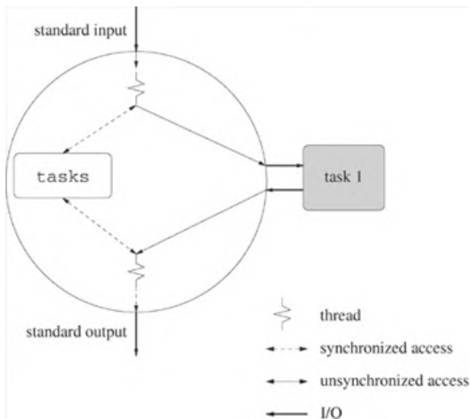
Figure 17.8. Schematic of a threaded NTPVM dispatcher for a single task.
