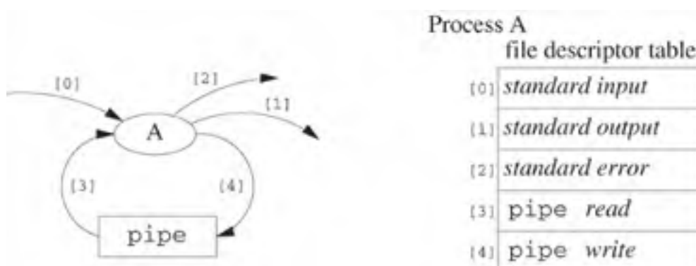
Figure 7.2. Status of the process of Example 7.1 after pipe(fd) executes.
