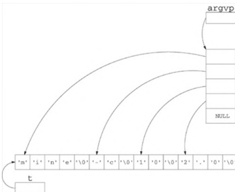
Figure 2.4. The makeargv parses the tokens in place by using strtok .
