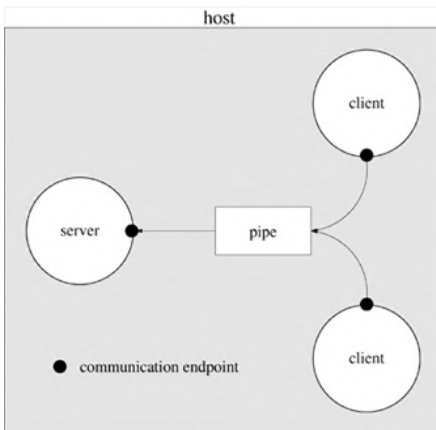
Figure 18.1. Multiple clients write requests to a shared one-way communication channel.
