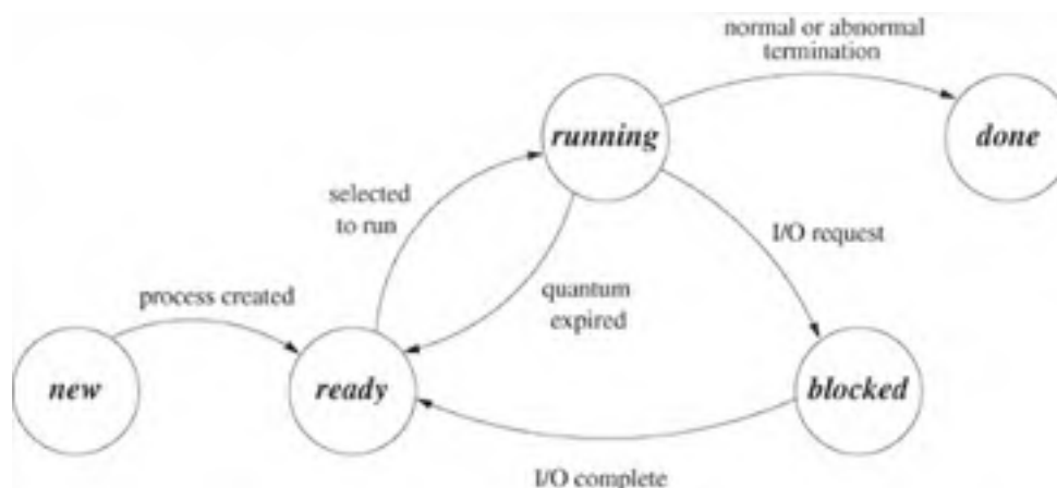
Figure 3.1. State diagram for a simple operating system.
