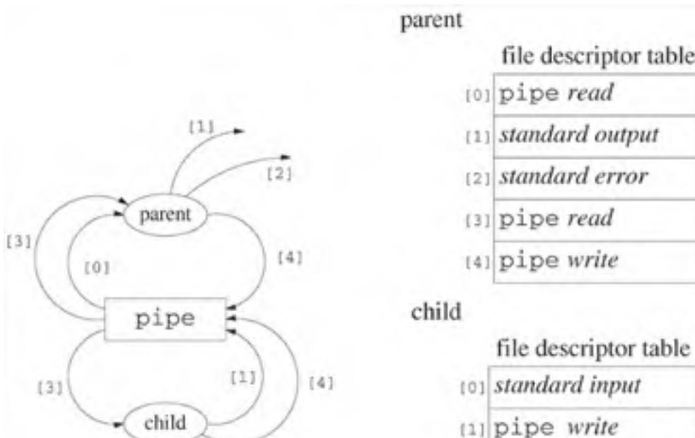
Figure 6.3. Status of the file descriptor table after both dup2 functions of Program 6.3.
