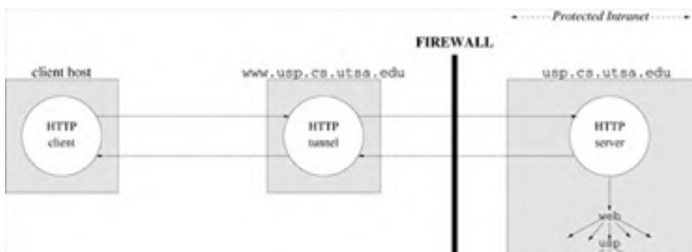
Figure 19.5. Tunnels provide a controlled portal through a firewall.
