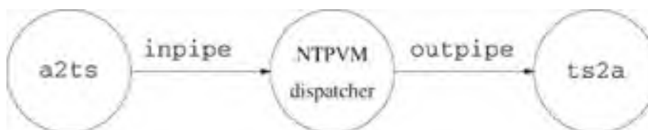
Figure 17.7. Logical process layout for debugging the dispatcher.
