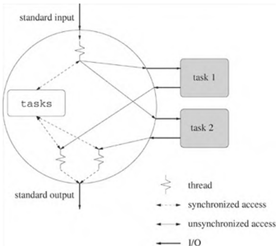
Figure 17.9. Schematic of a threaded NTPVM dispatcher.
