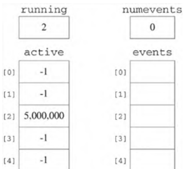
Figure 10.3. The timers data structure after timer [2] has been set for five seconds.
