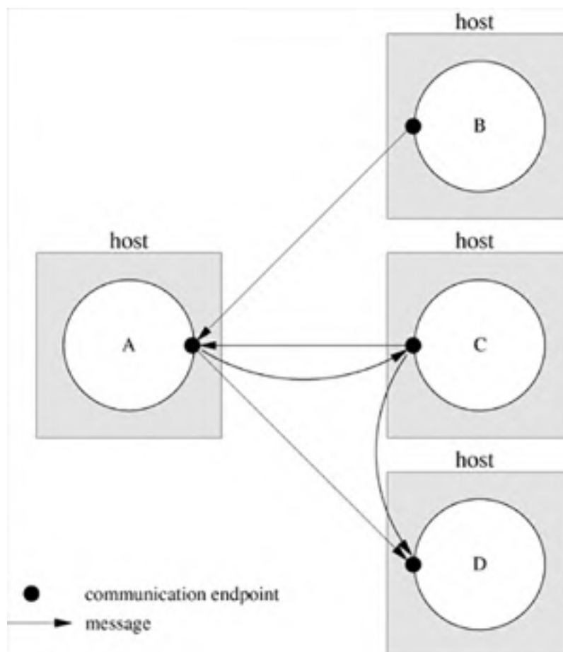
Figure 20.1. Four processes with connectionless communication endpoints.
