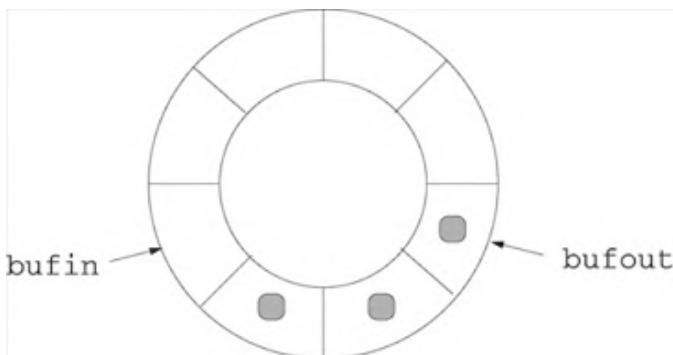
Figure 16.2. Circular buffer.
