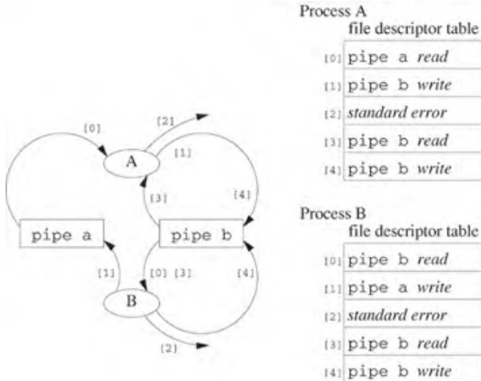
Figure 7.8. Connections of the processes of Example 7.5 after the entire code segment executes. Process A is the parent and process B is the child.
