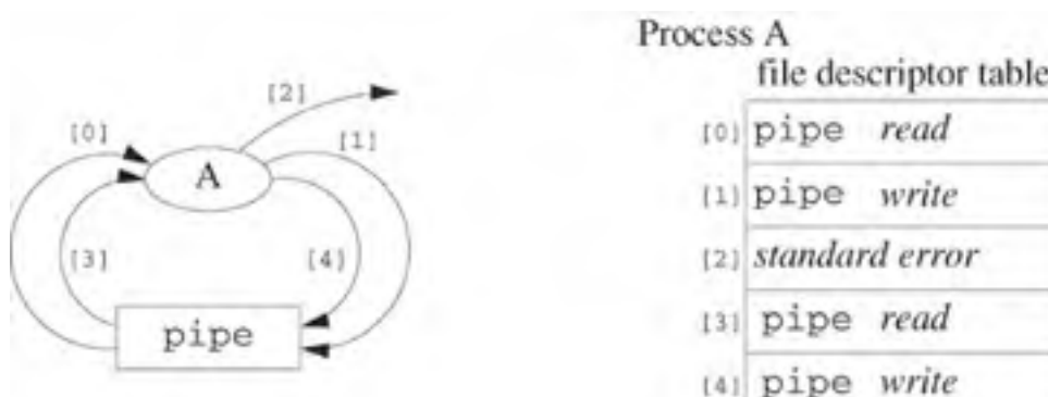
Figure 7.3. Status of the process of Example 7.1 after both dup2 functions execute.
