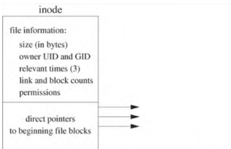
Figure 5.3. Schematic structure of a traditional UNIX file.
