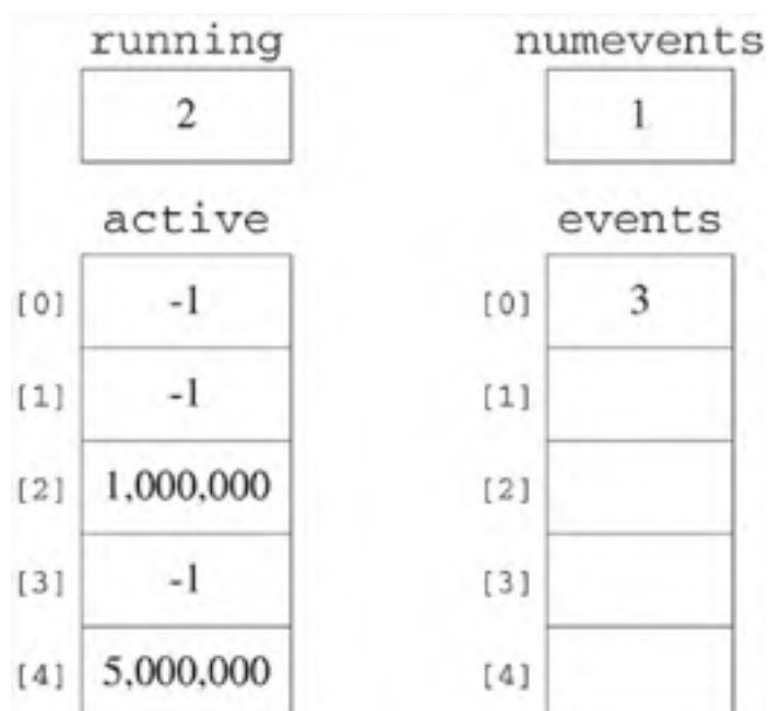
Figure 10.8 shows the situation two seconds later. Timer [2] expires and timer [4] becomes the running timer.
