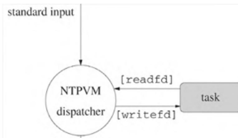
Figure 17.4. NTPVM dispatcher communicates with its children through pipes.
