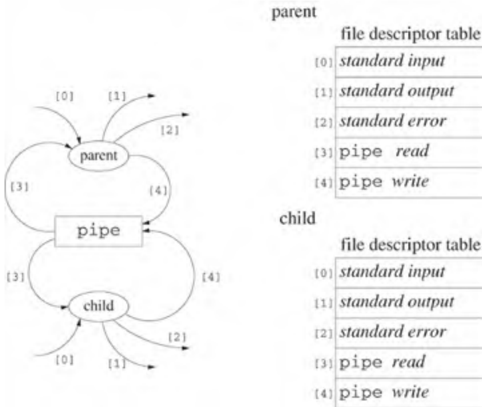
Figure 6.3. Status of the file descriptor table after both dup2 functions of Program 6.3.
