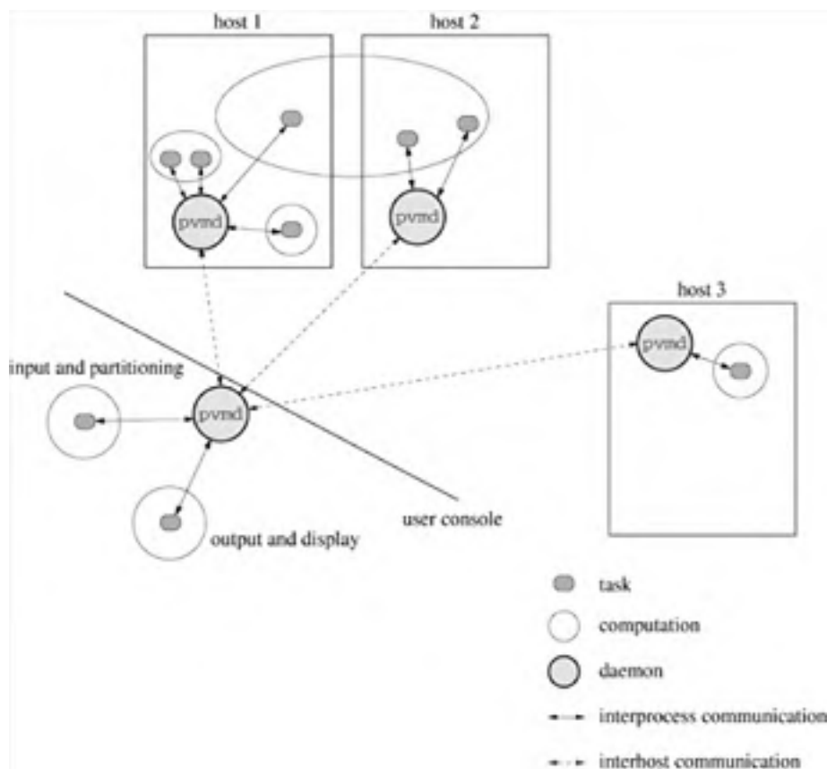
Figure 17.2. Schematic of a PVM.
