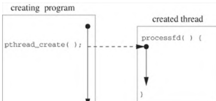
Figure 12.2. Program that creates a new thread to execute processfd has two threads of execution.
