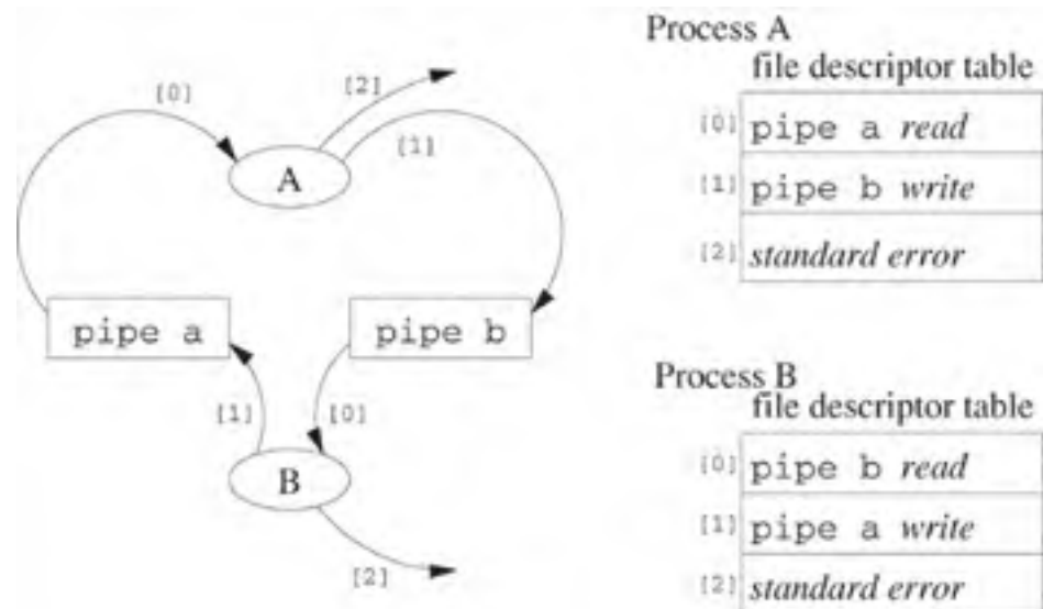
Figure 7.8. Connections of the processes of Example 7.5 after the entire code segment executes. Process A is the parent and process B is the child.
