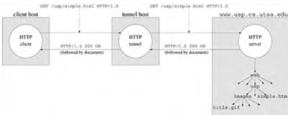
Figure 19.4. Communication between a user agent and an origin server through a tunnel.
