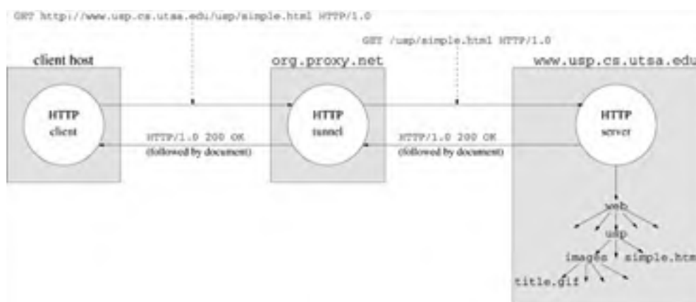
Figure 19.6. A proxy accesses any server on behalf of a client.
