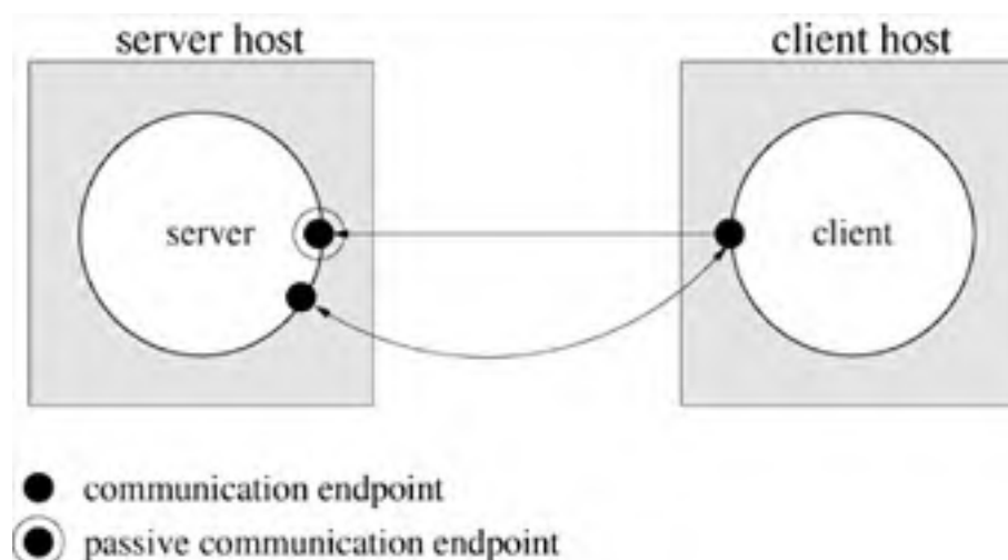
Figure 18.2. Schematic of connection-oriented client-server communication.
