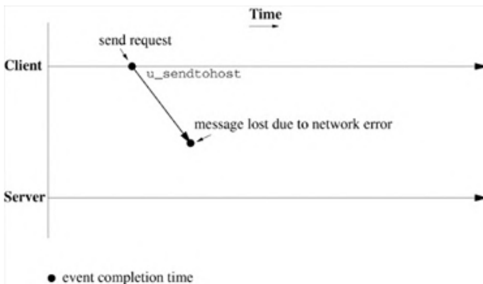
Figure 20.4. Time line illustrating a lost request for the simple-request protocol.
