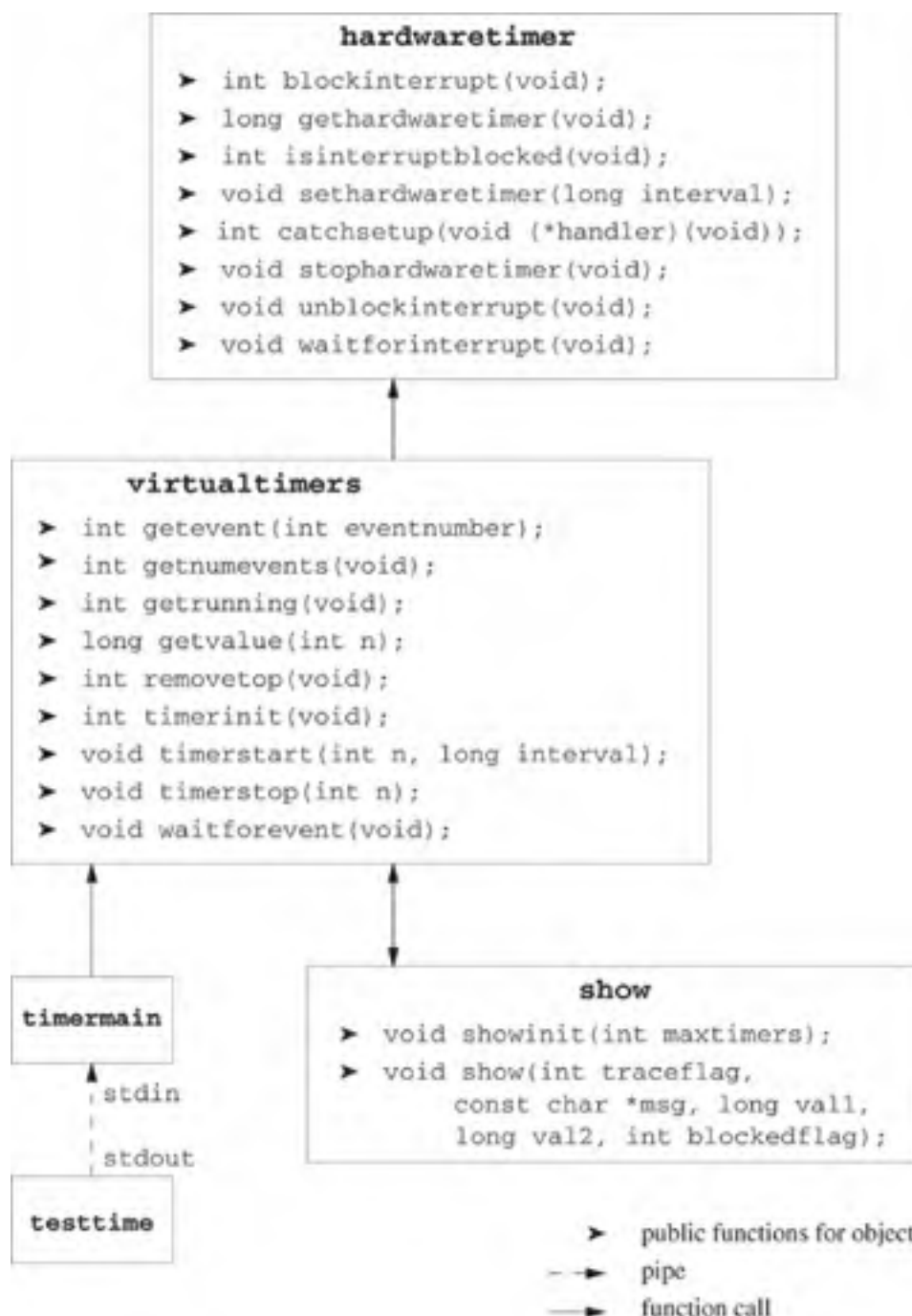
Figure 10.1. The five timer modules to be created in this project.
