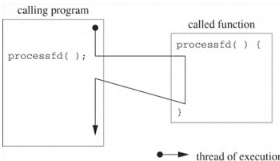
Figure 12.1. Program that makes an ordinary call to processfd has a single thread of execution.
