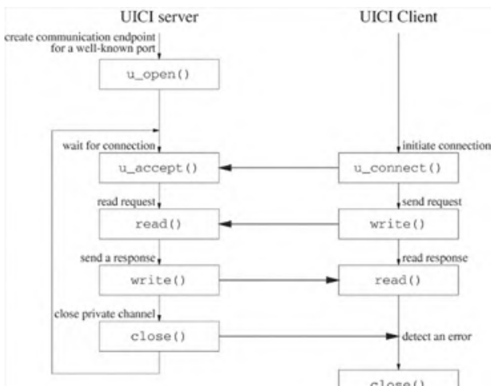
Figure 18.6. A typical interaction of a UICI client and server.
