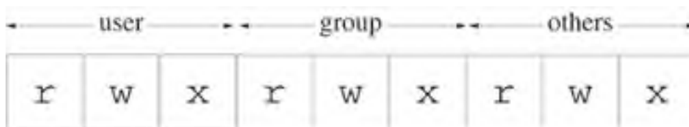
Figure 4.1. Historical layout of the permissions mask.
