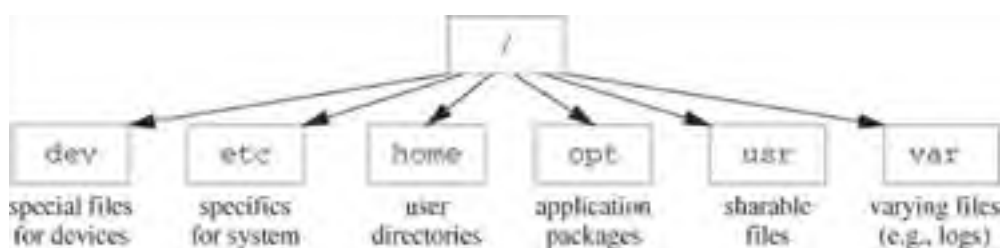
Figure 5.2. Structure of a typical UNIX file system
