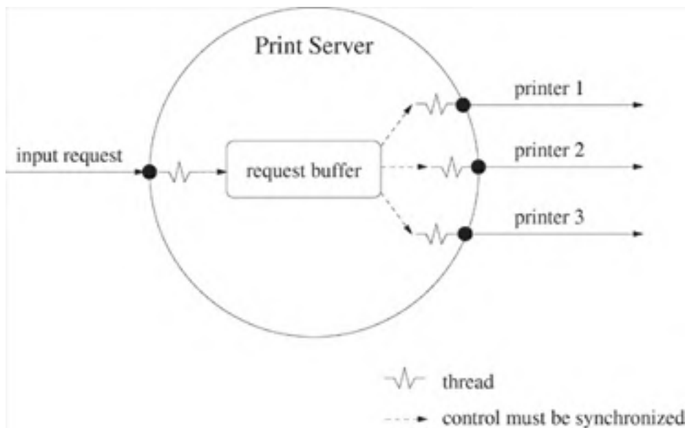
Figure 16.3. Schematic of a threaded print server.
