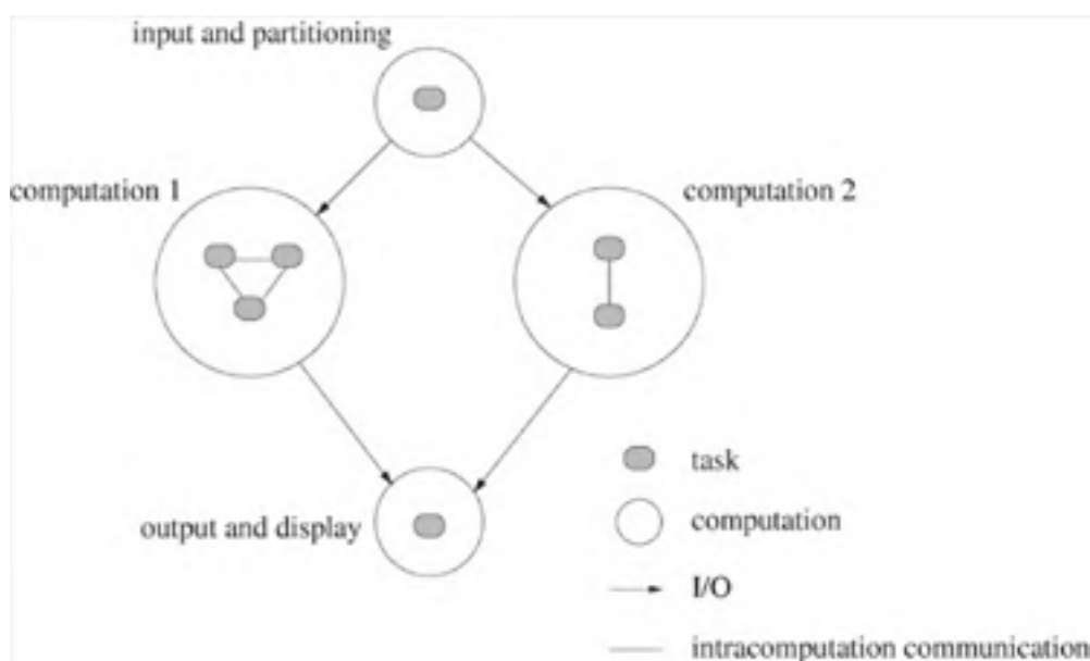
Figure 17.1. Logical view of an application running on a PVM virtual machine.
