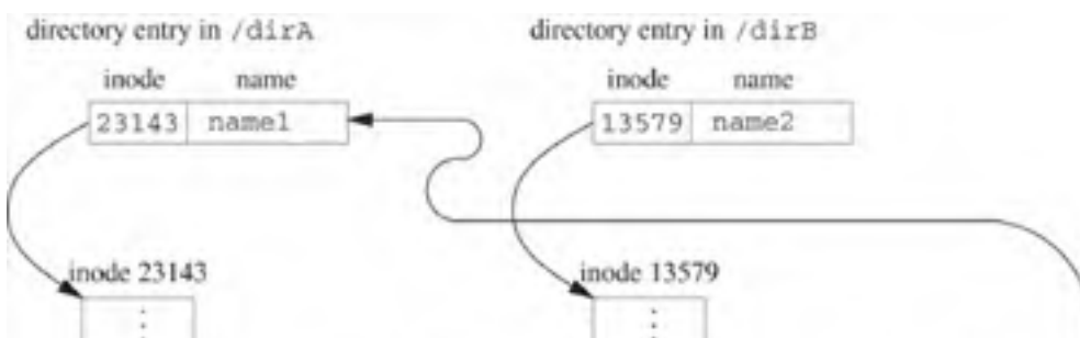
Figure 5.9. Situation after editing a file that has a symbolic link.
