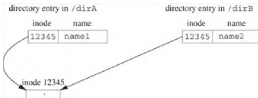
Figure 5.5. Two hard links to the same file shown in Figure 5.4 .
