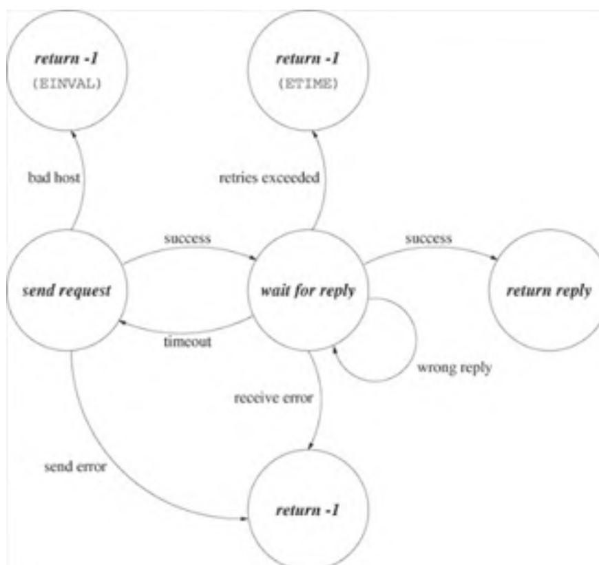
Figure 20.8. Request-reply with timeouts.
