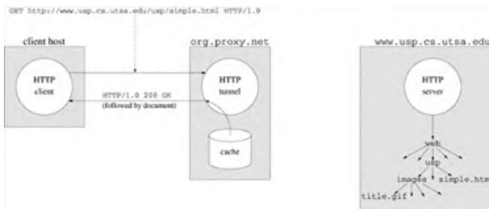
Figure 19.7. If possible, a proxy cache retrieves requested resources from its local store.
