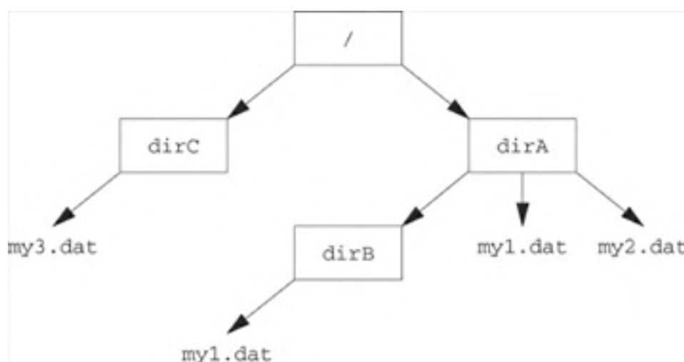
Figure 5.1. Tree structure of a file system.
