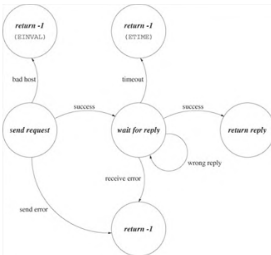
Figure 20.7. State diagram of the client for request-reply with simple timeout.
