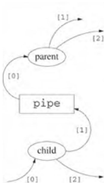
Figure 6.4. Status of the file descriptor table after all close calls of Program 6.3 .
