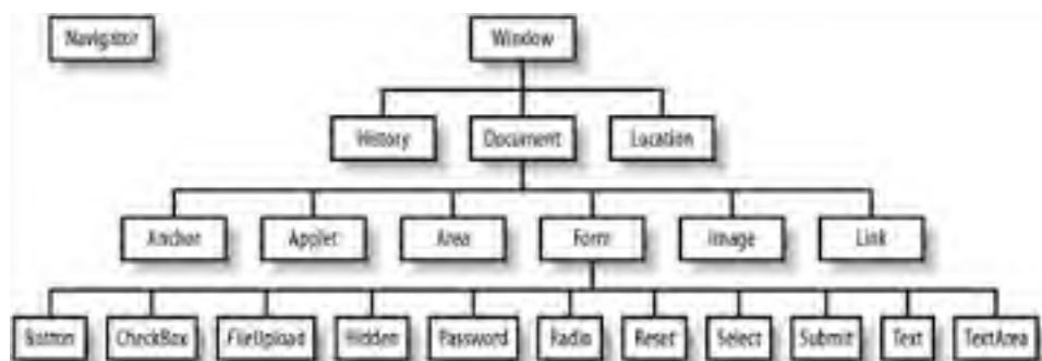
Figure 9-2. The hierarchy of window objects in the DOM
