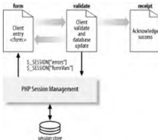
Figure 10-4. Phonebook entry form and validation
