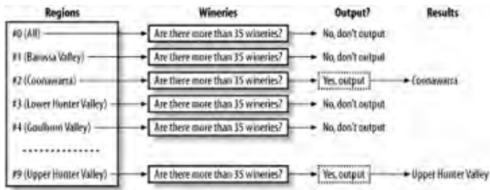
Figure 15-1. Evaluating a nested query that uses EXISTS
