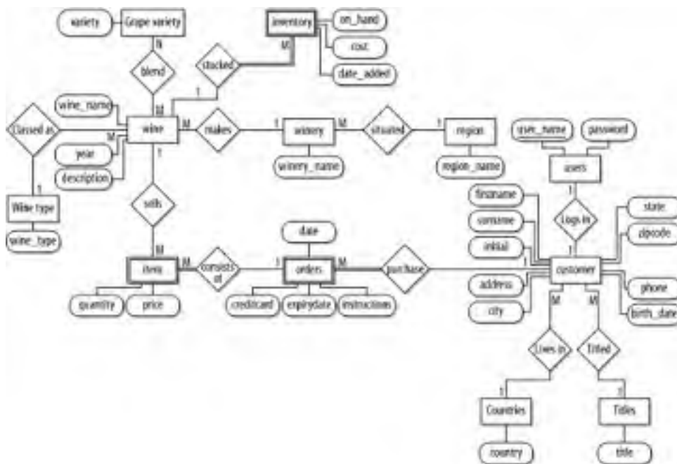
Figure E-4. An almost-complete ER model for the winestore
