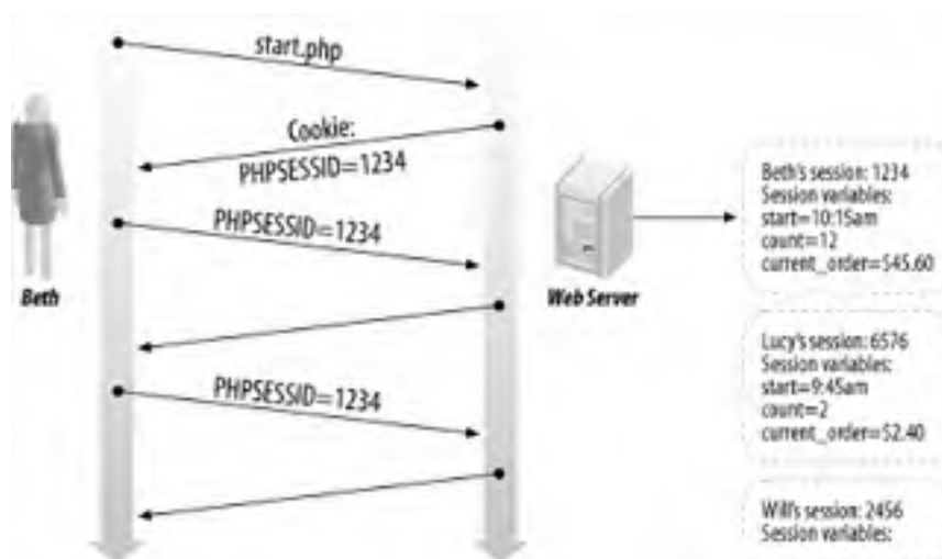
Figure 10-1. Session IDs and session variables
