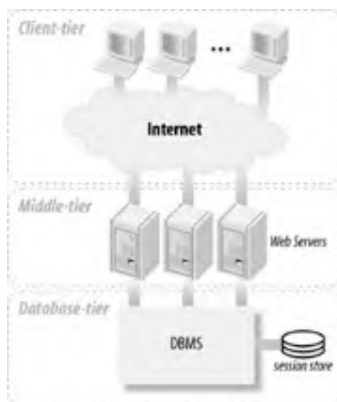
Figure F-1. Three-tier architecture using a database to store session variables
