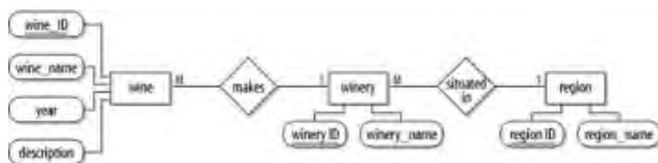
Figure E-2. A simple ER model showing the relationship between wines, wineries, and regions
