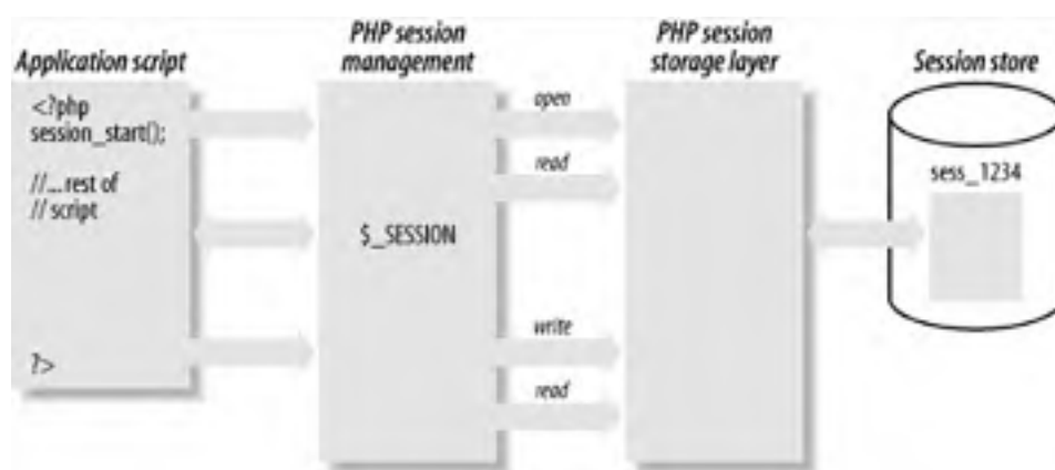
Figure F-2. PHP session management
