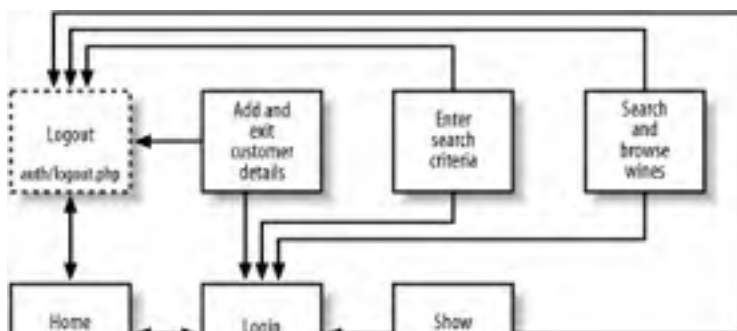
Figure 16-2. More winestore application architecture
