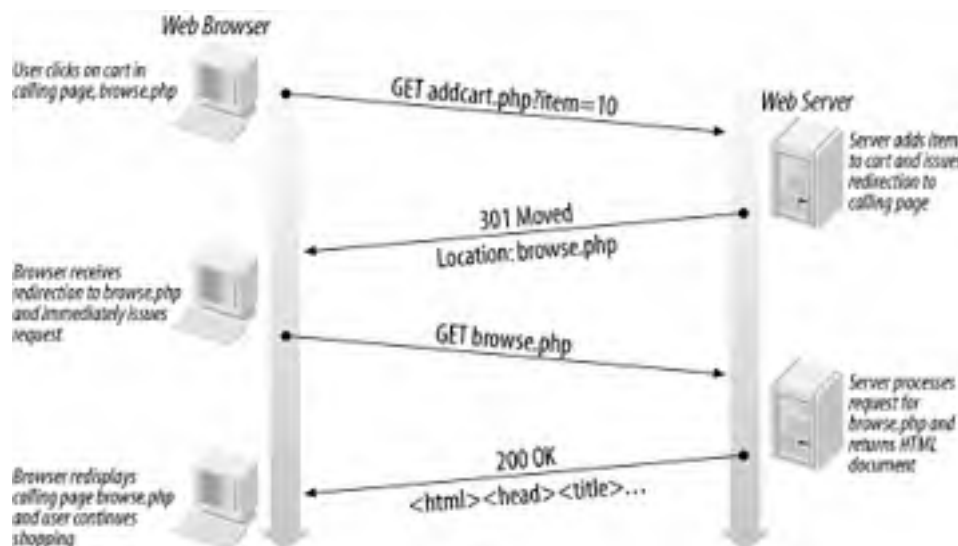
Figure 6-7. The principle of one-component querying
