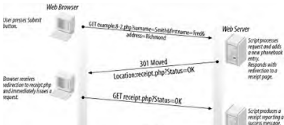
Figure 8-2. Solving the reload problem with a redirection to a receipt page
