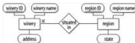
Figure 5-2. An example relational model of the winery database
