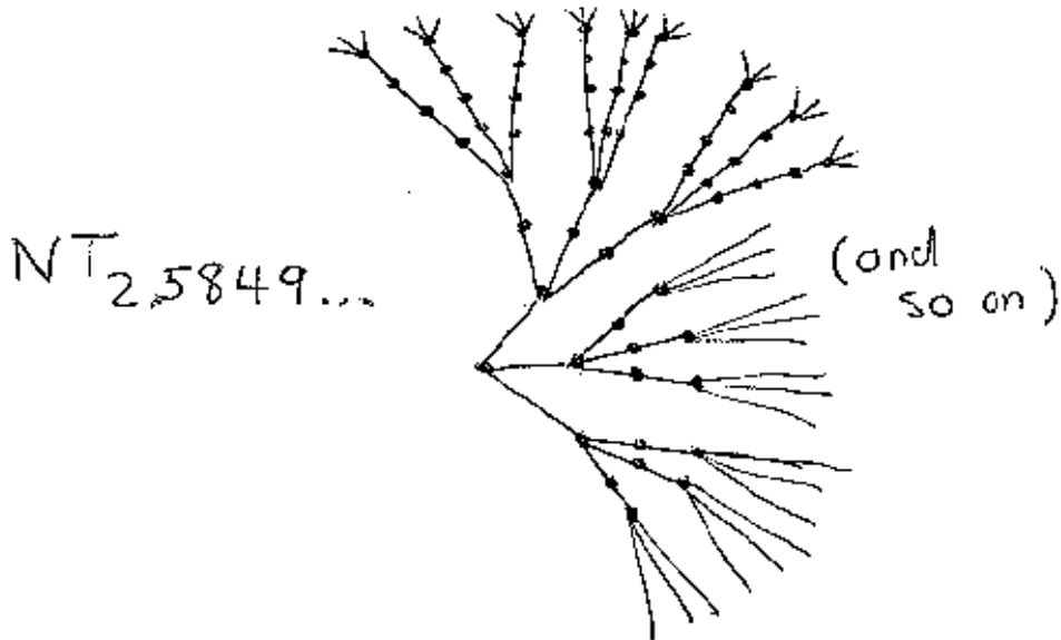
Figure 25: NT_{2.5849\dots} : A 2.5849...-dimensional tree.
