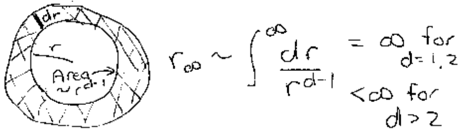
Figure 4: Can a physicist’s scribblings prove Polya’s theorem?
