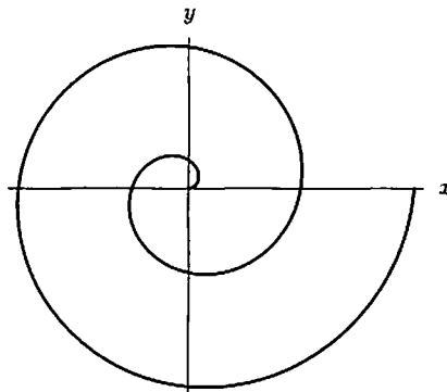
Figure 3.13: The spiral x = t \cos t, y = t \sin t for 0 \leq t \leq 4\pi
