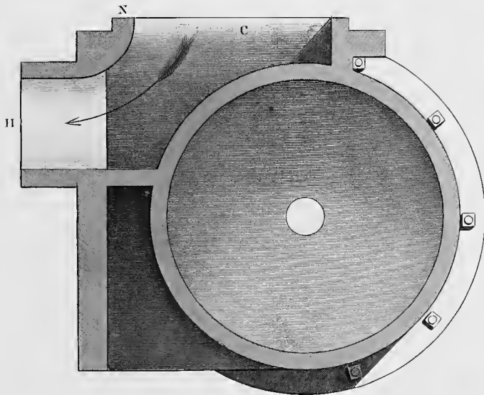
Fig. 4. Section through G.H. Fig. 1. Plate 36
