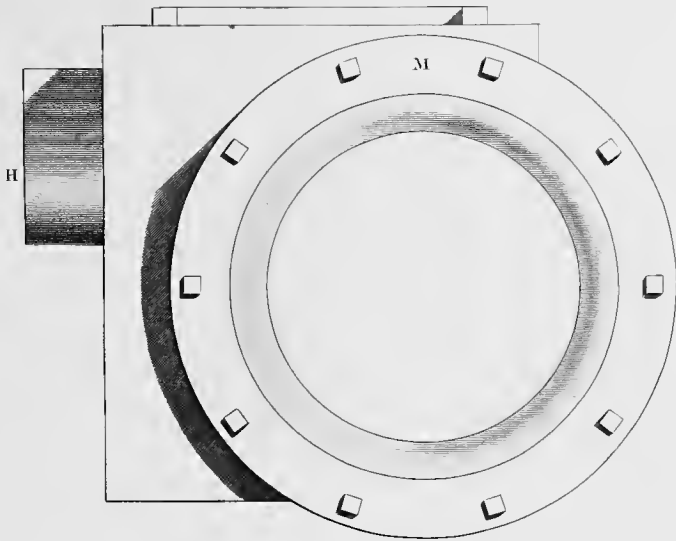
Fig. 3. End view
