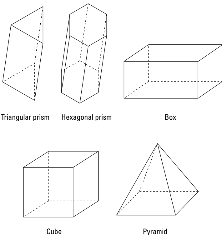
Figure 11-1: Common polyhedrons.
