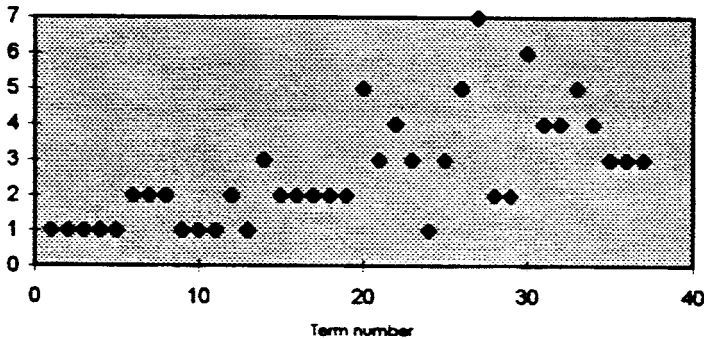
Diagram 4. The number of prime factors in the first 40 terms of the square-factorial sequence.
