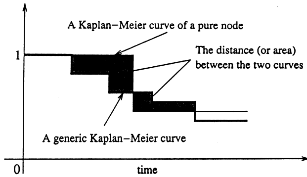
Fig. 142 Wasserstein metrics.
