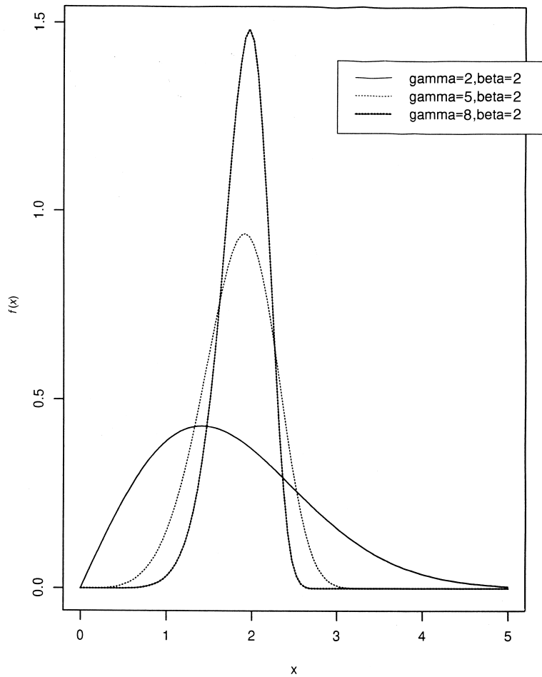
Fig. 145 Examples of Weibull distributions for several values of \gamma at \beta = 2 .
