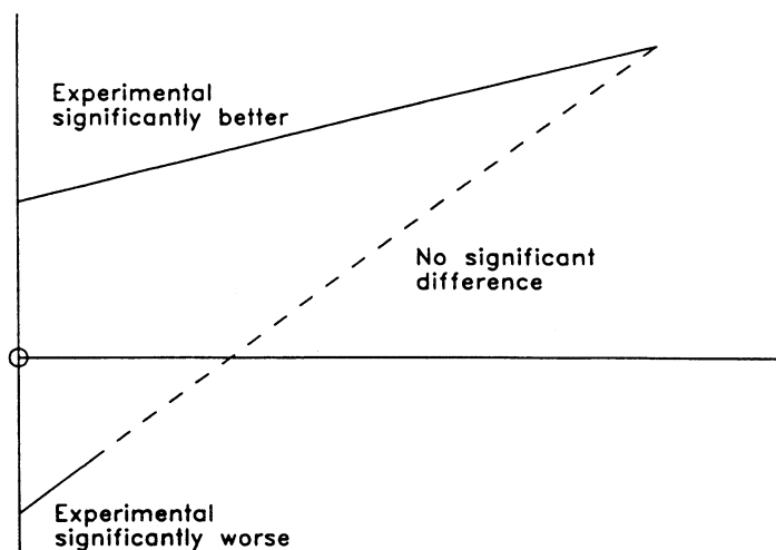
Fig. 135 The triangular region of a triangular test.
