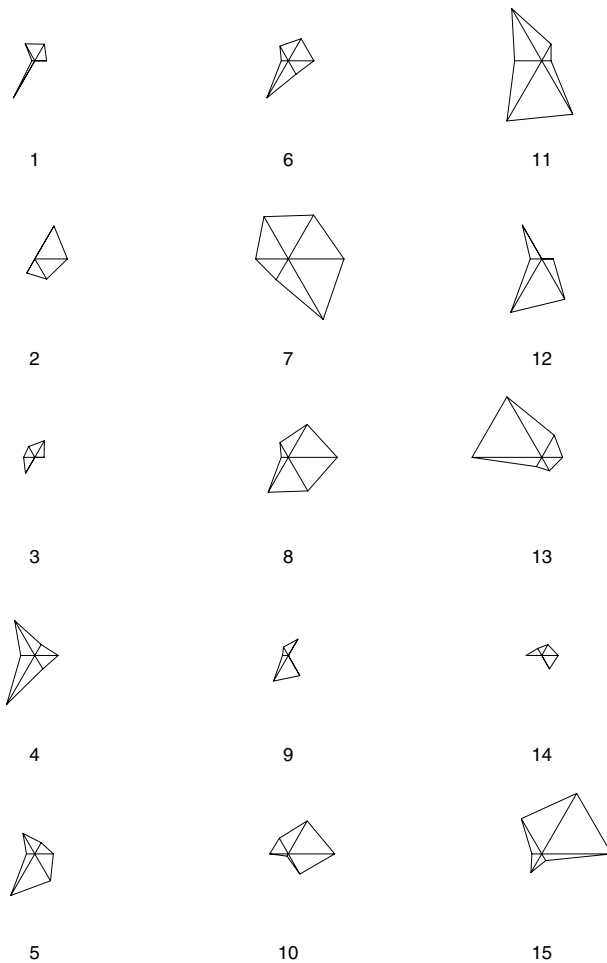
Fig. 125 A set of snowflakes for fifteen, six-dimensional multivariate observations.
