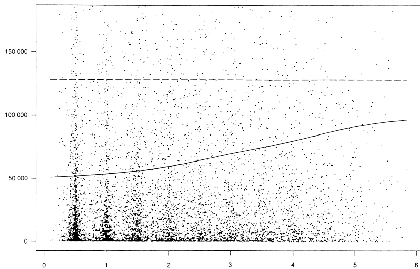
Fig. 138 Variogram plots.
