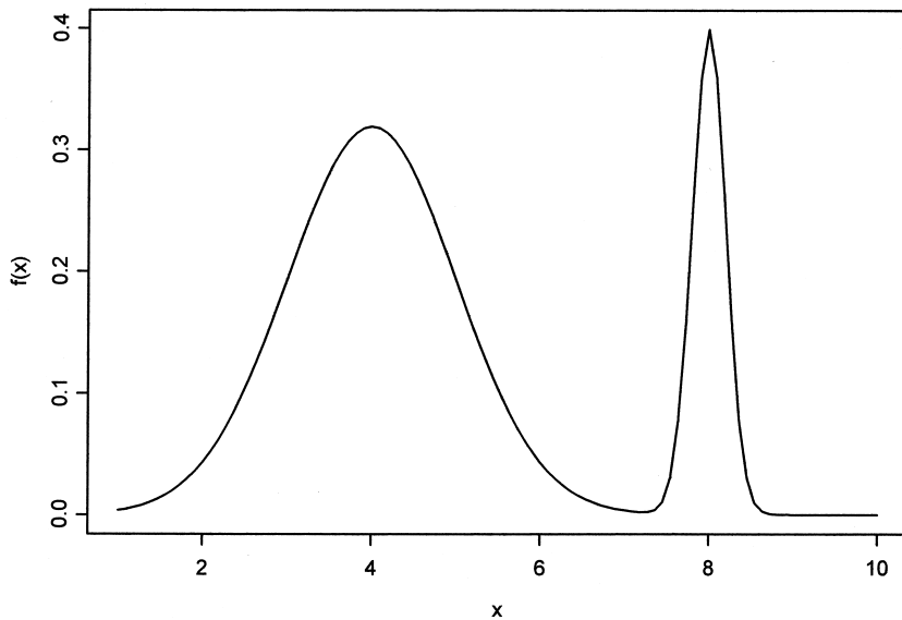
Fig. 64 Finite mixture distribution with two normal components.
