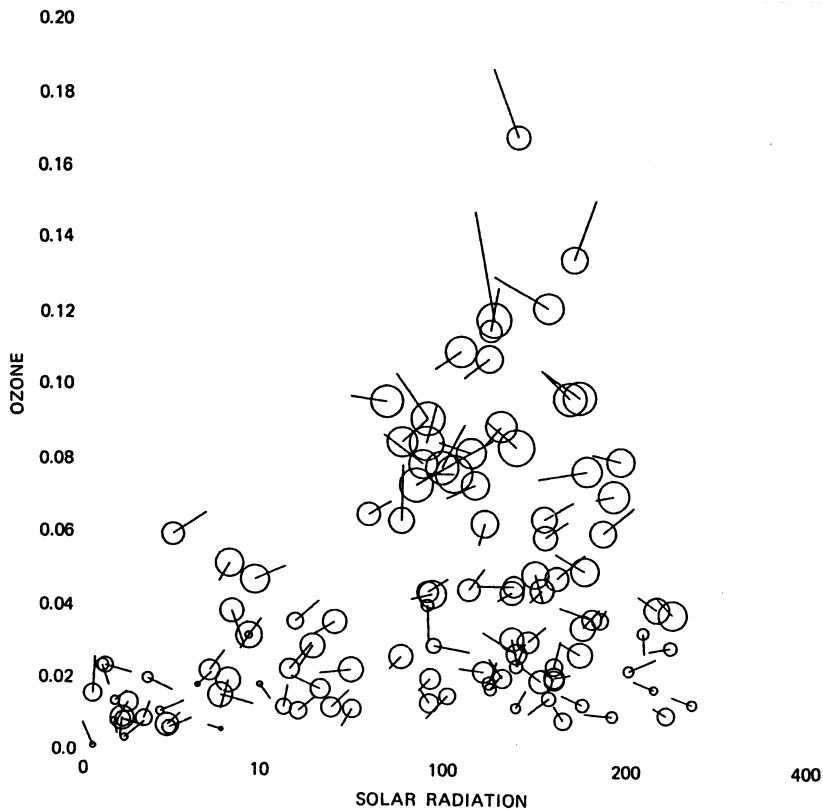
Fig. 144 Weathervane plot.
