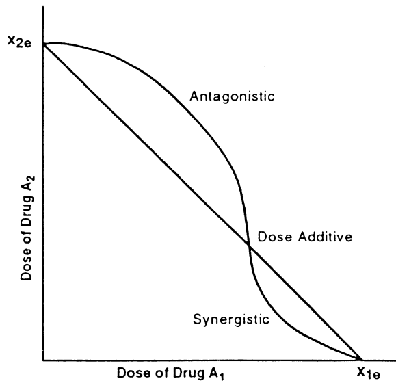
Fig. 76 An example of an isobologram.
