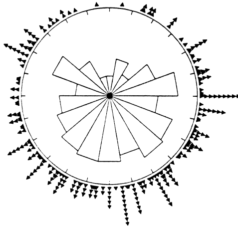
Fig. 115 Rose diagram for arrival times at an intensive care unit. (Reproduced from Statistical Analysis of Circular Data by permission of the publishers, Wiley.)
