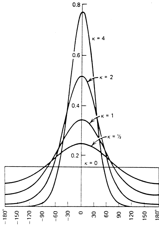
Fig. 141 Some examples of Von Mises distributions for \mu_0 = 0 and several values for \kappa .
