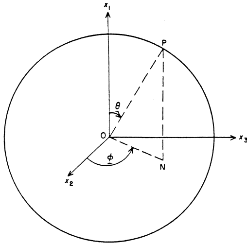
Fig. 126 An illustration of a spherical variable.
