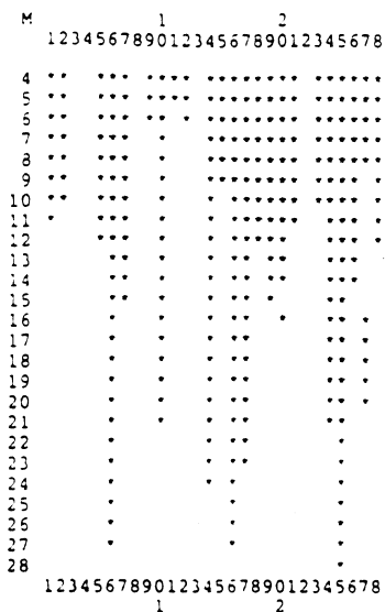
Fig. 127 An example of a stalactite plot.
