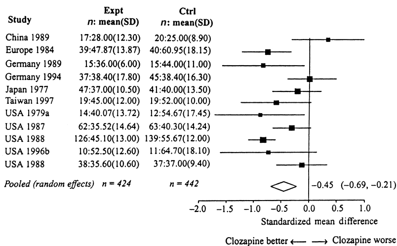
Fig. 65 Forest plot.
