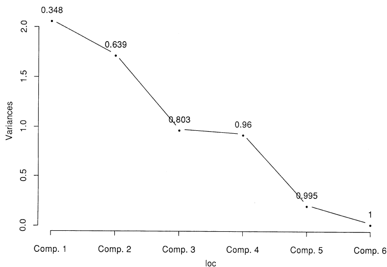
Fig. 118 Scree plot showing an 'elbow' at eigenvalue three.
