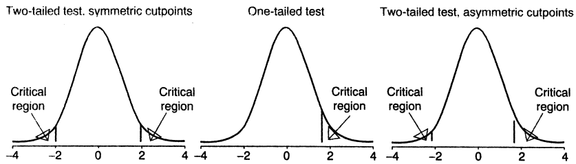
Fig. 48 Critical region.
