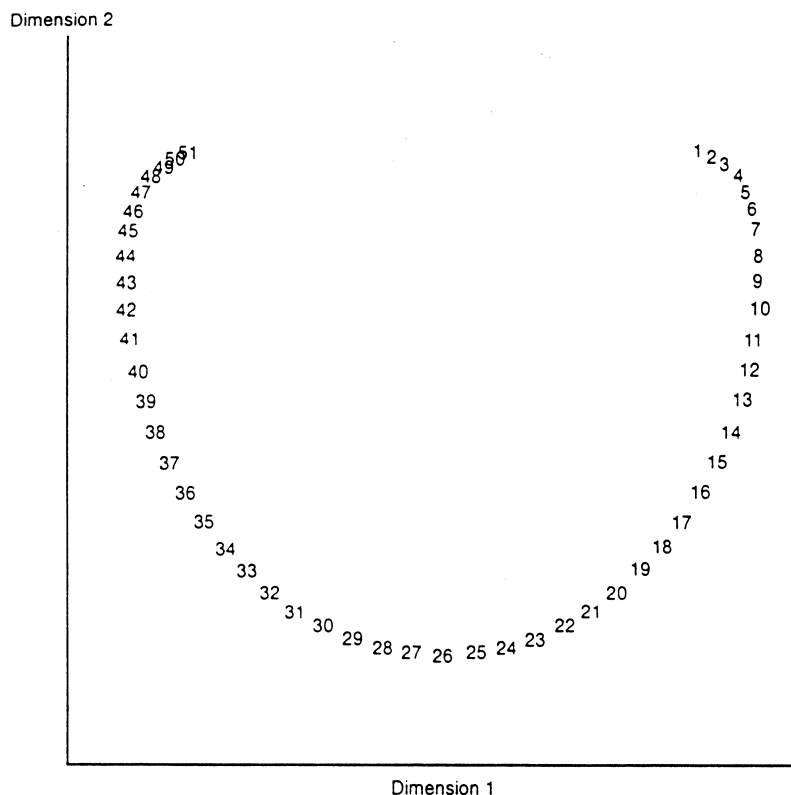
Fig. 119 Horseshoe effect.
