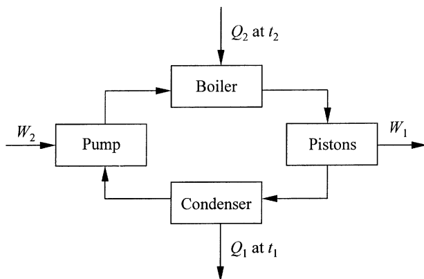
Figure 3.1. Diagram of the Woolf steam engine.
