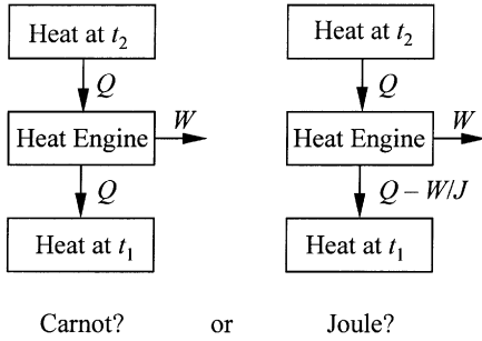
Figure 7.1. Heat engine operation between a high temperature t_2 and a low temperature t_1 , as viewed by Thomson in the conflicting theories of Carnot and Joule. Q represents heat, W work, J Joule's mechanical equivalent of heat, and \frac{W}{J} the heat equivalent to W . In the Carnot scheme, no heat is lost. In Joule's picture, an amount of heat \frac{W}{J} is lost.
