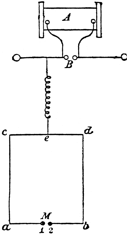
Figure 12.5. Hertz's coil circuit connected to a wire loop with a spark gap.
