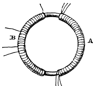
Figure 11.2. Faraday's first electromagnetic induction experiment. From Henry Bence Jones, The Life and Letters of Faraday (London: Longmans, Green, 1870), 2:2.
