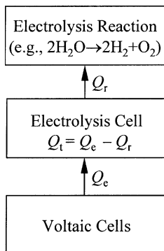
Figure 5.1. Input to and output from an electrolysis cell, according to Joule. The measured free heat Q_t in the cell depends only on the input Q_e from the voltaic cell and the output Q_r to the electrolysis reaction. It is equal to the input Q_e minus the output Q_r , that is, Q_t = Q_e - Q_r .
