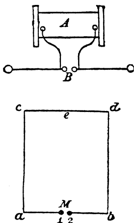
Figure 12.6. Hertz's coil circuit and wire loop disconnected. Sparks are still produced at the gap in the loop.
