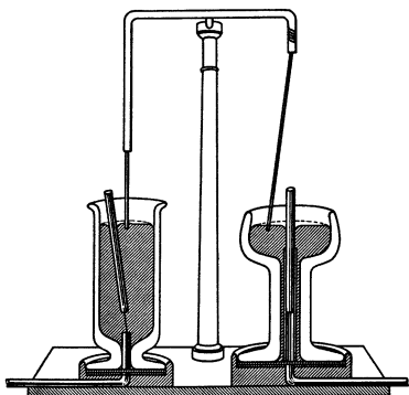
Figure 11.1. Faraday's experiments demonstrating electromagnetic rotation. From plate IV of Michael Faraday, Experimental Researches in Electricity (London: Taylor and Francis, 1839), vol. 2.
