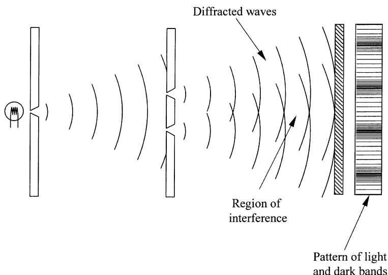
Figure 19.2. Diffraction and interference in the two-slit experiment.
