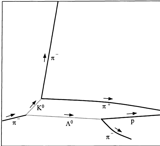
Figure 26.2. Interpretation of fig. 26.1. Only the relevant tracks are shown.
