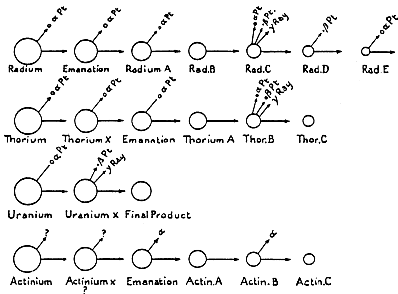
Figure 21.1. The radium, thorium, uranium, and actinium series of radioactive disintegrations, as displayed by Rutherford in his 1904 Bakerian lecture.
