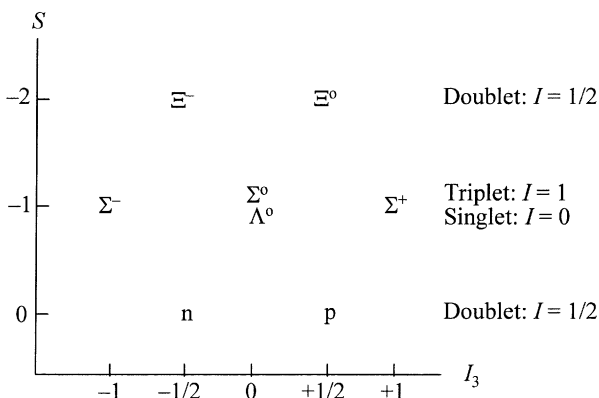
Figure 26.3. An octet of baryons plotted according to their isospin I_3 and strangeness S . Each symbol represents a point on the plot. For example, “ n ” locates a point at I_3 = -\frac{1}{2} and S = 0 .
