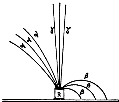
Figure 21.2. Rutherford's sketch of the three kinds of emissions from radium.
