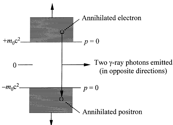
Figure 24.3. Annihilation of a positron and an electron resulting in formation of \gamma -rays.
