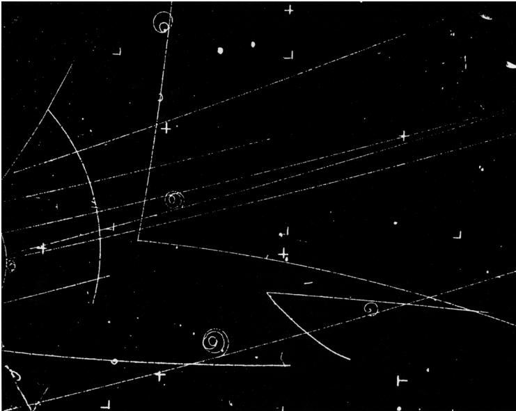
Figure 26.1. Photograph of tracks induced in a hydrogen-filled bubble chamber by a beam of high-energy, negatively charged pions. This photograph is reproduced by permission from the Lawrence Berkeley National Laboratory.
