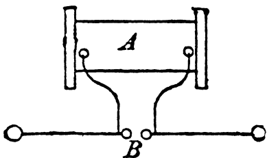
Figure 12.4. Hertz's coil circuit. This figure and the two following are adapted from Heinrich Hertz, "On Very Fast Electric Oscillations," in Wiedemann's Annalen der Physik und Chemie 31 (1887): 431.
