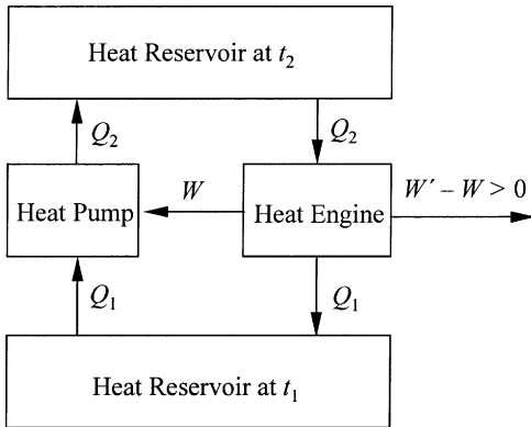
Figure 3.2. Illustration of impossible perpetual work output obtained by linking two ideal heat engines with different work outputs, W and W' .
