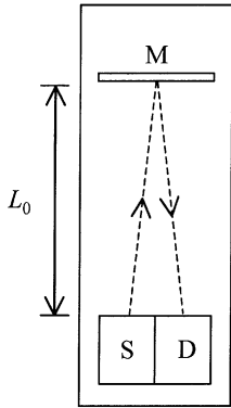
Figure 14.1. Einstein's light clock, as seen by an observer traveling with the clock. The distance between the source and the detector is exaggerated. This figure, the one that follows, and fig. 14.4 are adapted with permission from Robert Resnick, David Halliday, and Kenneth Krane, Physics , 4th ed. (New York: Wiley, 1992), 470.
