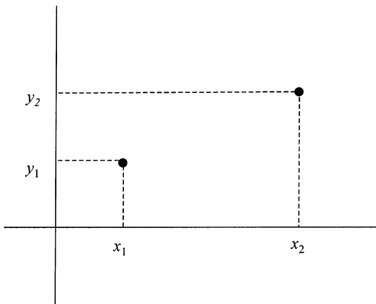
Figure 14.5. Location of two events in two spatial dimensions at the two points x_1, y_1 and x_2, y_2 .
