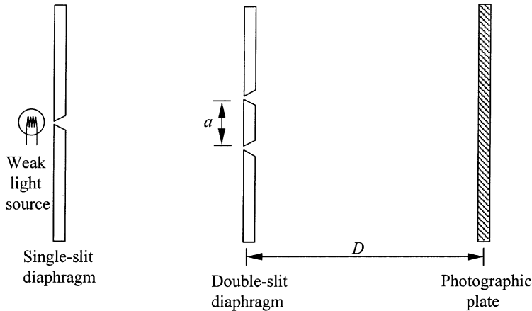
Figure 19.1. The two-slit experiment.
