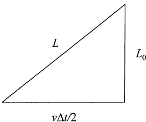
Figure 14.3. A right triangle constructed from the distances shown in fig. 14.2, demonstrating that according to the Pythagorean theorem L^2 = L_0^2 + (v\Delta t / 2)^2 or L = \sqrt{L_0^2 + (v\Delta t / 2)^2} .
