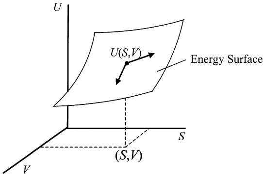
Figure 9.1. An energy surface containing points located by the entropy S , the volume V , and the internal energy regarded in the Gibbs manner, as a function U(S, V) of S and V .
