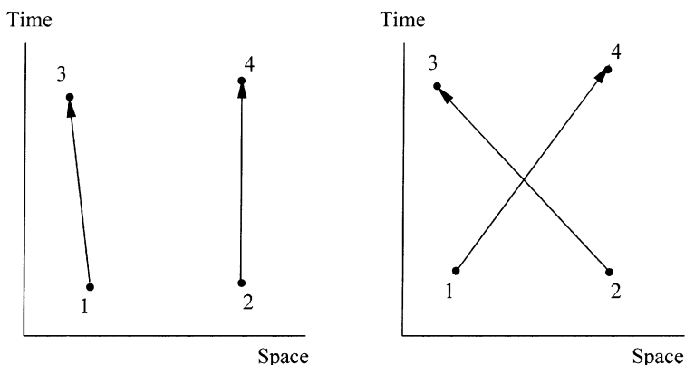
Figure 25.1. Feynman diagrams for two ways two electrons can get from points 1 and 2 in space and time to points 3 and 4.
