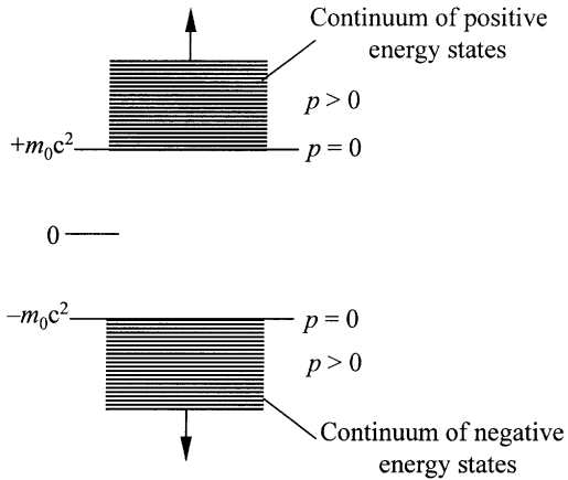
Figure 24.1. Positive and negative energy states according to the relativistic energy equation (5).
