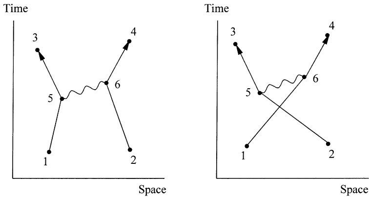
Figure 25.2. Feynman diagrams for two more ways two electrons can get from points 1 and 2 in space and time to points 3 and 4. These paths involve interaction between the electrons mediated by a photon.
