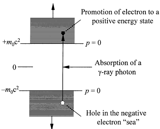
Figure 24.2. A negative-energy electron promoted to a positive-energy state by the absorption of a \gamma -ray photon.
