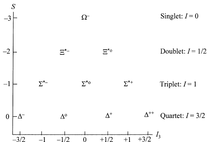
Figure 26.4. A decuplet of baryons plotted as in fig. 26.3.
