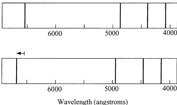
Figure 27.1. Wavelengths from the spectrum of light emitted by hydrogen. Above: as they appear normally. Below: the same wavelengths redshifted by about 2%, with z = 0.02 . An angstrom is a very small measure of length, equal to 10^{-8} centimeter. Adapted with permission from John Hawley and Katherine Holcomb, Foundations of Modern Cosmology (New York: Oxford University Press, 1998), 263.
