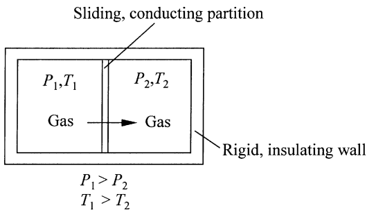
Figure 9.4. An isolated system on its way to equilibrium, driven by mechanical and thermal nonuniformities.
