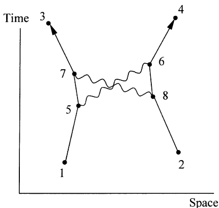
Figure 25.3. Feynman diagram for still another way two electrons can get from points 1 and 2 to points 3 and 4. Each electron emits and absorbs a photon.
