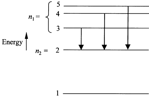
Figure 16.1. An energy-level diagram showing emission transitions for three of the lines in the hydrogen Balmer series.
