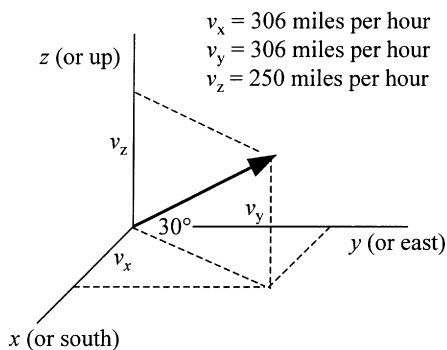
Figure 12.1. Picture of a velocity vector \mathbf{v} (represented by the arrow) for an airplane headed southeast at 500 miles per hour and climbing at an angle of 30^\circ .
