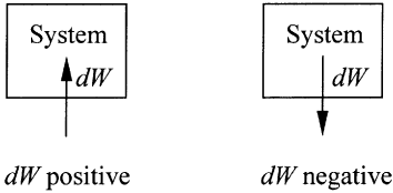
Figure 8.2. Illustration of the sign convention for dW .
