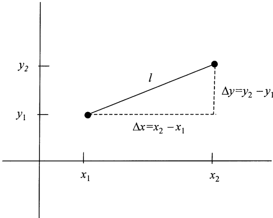
Figure 14.6. Calculation of the spatial interval l between the two events of fig. 14.5.
