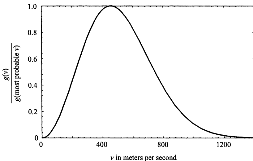
Figure 13.2. Maxwell’s distribution function g(v) . The plot is “normalized” by dividing each value of g(v) by the value obtained with v given its most probable value.
