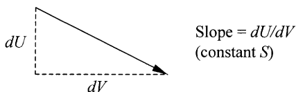
Figure 9.2. Side view of the left arrow extracted and enlarged from fig. 9.1. Like the ratio of rise to run for a staircase, the ratio of dU (rise) to dV (run), that is, the derivative \frac{dU}{dV} , calculates the slope of the arrow, and of the energy surface, at the point where the arrow is drawn.
