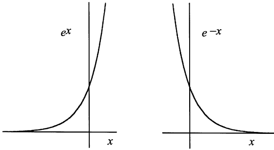
Figure 13.1. Typical exponential functions: the increasing e^x and the decreasing e^{-x} .
