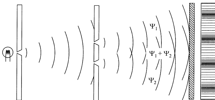
Figure 19.3. Wave functions for the two-slit experiment.
