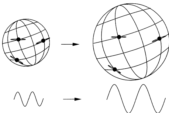
Figure 27.2. Above: an impression of an expanding universe as it might be seen in two-dimensional curved space. The two-dimensional expansion is like the inflating of a balloon with the galaxies pasted on its surface. Below: the corresponding increase in the wavelength of light. Adapted with permission from John Hawley and Katherine Holcombe, Foundations of Modern Cosmology (New York: Oxford University Press, 1998), 282.
