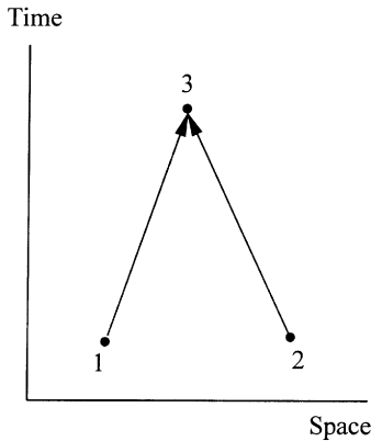
Figure 25.4. Feynman diagram for two electrons attempting to occupy the same point in space and time. The amplitude for this process is zero if the two electrons have the same spin state, nonzero if they have different spin states.
