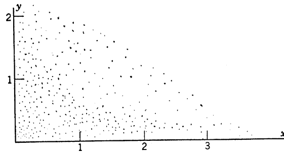
Fig. 1. Probability density distribution.
