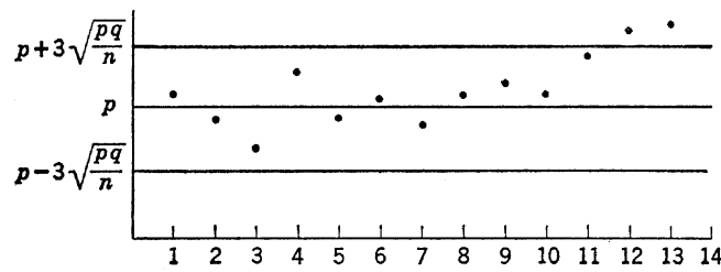
Fig. 10. Control chart for fraction defective.
