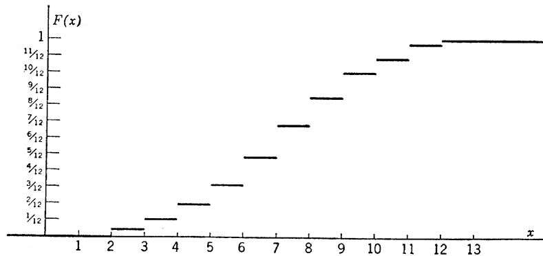
Fig. 4. Graph of a distribution function.
