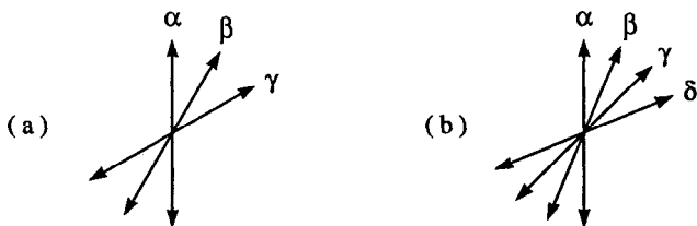
Fig. 6.7. Linear polarization directions giving the maximal violation of (a) Bell's inequality (6.26), and (b) the CHSH inequality (6.30).
