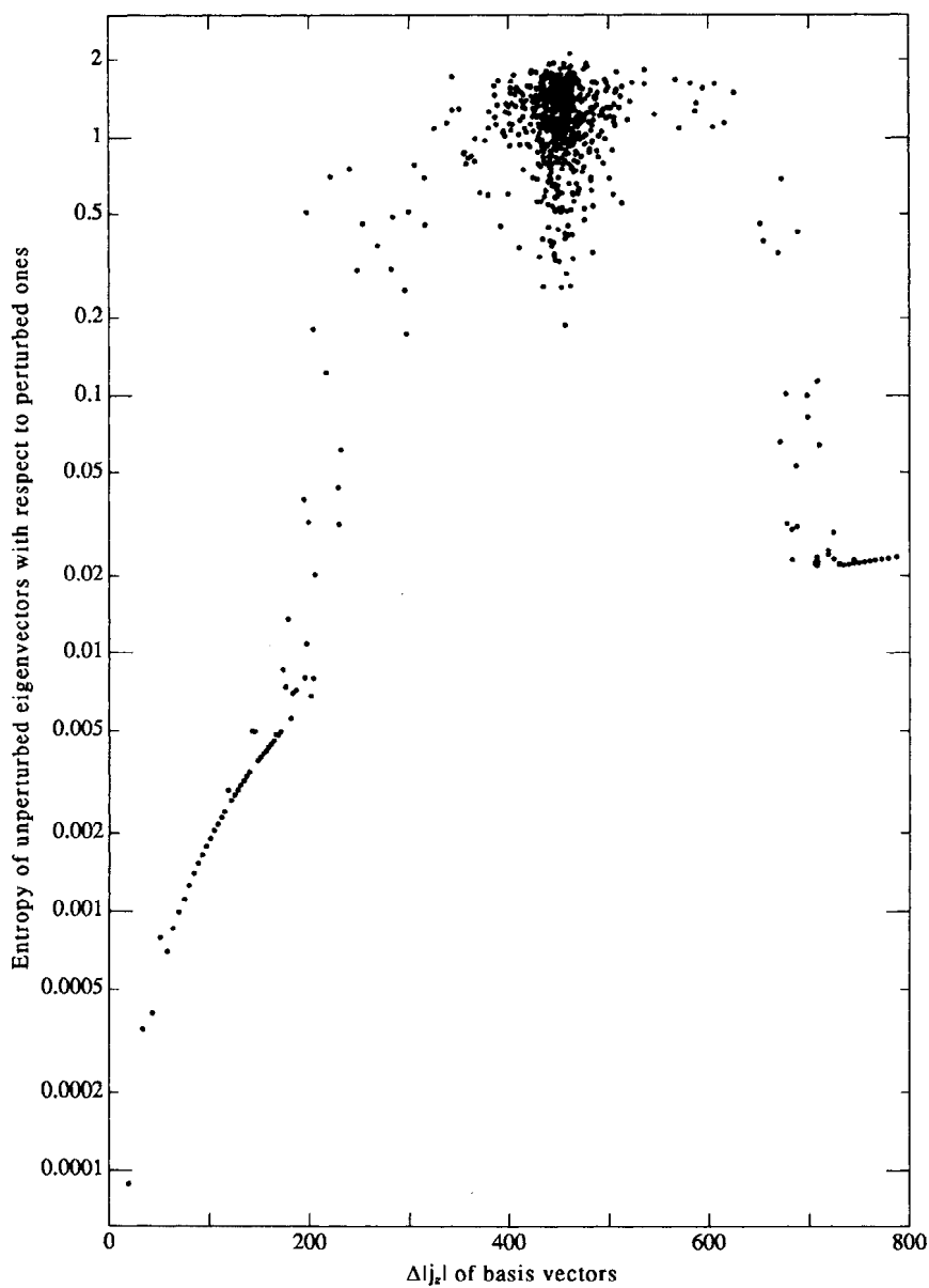
Fig. 11.10. Sensitivity of eigenvectors of U to a perturbation, versus their extent in |j_z\rangle space. The blob at the top contains extended and fragile states. The two strings contain robust states, localized near the classical fixed points.
