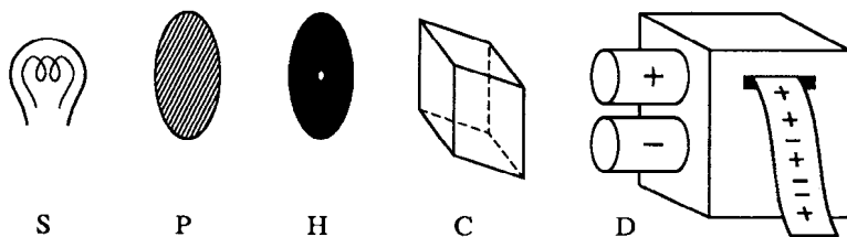
Fig. 1.3. Light from a thermal source S passes through a polarizer P , a pinhole H , a calcite crystal C , and then it triggers one of the detectors D . The latter register their output in a device which prints the results.
