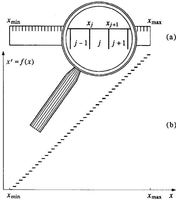
Fig. 4.3. (a) The magnifying glass shows the details of a ruler used to measure the continuous observable x . (b) The result of the measurement is given by the staircase function f(x) .
