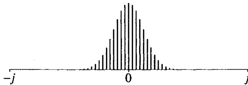
Fig. 12.6. Expected probability distribution for a measurement of J_z , after preparation of a state with j_z = j , and its rotation by \pi/2 . The calculations were done for j = 32 . The standard deviation is \Delta J_z = 4 .
