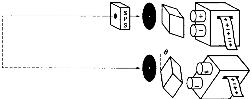
Fig. 6.3. If one of the detecting stations is tilted by an angle \theta , the correlation of the outcomes is \cos 2\theta .
