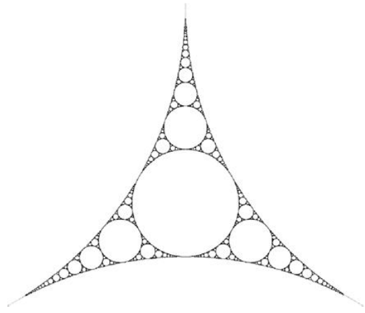
Apollonius problem The Apollonian gasket.
