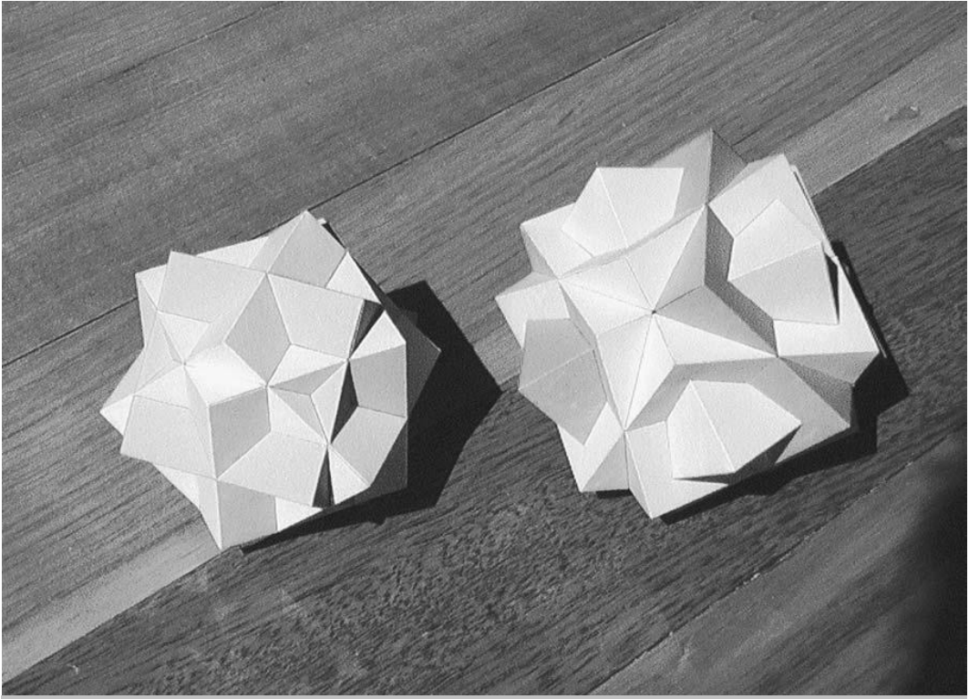
compound polyhedron A compound polyhedron of three cubes (left), such as that used in Escher's picture "Waterfall." The compound of four cubes (right) is also known as Bakos's compound. Robert Webb, www.software3d.com ; created using Webb's Stella program
