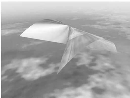
Whitney's umbrella Takashi Nishimura
