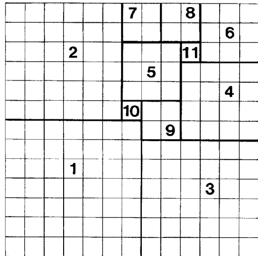
The solution of Mrs. Perkins’s quilt.
