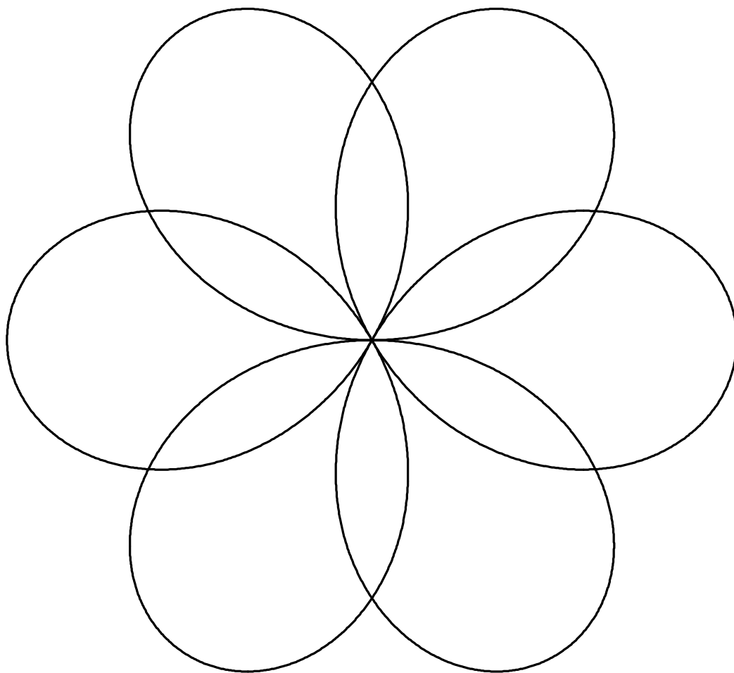
rose curve © Jan Wassenaar, www.2dcurves.com
