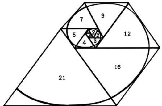
plastic number Spiraling systems illustrate the Fibonacci numbers (top) and the Padovan sequence.
