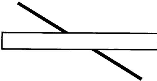
Poggendorff illusion
