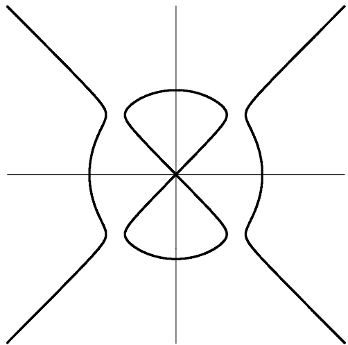
devil's curve © Jan Wassenaar, www.2dcurves.com
