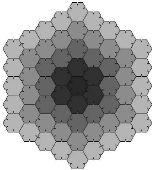
Heesch number A tiling in which copies of the same shape are used out to the fourth surrounding layer, or corona. David Eppstein
