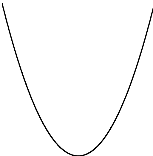
parabola Jan Wassenaar, www.2dcurves.com
