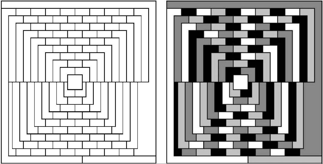
four-color map problem Martin Gardner's spoof counterexample to the four-color theorem (left) and a solution using four colors (right). The different colors are represented here in black, white, and gray.
