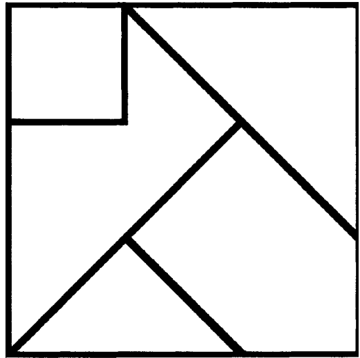
Pythagorean puzzle solution.
