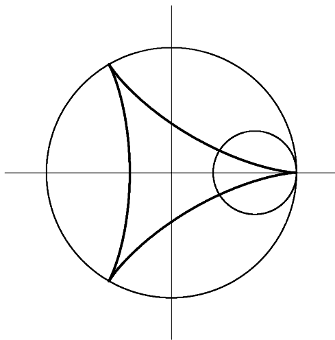
deltoid The deltoid curve. © Jan Wassenaar, www.2dcurves.com
