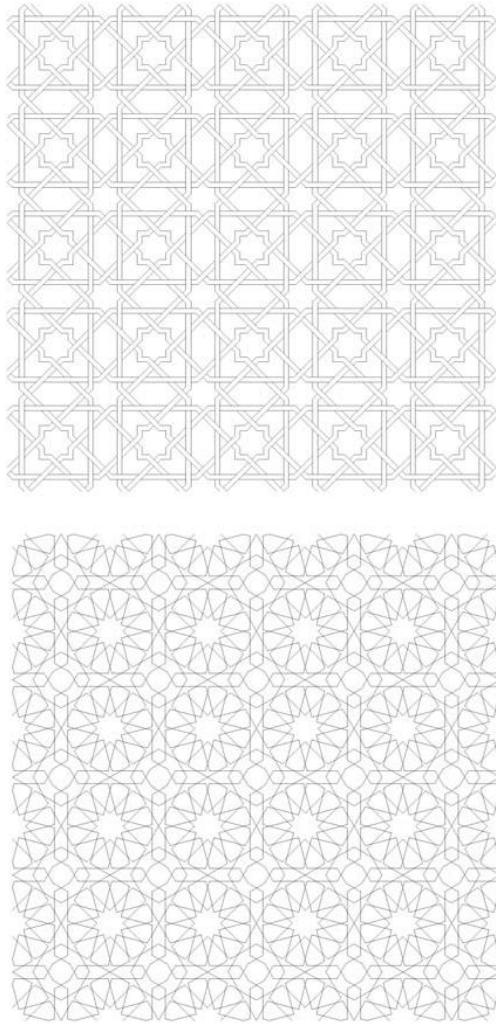
Alhambra Computer-generated tilings based on Islamic tile designs such as those found in the Alhambra. Xah Lee , www.xahlee.org
