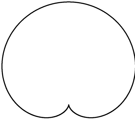
limaçon of Pascal © Jan Wassenaar, www.2dcurves.com
