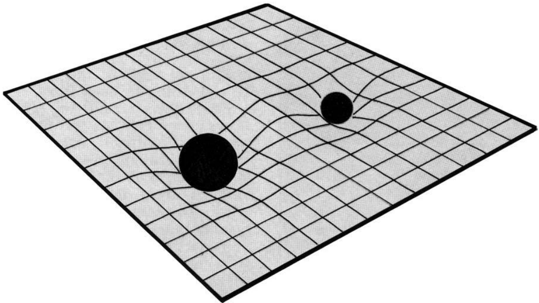
space-time Gravity seen as a curvature of the fabric of space and time.
