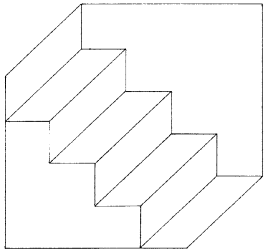
Schröder's reversible staircase
