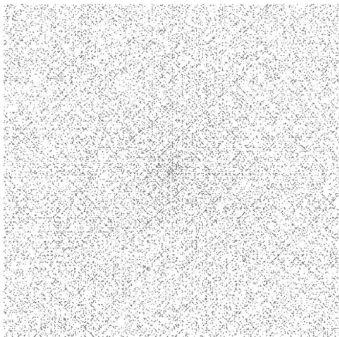
Ulam spiral Patterns amid the primes.
