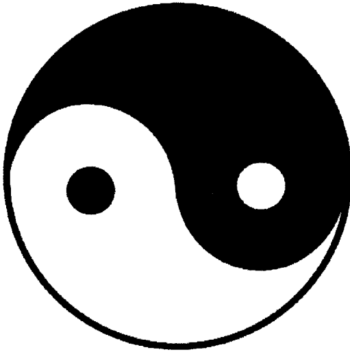
Great Monad
