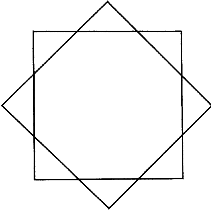
star of Lakshmi
