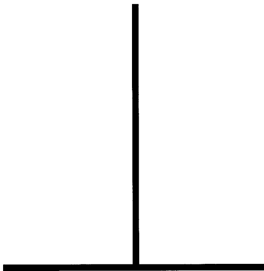
vertical-horizontal illusion
