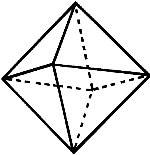
octahedron One of the Platonic solids.
