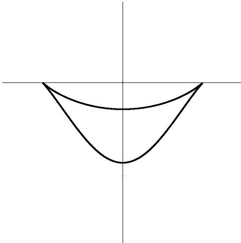
bicorn The bicorn curve © Jan Wassenaar, www.2dcurves.com
