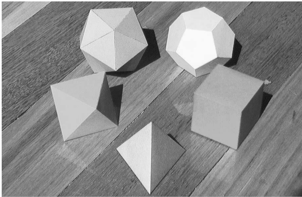
Platonic solid Clockwise from the extreme right: the cube, tetrahedron, octahedron, icosahedron, and dodecahedron. Robert Webb, www.software3d.com; created using Webb's Stella program
