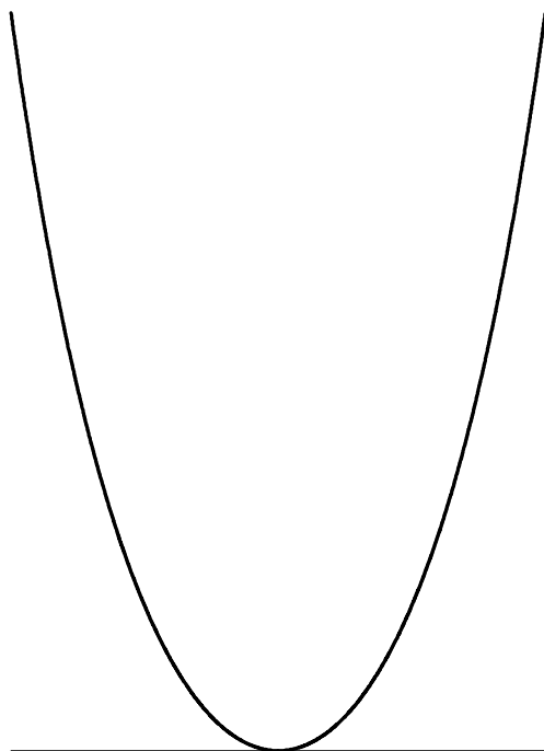
catenary The catenary curve. © Jan Wassenaar, www.2dcurves.com
