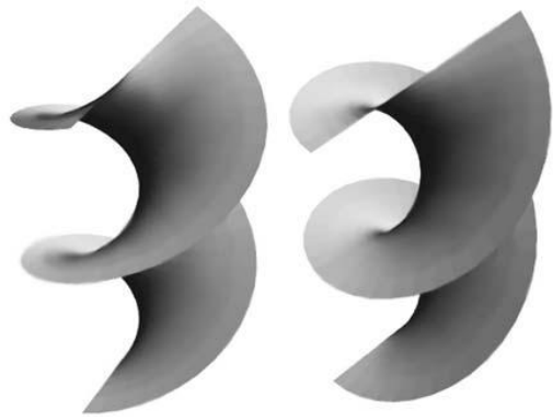
helicoid Richard Palais
