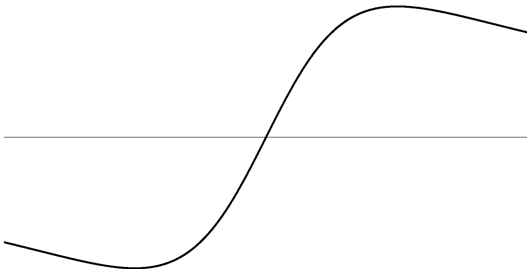
serpentine The serpentine curve. © Jan Wassenaar, www.2dcurves.com
