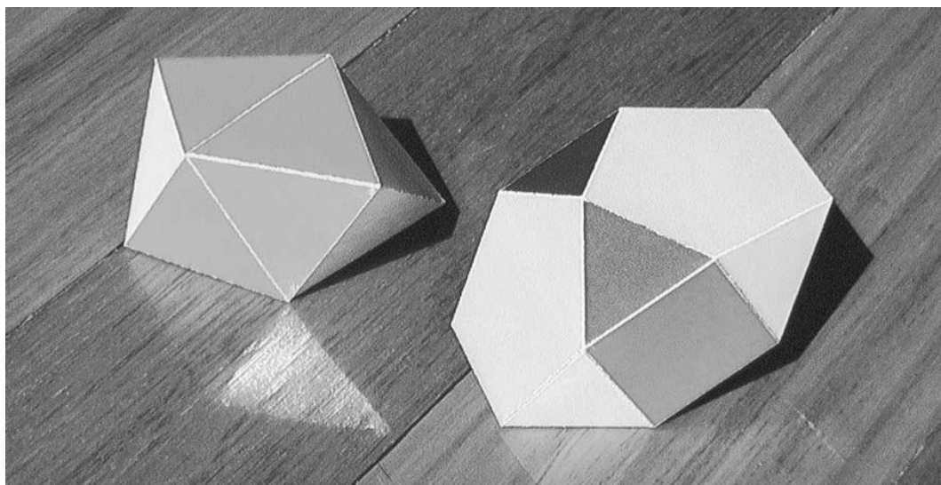
Johnson solid Two of the 92 Johnson solids: the bilunabirotunda (J91, right) and the snub disphenoid (J84, left). Robert Webb, www.software3d.com ; created using Webb's Stella program
