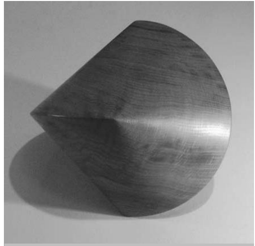
sphericon A model in oak of this remarkable shape. Paul and Colin Roberts
