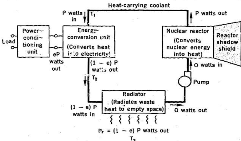
Figure 7 Schematic diagram of a generalized nuclear-reactor space power plant.
