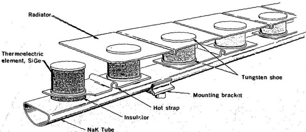
Figure 13 The SNAP-10A thermoelectric converter module. Heat brought in by hot NaK is partially converted to electricity in the thermoelectric elements. Waste heat is radiated to empty space.
