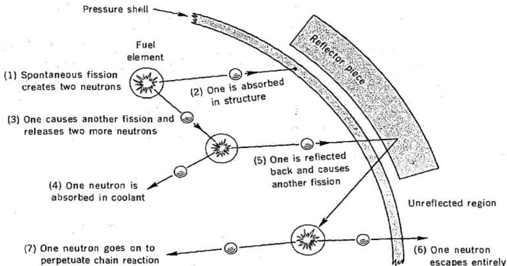
Figure 9 Neutron economy in a reactor core. The illustration assumes two neutrons are born in each fission. The reactor is just critical (self-sustaining) when each fission causes another fission.
