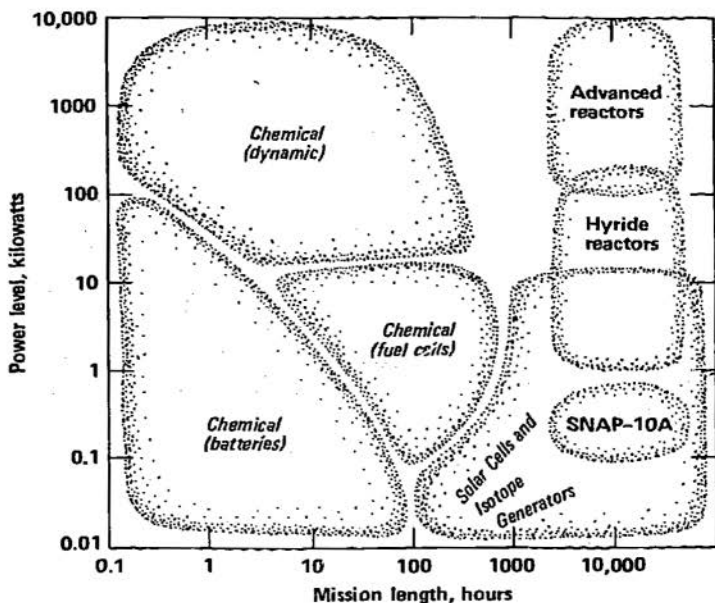
Figure 6 Areas of superiority for various space power plants. Generally, the higher the power level and the longer the mission, the greater the superiority of nuclear reactor power. Superiority on this chart means least weight.
