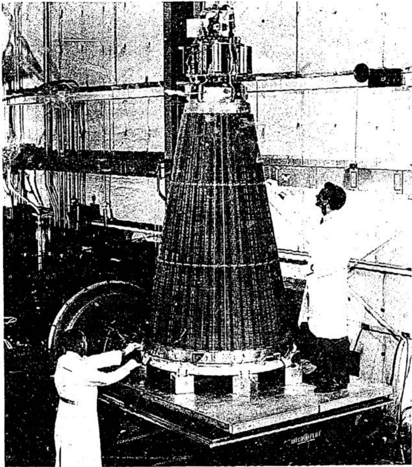
Figure 19 The complete SNAP-10A power plant showing the reactor perched on top of the conical radiator-thermoelectric element assembly (also shown on the cover). A rocket launch shroud surrounded this power plant during the launch period, but was blown off with explosive bolts once the reactor was in orbit.
