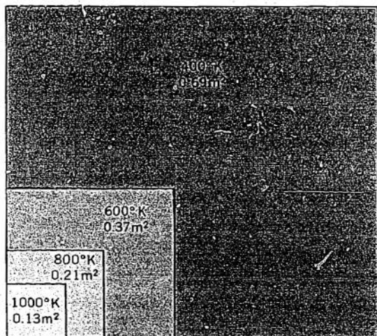
Figure 17 Relative areas required to radiate waste heat to empty space at different temperatures. Increasing the radiator temperature rapidly brings down area and weight. (Figures given are calculated for 1 kilowatt of heat and perfect emissivity.)
