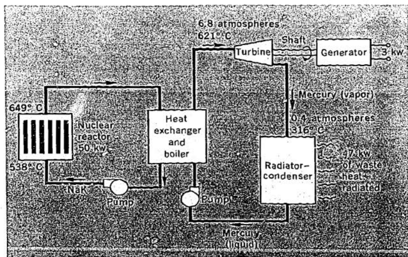
Figure 15 Schematic diagram of SNAP-2 nuclear power plant.
