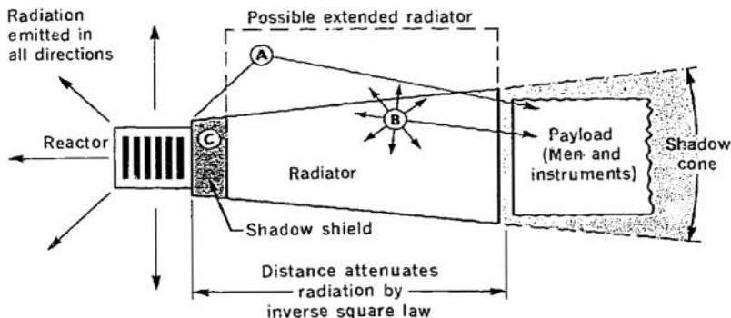
Figure 21 Shielding problems. Ordinarily, radiation is sufficiently attenuated by a shadow shield. In Case A, however, reactor-produced neutrons may be scattered off an extended radiator or another piece of equipment outside the shadow cone. In Case B, radioactive NaK in the radiator creates a new radiation source on the other side of the shadow shield. Case C shows radiation absorption in the shield.
