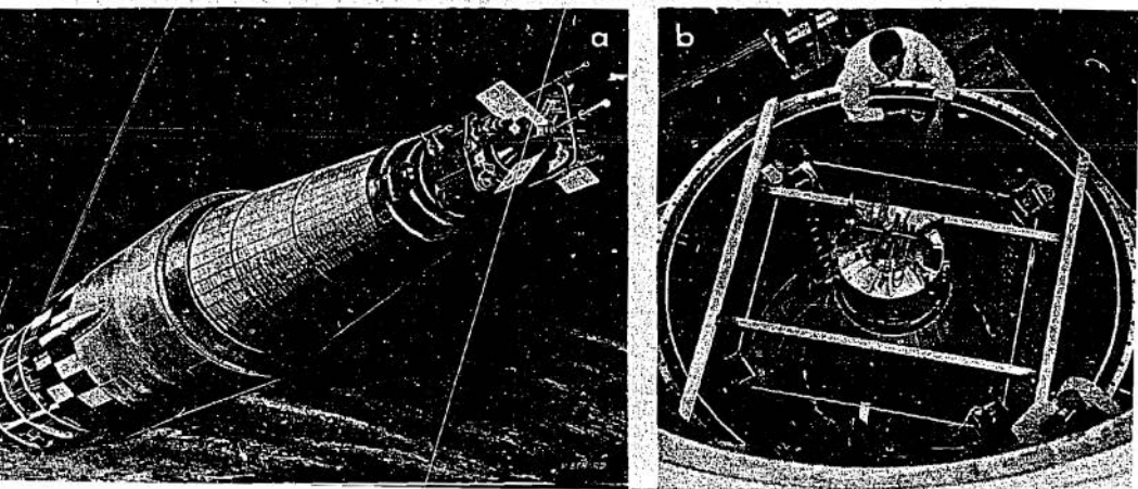
Figure 4 (a) SNAP-10A in orbit. It functioned successfully. (See cover.) (b) This earthbound counterpart generated electricity continuously under simulated space conditions for more than a year.
