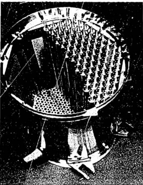
Figure 12 The SNAP-2 reactor. Movable reflector pieces vary the rate of power production.
