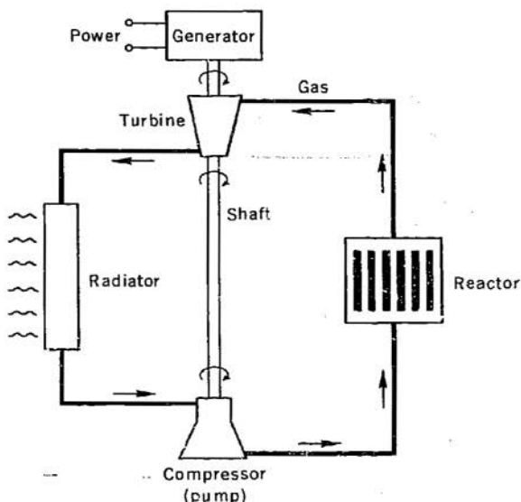
Figure 26 The Brayton cycle (gas-turbine cycle) nuclear space power plant.
