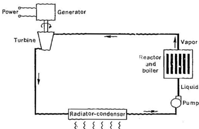
Figure 24 Schematic diagram of a power plant in which the liquid metal boils directly in the core. The intermediate heat exchanger and primary coolant pump of SNAP-2 and SNAP-8 are thereby eliminated.
