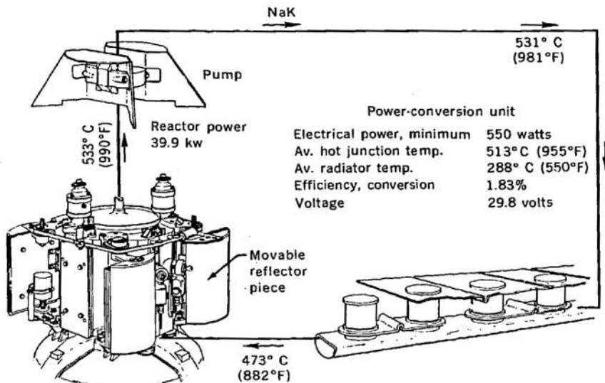
Figure 14 Schematic diagram of the SNAP-10 reactor and power-conversion unit.
