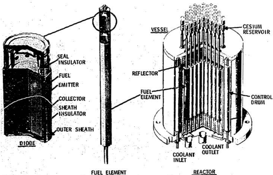
Figure 25 Thermionic diodes (left) can be assembled like flashlight batteries in long fuel elements (center). The elements are then arranged to make a reactor core as shown on the right.
