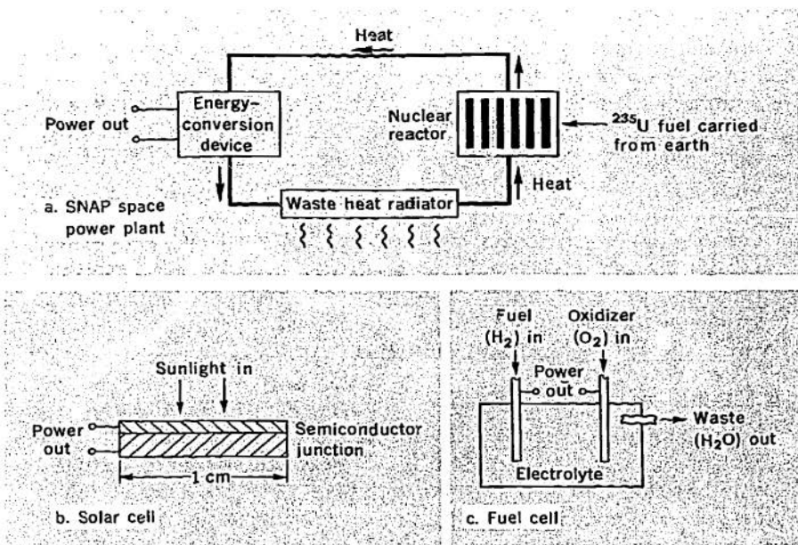
Figure 5 Comparison of important space power plants. In (a) SNAP converts fission-produced heat to electricity. In (b) the solar cell converts energy of photons to electricity. In (c) the fuel cell converts chemical energy into electricity.
