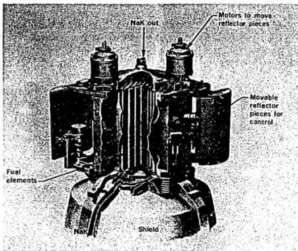
Figure 12 The SNAP-2 reactor. Movable reflector pieces vary the rate of power production.
