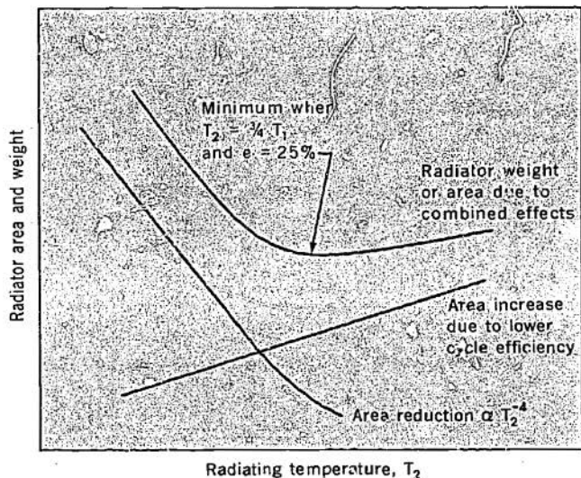
Figure 18 Sketch showing qualitatively how increasing the temperature ( T_2 ) decreases radiator area on one hand due to the Stefan-Boltzmann Law, but increases it on the other due to loss of cycle efficiency, as described by the Carnot efficiency equation. ( T_1 is assumed to be constant.)
