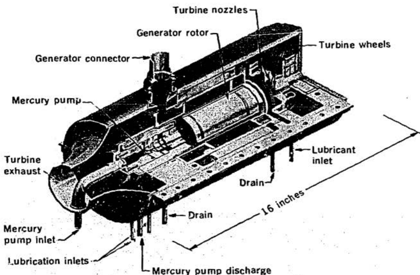
Figure 16 Combined turbine-generator-pump unit.
