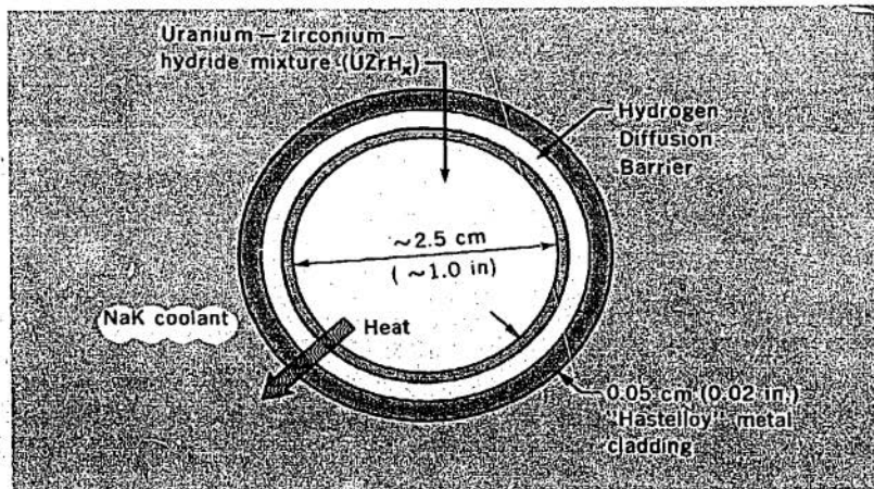
Figure 10 A typical fuel element for a SNAP hydride core reactor.
