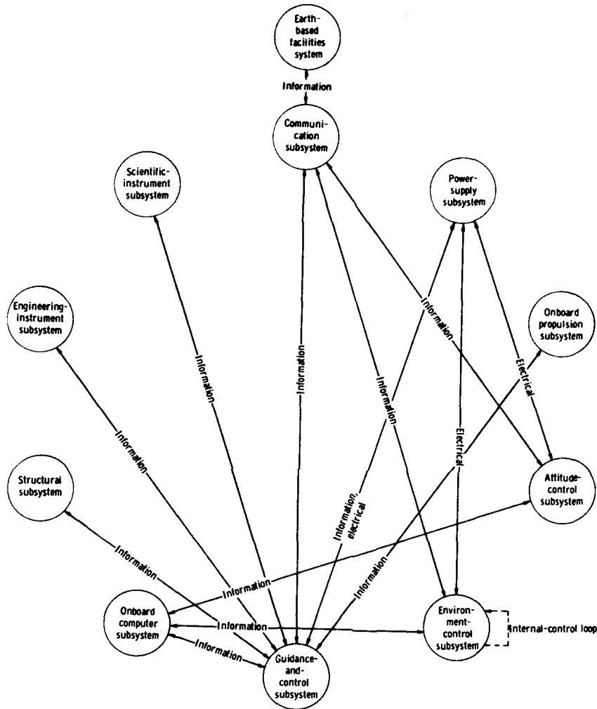
FIGURE 6-2.—Interface diagram showing the more important relationships between the three satellite-control subsystems and the remainder of the spacecraft. The information interface includes the transmission and reception of error and navigational information as well as commands.
