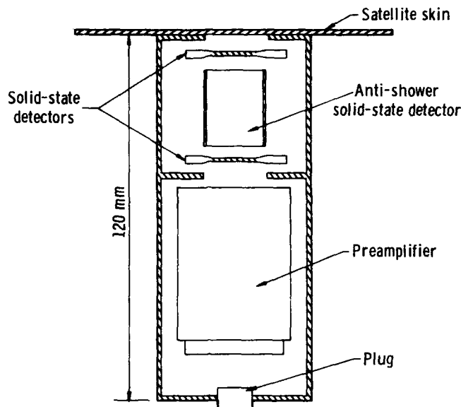
FIGURE 13-21.—Arrangement of solid-state detectors in the ESRO-2 cosmic-ray experiment of Labeyrie et al.
