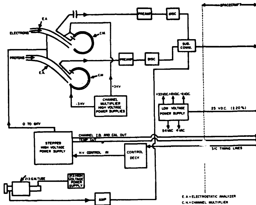
FIGURE 11-58.—Schematic of the OGO-B and OGO-E electrostatic analyzer shown in figure 11-57 (ref. 31).
