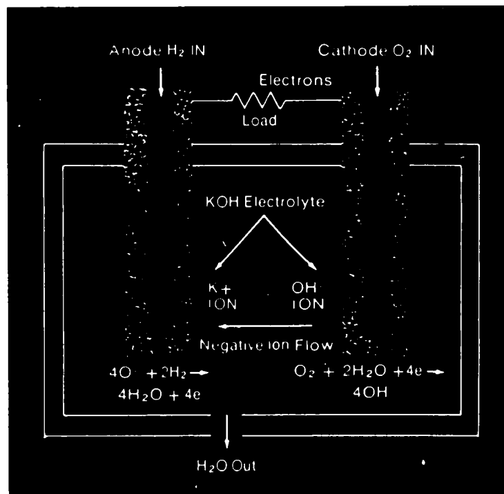
5 Schematic showing the operation of a hydrogen-oxygen fuel cell. The hydrogen and oxygen gases enter through porous electrodes.
