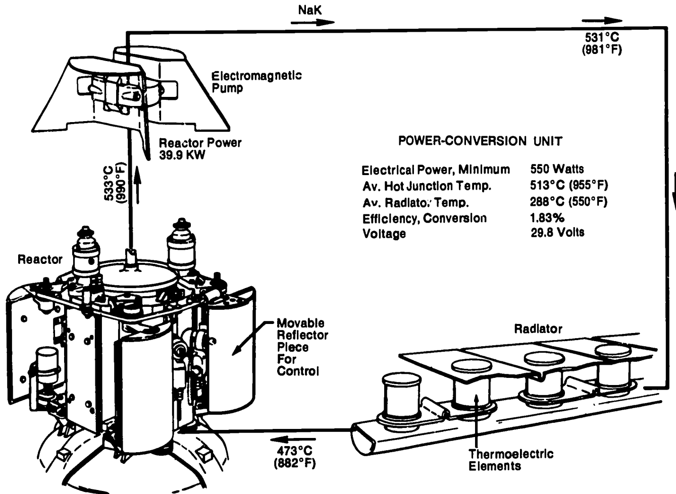
17 Schematic of the SNAP-10A reactor-thermoelectric power plant.
