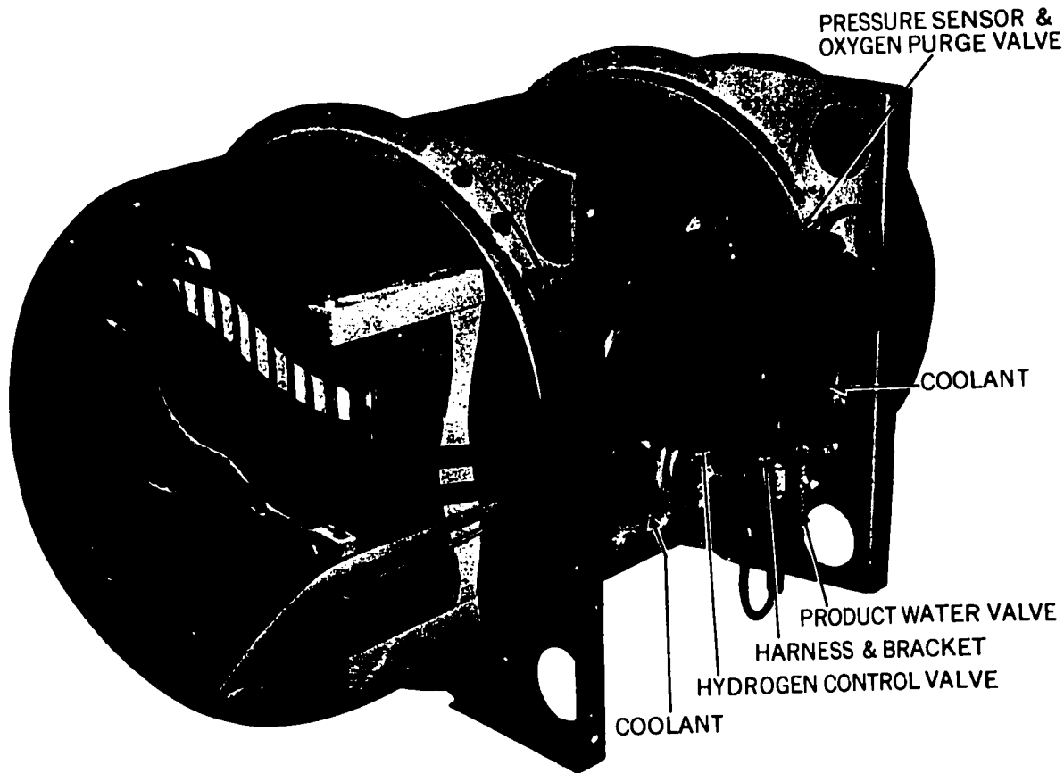
6 The Gemini fuel cell. Hydrogen and oxygen gases were "burned" in this fuel cell to produce electricity. The combustion product was water.
