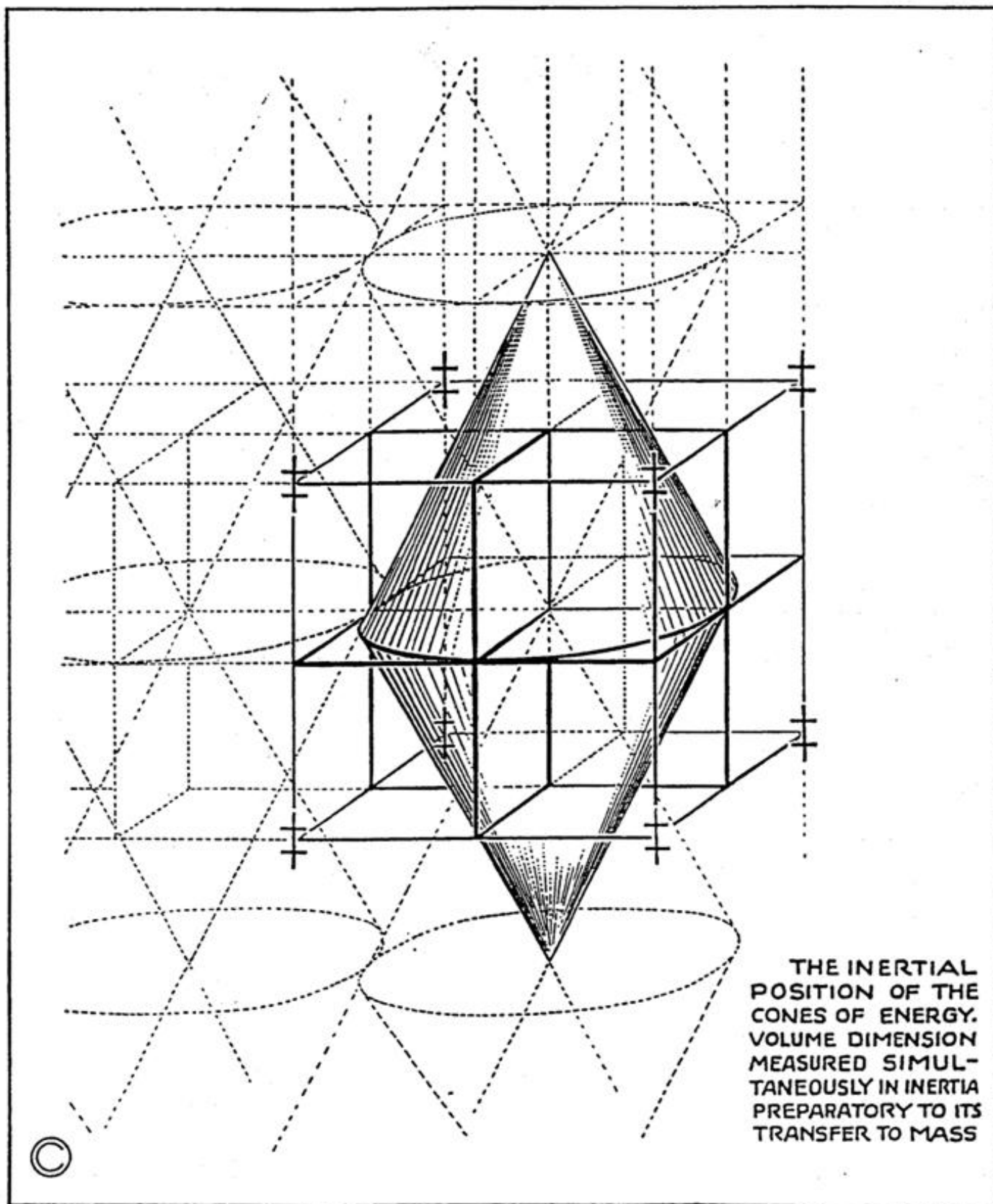
CHART DEFINING POSITION OF CONES OF ENERGY IN CONCEPT IN INERTIA. THE CONCEPT OF ENERGY IS UNIVERSALLY SIMULTANEOUS BUT ITS EXPRESSION IN MOTION IS SEQUENTIAL.
