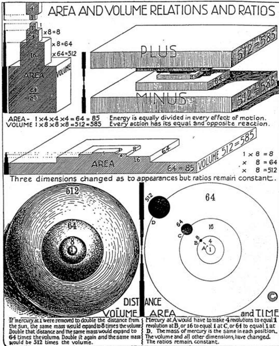
DIMENSION CHART No. 3. THE UNIVERSAL REPRODUCTIVE CONSTANT NEVER VARIES ITS RATIOS NO MATTER WHAT THE WAVE DIMENSION OR THE ACCUMULATION OF POTENTIAL. DIMENSIONS OF MASS CHANGE BUT THE RATIOS AND RELATIONS NEVER CHANGE
