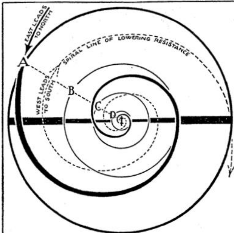
POTENTIAL RATIOS FOR RIGID MASS
