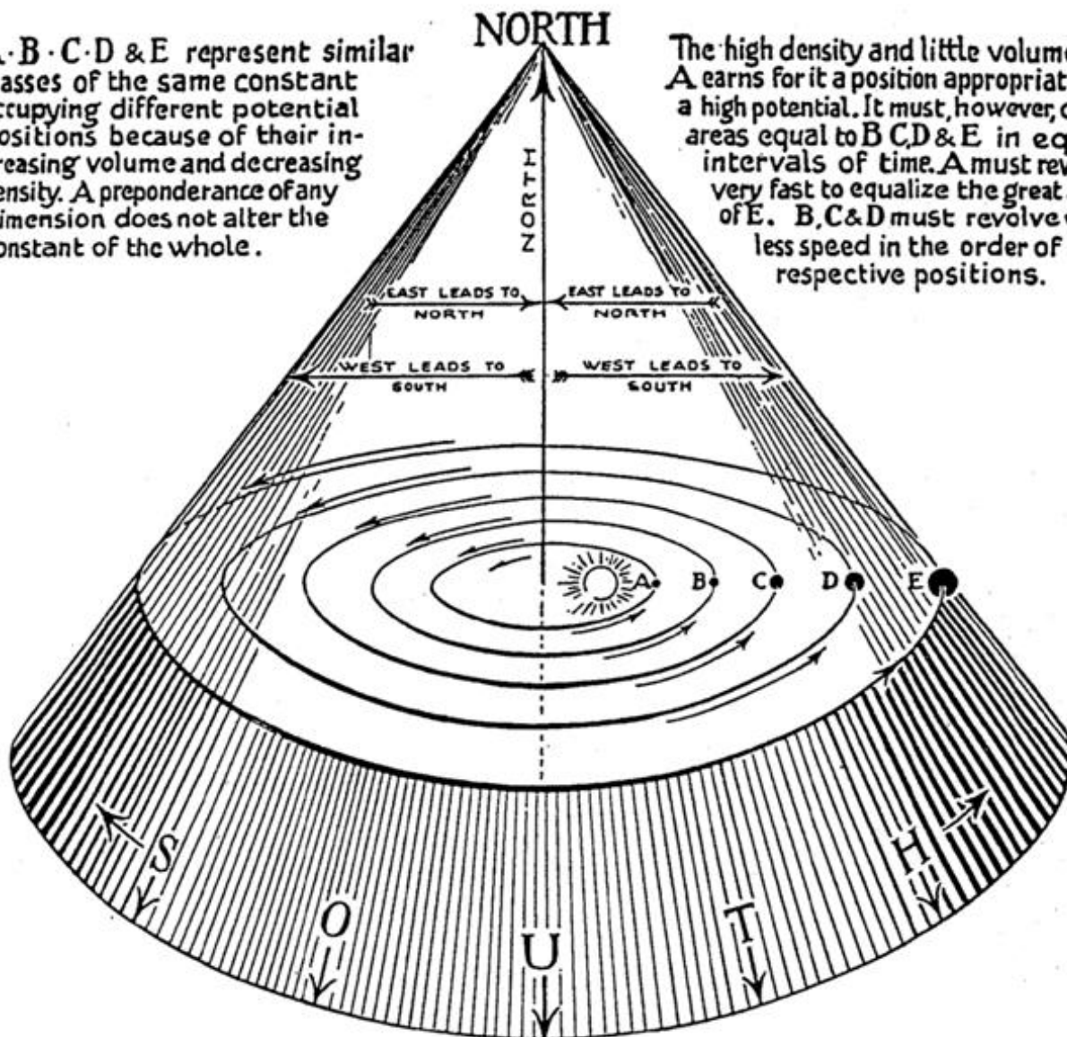
THESE ORBITS ARE DRAWN WITHOUT REGARD TO VARIATION OF PLANE
