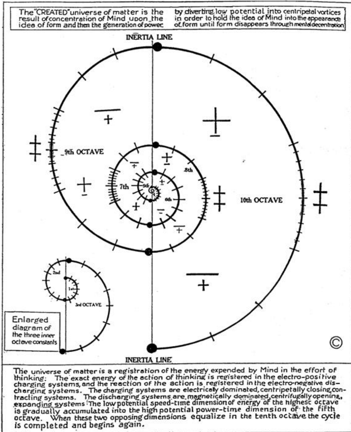
DIAGRAM OF THE TEN OCTAVE CYCLE OF INTEGRATING AND DISINTEGRATING LIGHT UNITS INTO ATOMIC SYSTEMS CALLED THE "ELEMENTS OF MATTER"
