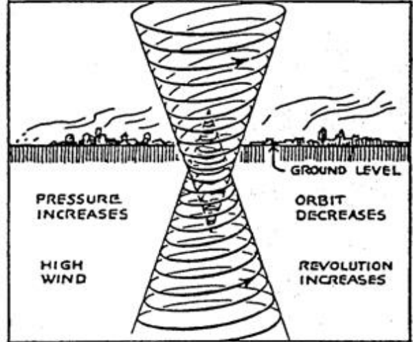
Energy is generated in contracting cones.
