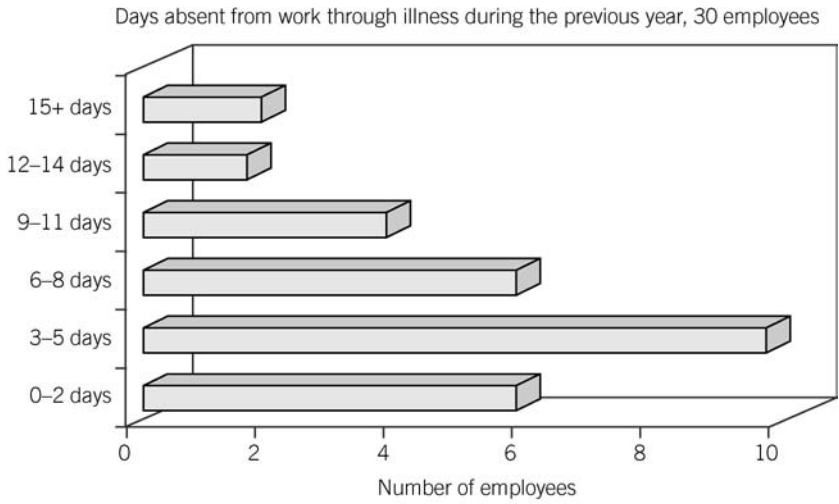
FIGURE 15 Horizontal bar chart example
