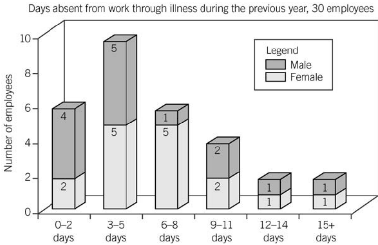
FIGURE 16 Stacked bar chart example
