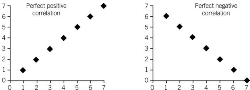
FIGURE 10 Correlations and scatter plot examples
