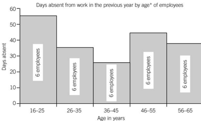
FIGURE 17 Histogram example
