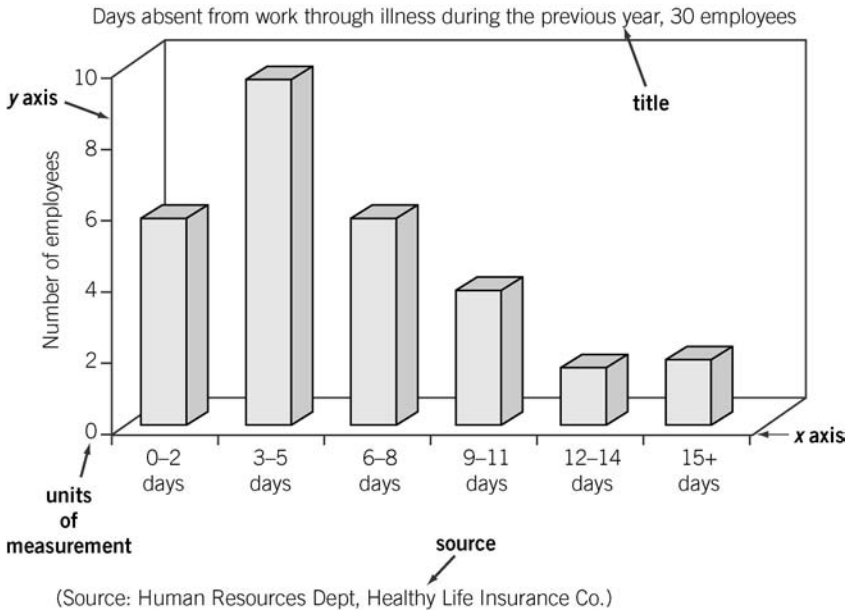
FIGURE 14 Simple bar chart example
