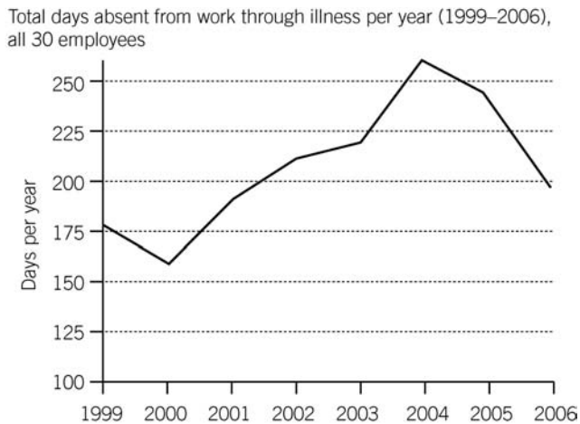
FIGURE 19 Line graph example
