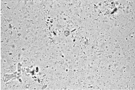
Fig. 7.2 Cyclospora oocysts in stool ×640
