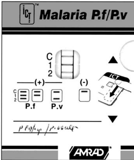
Fig. 3.8 Positive immunochromatographic test for mixed P. vivax and P. falciparum malaria
