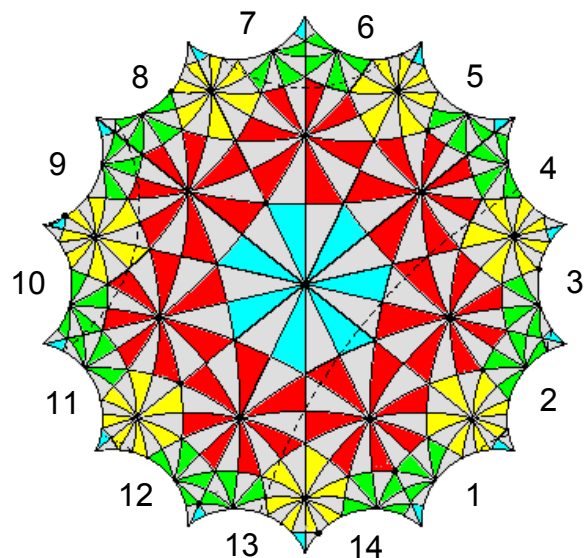
Figure 25. The Klein Configuration of the 168 elements of the group of transformations of the Klein Quartic equation.
