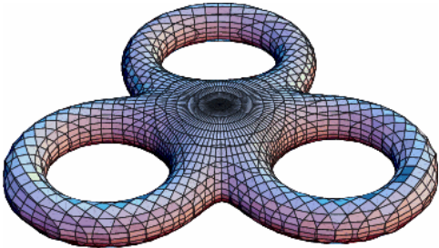
Figure 26. The 3-torus.
