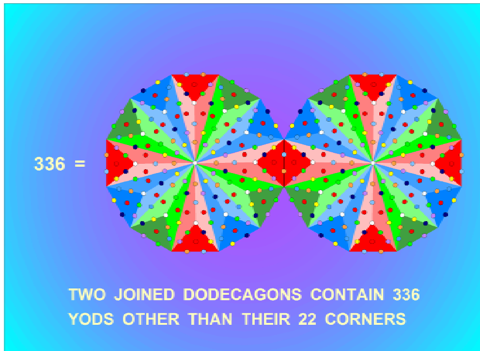
Figure 21. The last of the regular polygons in the inner form of the Tree of Life, the pair of dodecagons each acquire 168 yods when their sectors are divided into three tetractyses. Each yod symbolises a turn in a half-revolution of a whorl of the UPA and an element of the group PSL(2,7) .
