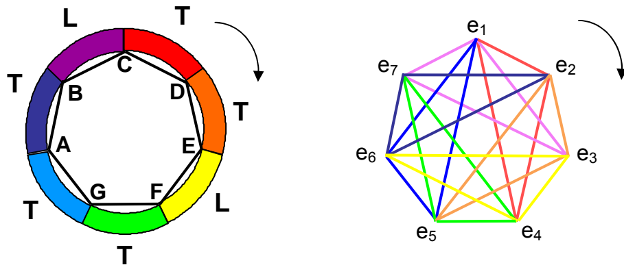
Figure 27. Comparison of the 7-fold musical scale and the 7 imaginary octonions.
