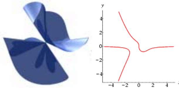
Figure.24. The Riemann surface of the Klein Quartic. (From: http://Mathworld.wolfram.com ).
