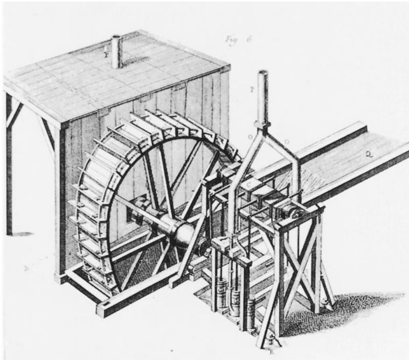
Fig. 10.1. Water power. Europeans began to use wind and water power on an unprecedented scale. Undershot waterwheels were constructed at many sites along the profuse streams with which Europe is favored.
