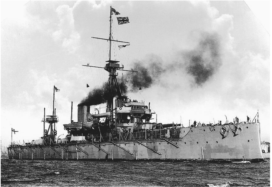
Fig. 15.4. The Industrialization of War. Launched in 1906, the HMS Dreadnought was the most formidable armored battleship of its day. With a main battery of ten 12-inch guns, driven by a steam turbine powerplant, and capable of a speed of 21 knots, this revolutionary vessel surpassed every previous warship in design and military capability and was testimony to the might of industrial civilization in Britain.
