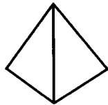
Tetrahedron
