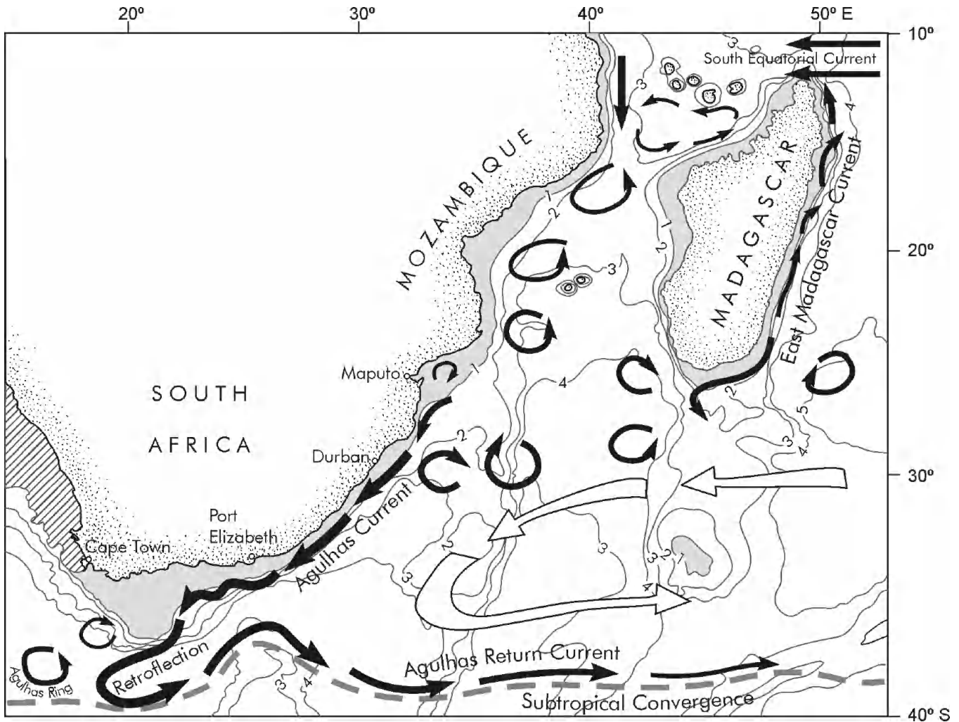
Agulhas rings that reach the South Atlantic Ocean and shed their heat, salt, and vorticity to the ambient waters are part of what makes the Agulhas Current a profound factor in both local weather and the global climate.
