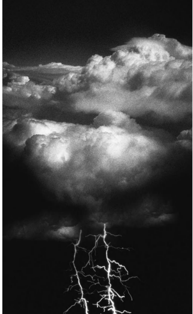
Worldwide, it is estimated that 50,000 thunderstorms occur every day, and over 18 million occur per year.
