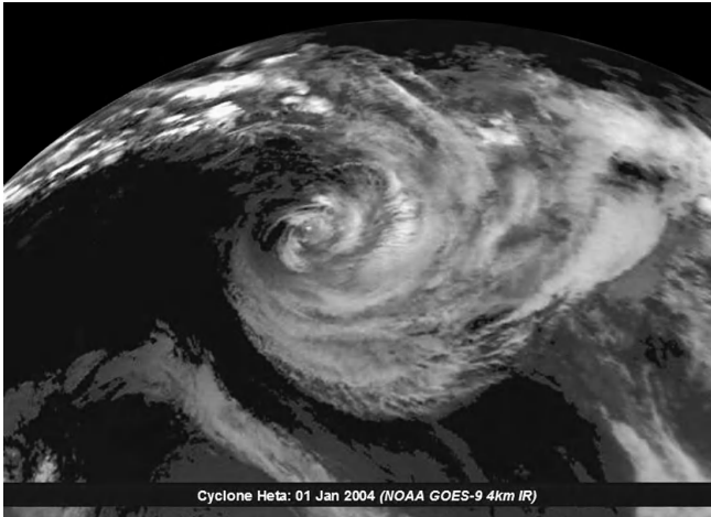
Cyclone Heta: 01 Jan 2004 (NOAA GOES-9 4km IR)
