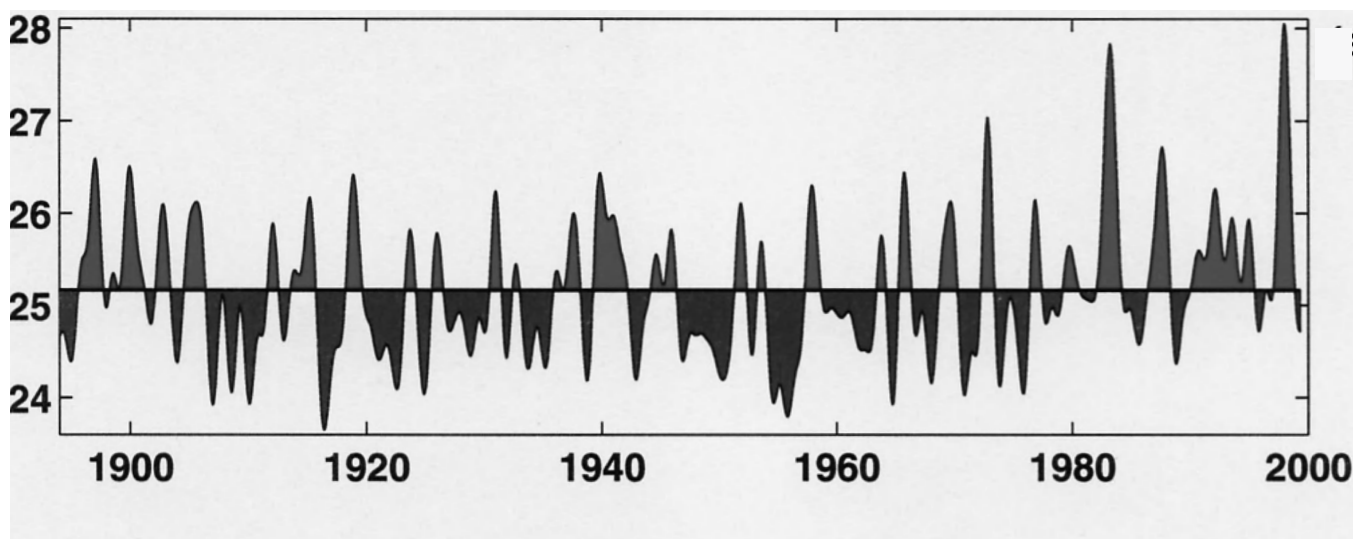
Oscillations in sea surface temperatures (in degrees Centigrade) over the past century, in the eastern equatorial Pacific Ocean (after removal of the seasonal cycle.) El Niño conditions prevailed during the periods in lighter gray above the 25 degree C line, La Niña during the periods in darker gray below the 25 degree C line.
