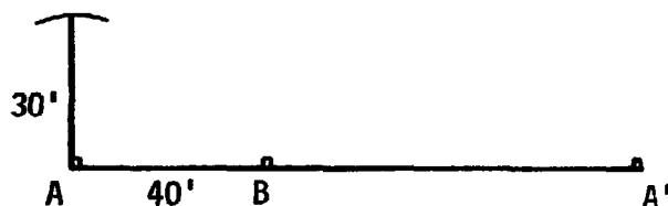
FIGURE IX-A. LAYING OUT A RIGHT ANGLE
