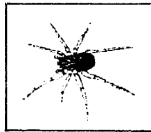
beneficials
