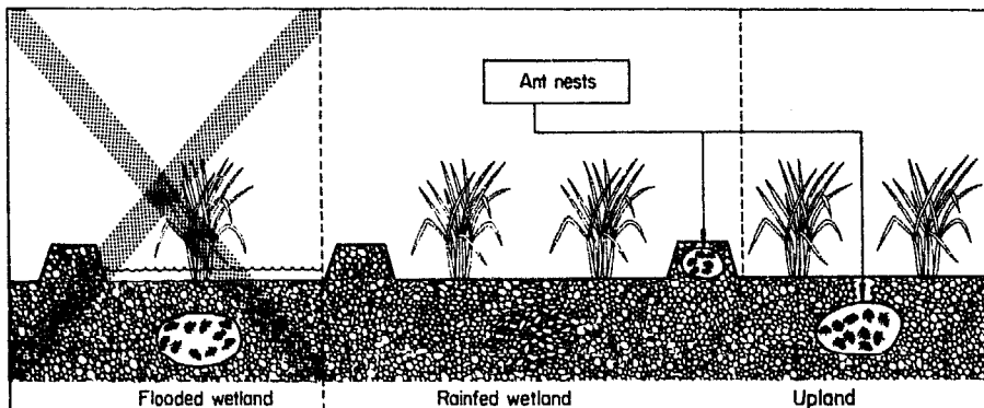
Rainfed wetland
