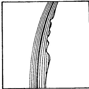
• Ragged leaves
