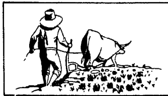
cultural control
