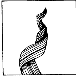
• Twisted leaves
