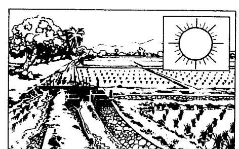
Irrigated wetland
