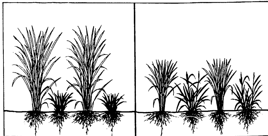
Traditional cultivar
