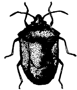
Scotinophara coarctata
