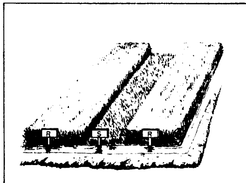
resistant varieties
