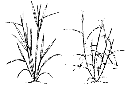
Wild rices
