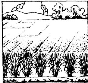
Cultivated rice
