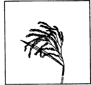
• Unfilled grains
