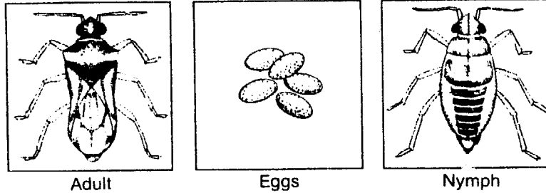
Adult
