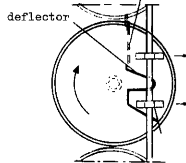
Fig. 118 - Plate distributor
