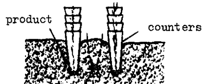
Fig. 120 - Different depth placement components fitted to planters
