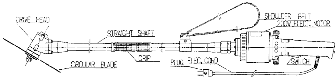
"CeCoCo" Portable Electric Cutter Model FC-2
