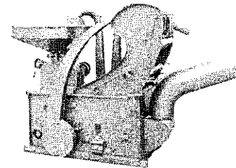
"CeCoCo" Rice Huller Model Automatic "AM"
