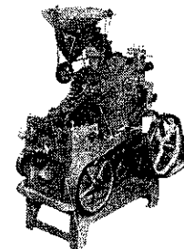
"CeCoCo" Automatic Machine-Screw Making Machine
