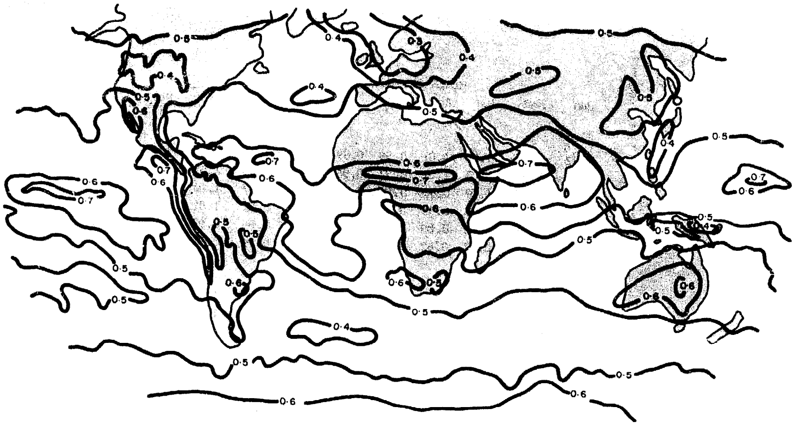
Figure A1. Clearness Index Map for January
