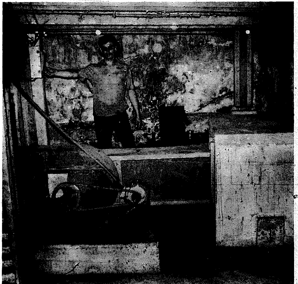
The furnace, at right, is connected to the centrifugal blower by a duct. The control switch in the upper left-hand corner should be located near the control for the rice hulls.
