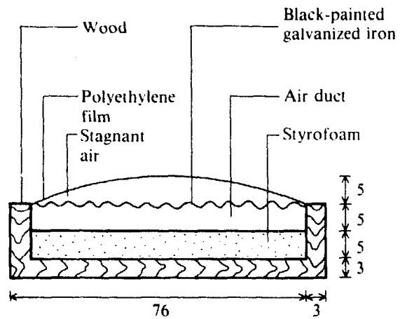
Fig. 3. Cross section of solar collector (experiment C) (dimensions in centimeters).
