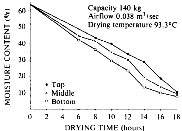
Fig. 8. Coffee berry drying curves with an initial moisture content of 64% and airflow rate of 0.038 m 3 /sec.
