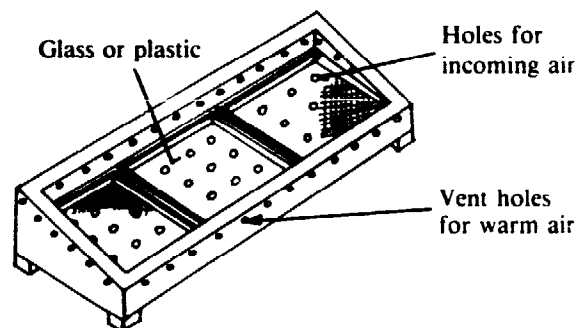
Fig. 2. Diagram of a typical direct dryer.
