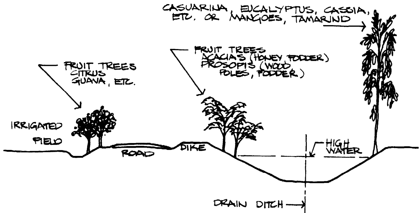
TREES ALONG DRAINAGE STRUCTURE
