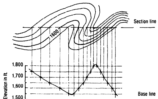
Fig. 177. How a section is drawn.
