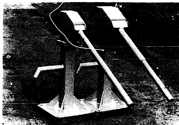
Fig. 116. SWN 80 and SWN 81 handpumps.
