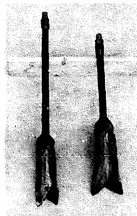
Fig. 141. Stone augers.
