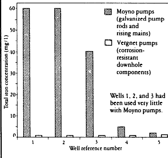
Figure 4.3B Changes in Iron Concentrations in Well Water due to Substitution of Corrosion-Resistant Pumps
