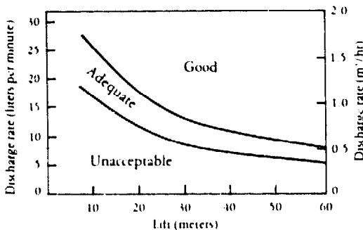
Box Figure 5.1A Variations in Pump Discharge Rate with Pumping Lift
