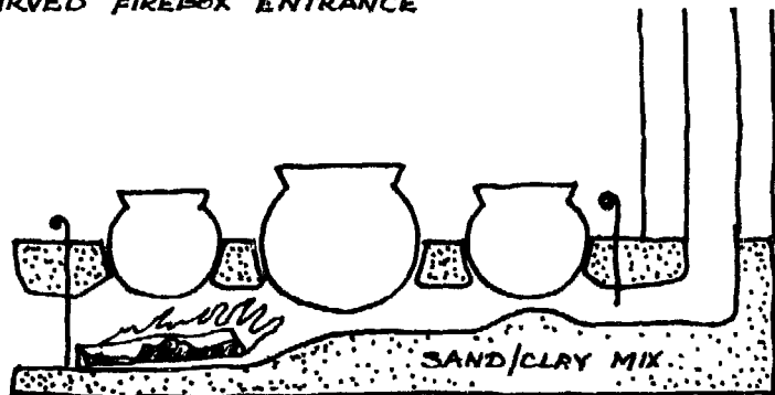
SECTION ALONG TUNNEL
