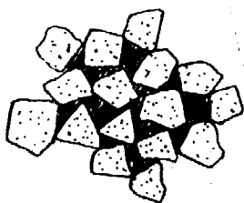
SAND GRAINS BIND TOGETHER. SHRINKING CLAY CAN'T SHRINK THE WHOLE MASS
