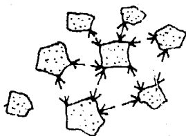
SAND GRAINS APART LEAVE ROOM FOR CLAY TO SHRINK ALONG ARROWS
