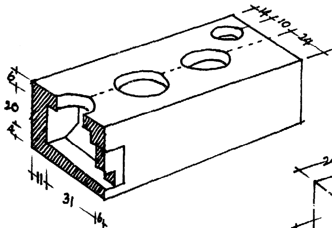
CROSS SECTION THROUGH FIREBOX
