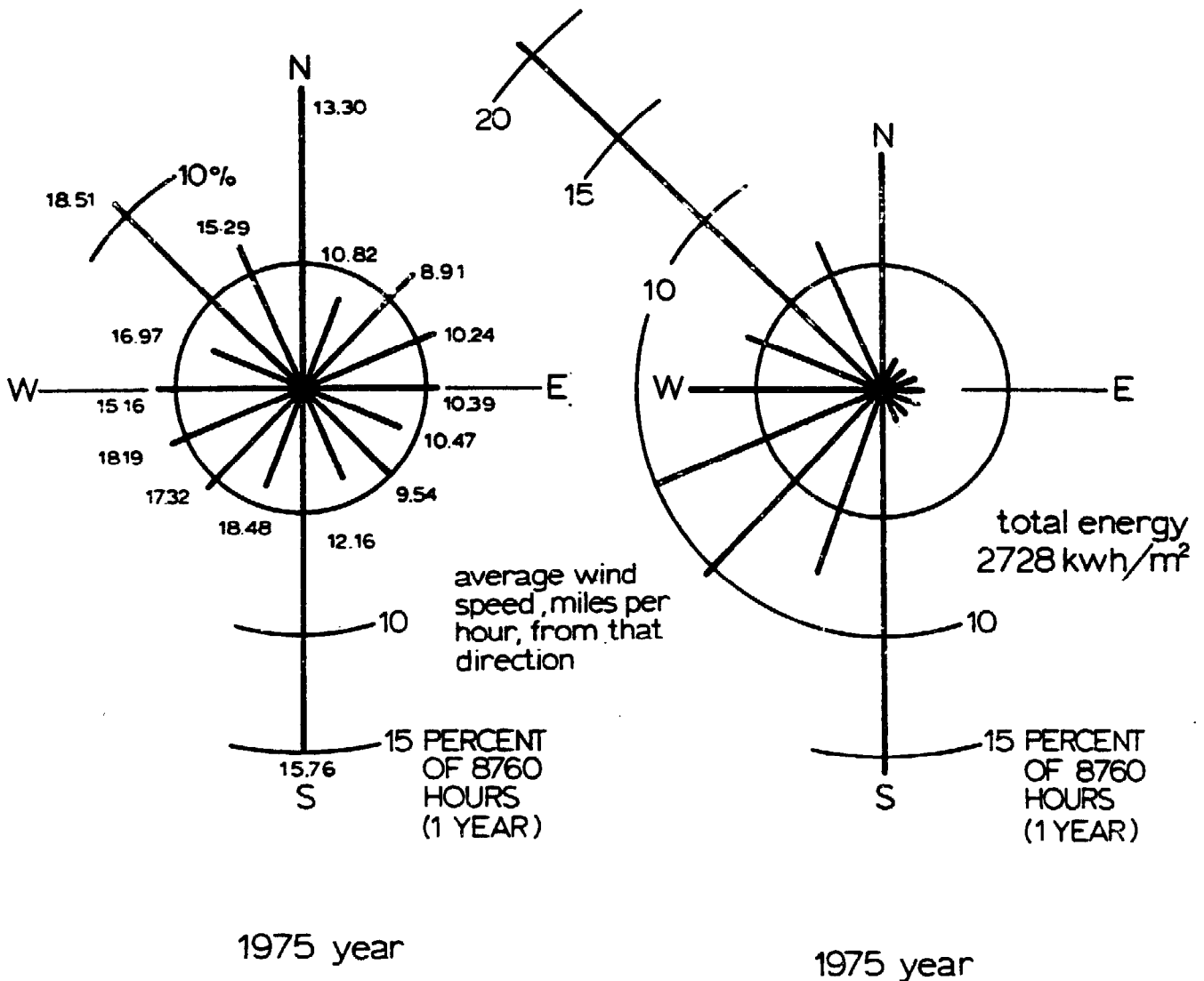
FIGURE 3-5: Wind rose for Muskegon Coast Guard Station, Michigan, at 30 meters.
