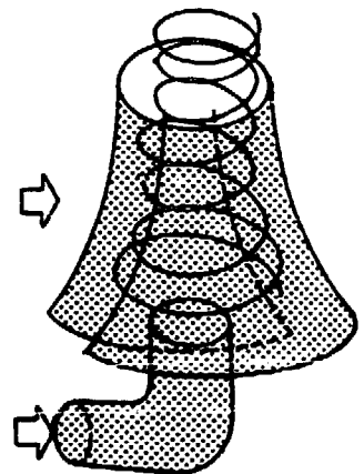
CONFINED VORTEX
