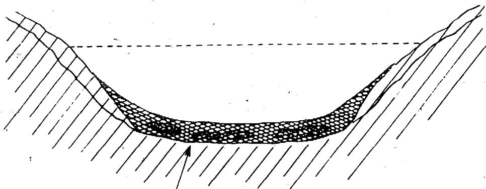
Trench under proposed crest of dam extends into canyon sides far enough to remove pockets of gravel lodged there.
