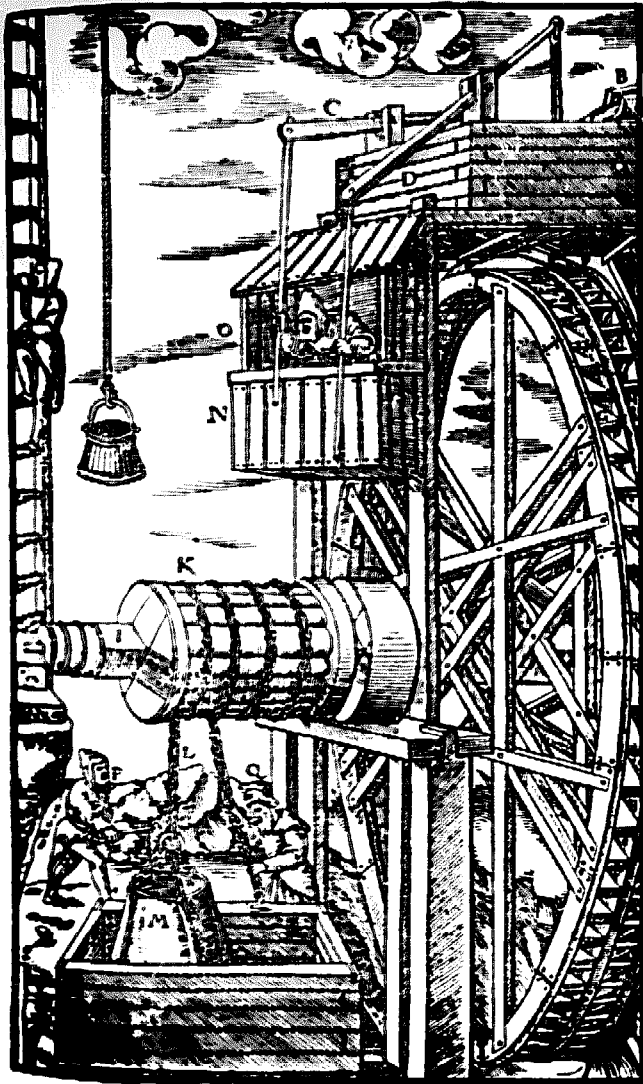
fig. 39: Axle used as a winding drum. A: Reservoir E: Race C, D: Levers F, F: Troughs under the water gates G, H: Double rows of buckets I: Axle K: Larger drum L: Drawing-chain M: Bag N: Hanging cage
