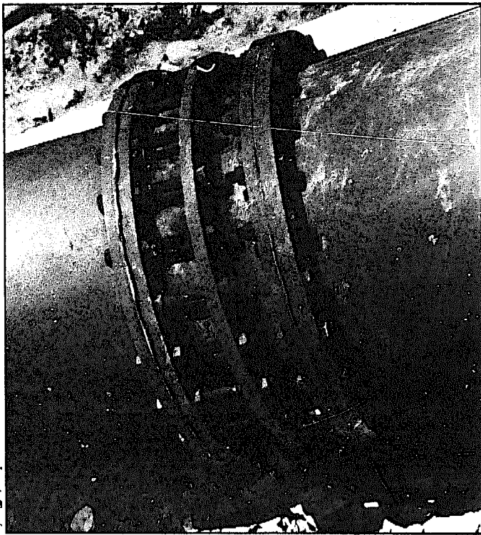
Fig. 5.134. A sliding-type expansion joint.
