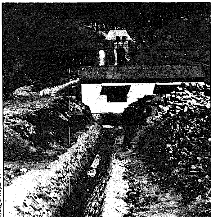
Fig. 5.25. This tailrace will carry water from the powerhouse back to the stream. The short penstock can be seen behind the powerhouse (also see Fig. 5.121).
