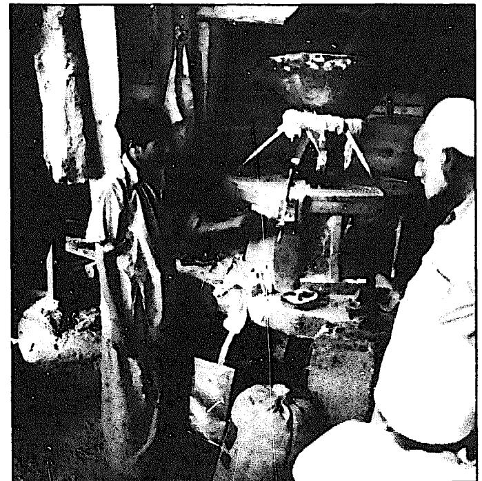
Fig. 10.46. Turbines at a number of powerhouses are directly coupled to flour milling equipment.
