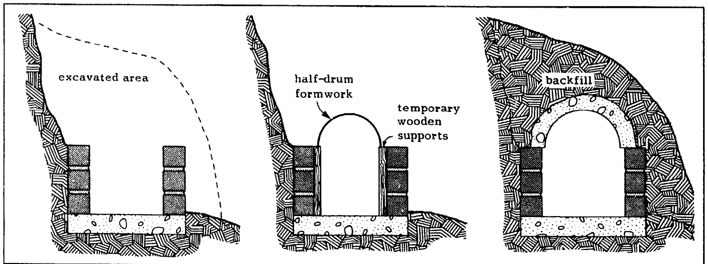
Fig. 5.105. Steps in the construction of a covered stretch of canal at Bundi, Papua New Guinea (Source: B. Vögtli).
