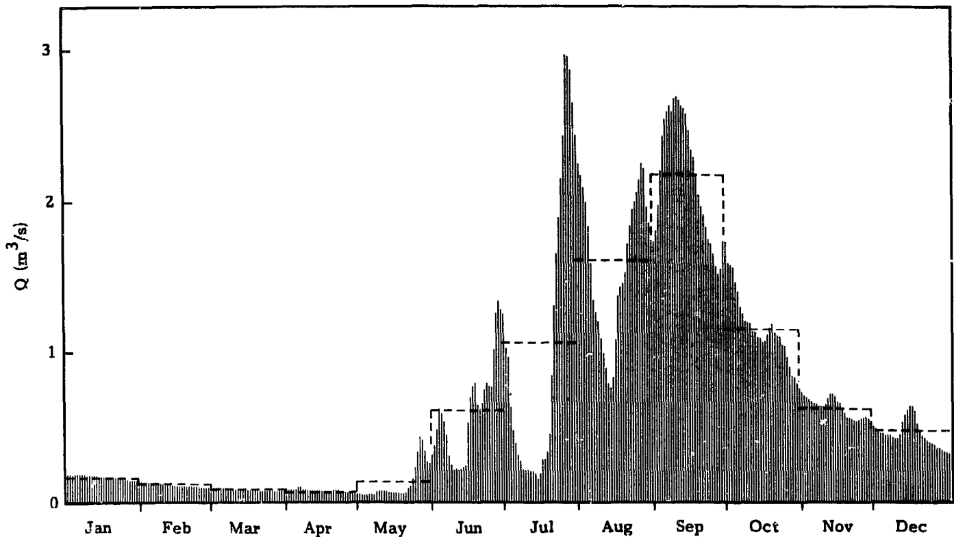
Fig. 3.2. A typical flow hydrograph. The dashed lines indicate average monthly flows.
