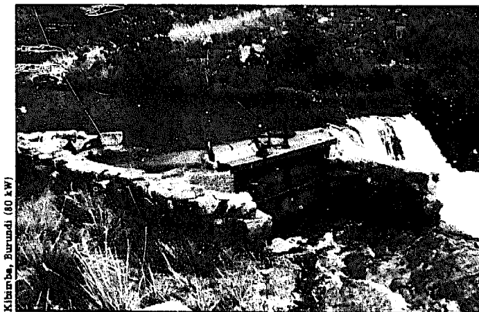
Fig. 5.52. Only a gate followed by a spillway is used at the intake at this site.
