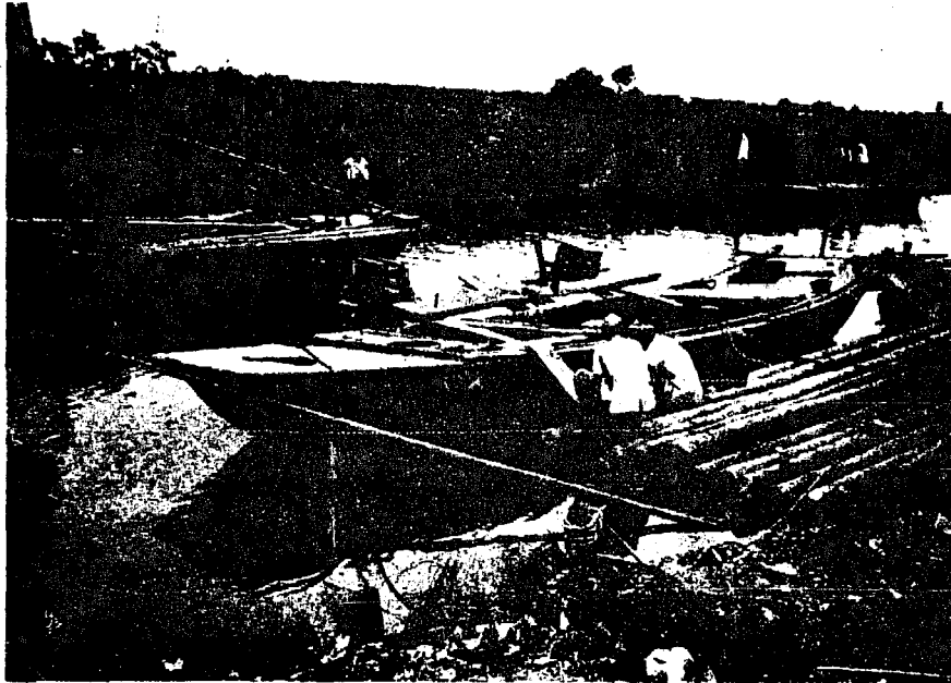
FIGURE A-2 Repairing a damaged ferroceement hull. In the background are wooden counterparts.
