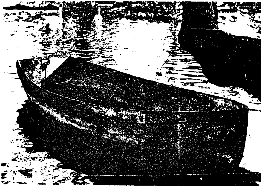
FIGURE 7 Built in 1887, this Dutch ferroceement boat was still afloat, in 1967, at the Amsterdam Zoo. ( Cement , Amsterdam, The Netherlands)
