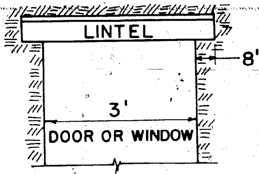
Figure 95. Wood lintel.
