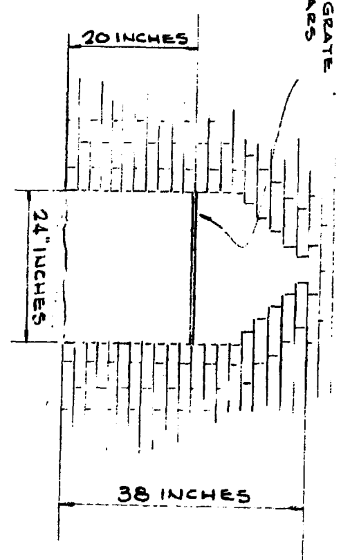
FRONTAL VIEW OF THE FIREBOX
