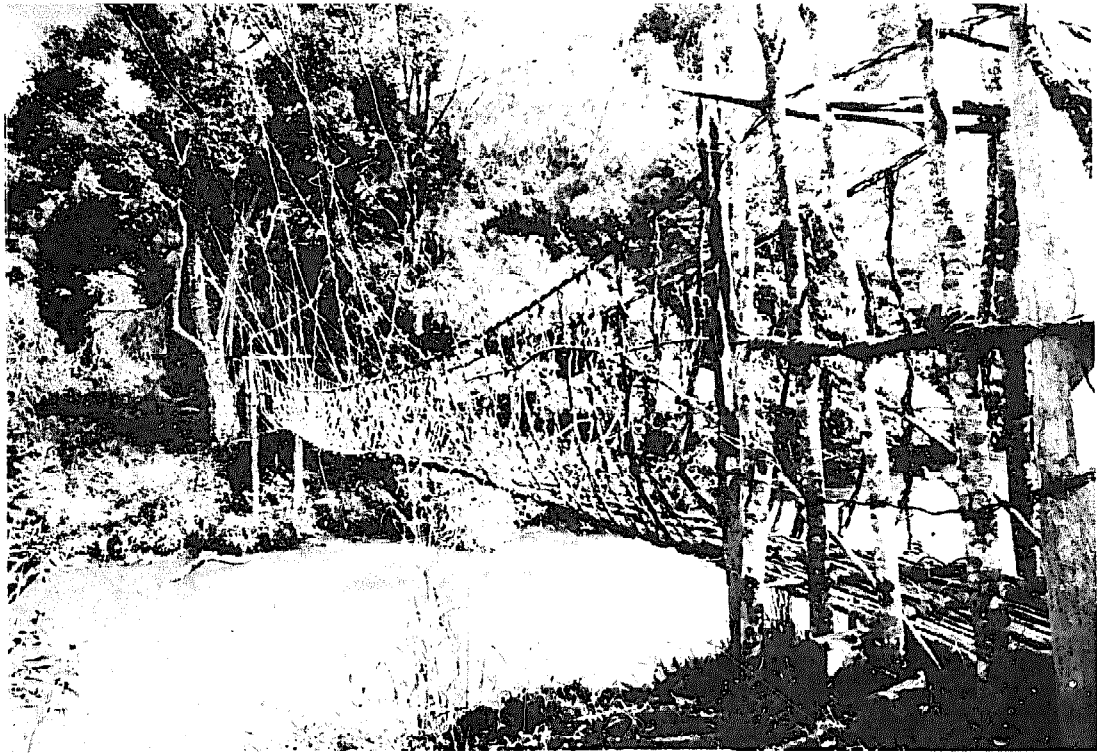
Fig. 48 Another view of Pulumita Bridge.
