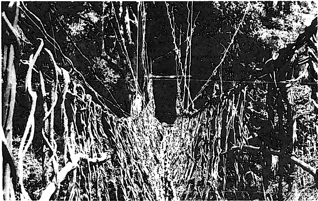
Fig. 49 Pole walkway (facing north) with vine spanning cables and suspenders, Pulumita Bridge. A recently added steel cable can be seen in the upper left hand corner.
