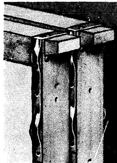
Metal-spaced frame
