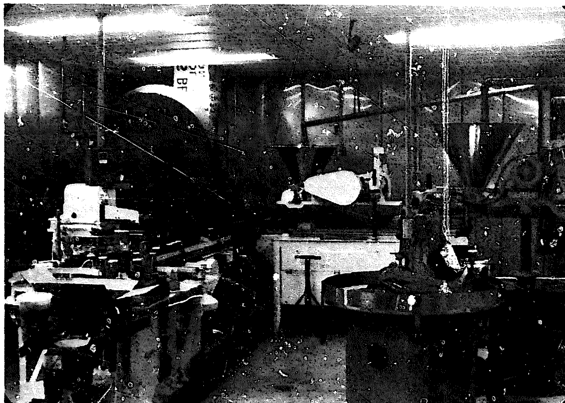
Bottling proceeds smoothly on a continuous conveyor moving from left in picture to right where the filled jar is capped. Note funnel-shaped automatic honey measuring devices. — Photo courtesy of Stewart Honey Bee Products
