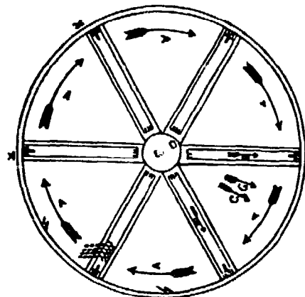
Fig. 4—Diagram of radial extractor from Gleanings in Bee Culture , October 1, 1888.
