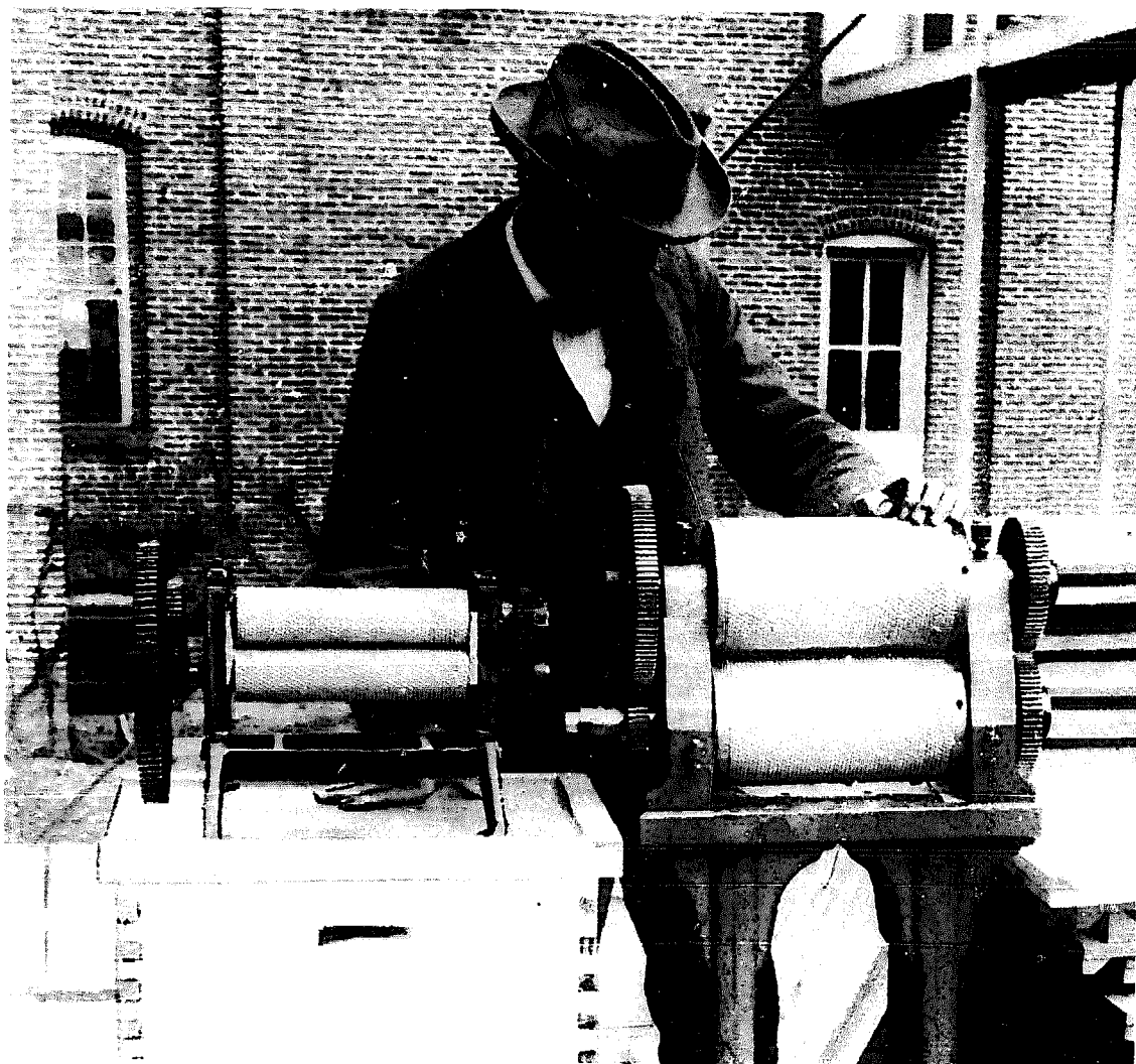
A 2½-inch roll and a 10-inch roll foundation mill with Mr. E. B. Weed standing in the background. The large mill has its angle reversed so that the parallel walls are horizontal instead of vertical as shown in Fig. 2 on page 185. See text.
