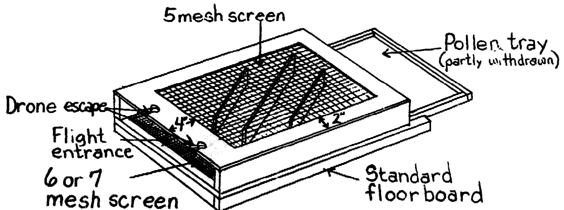
O.A.C. pollen trap.
