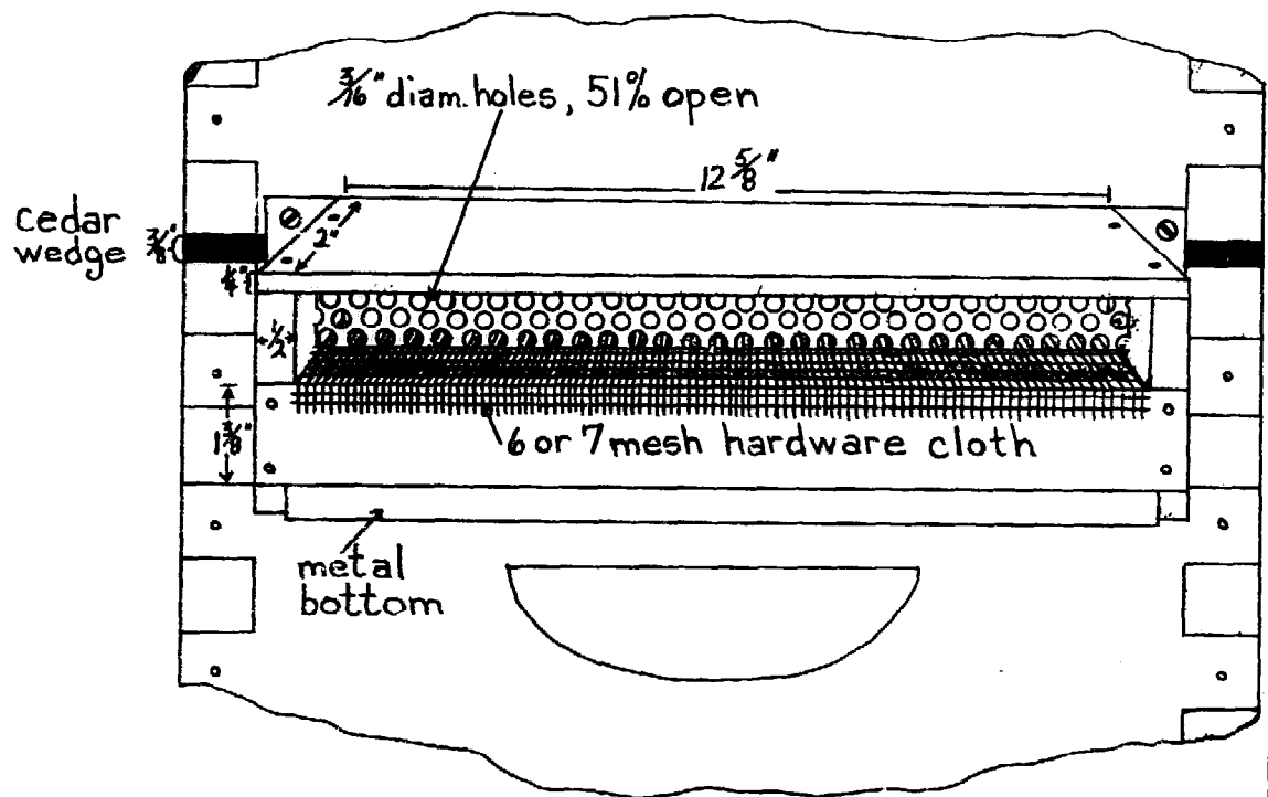
Modified pollen trap, front view.
