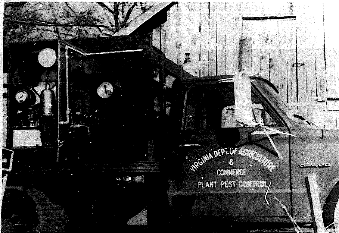
Truck-mounted fumigator used in Virginia. Control box showing gauges which indicate temperature and pressure, the measuring flask on hanging scale and the battery which powers vacuum pump. Note white frost on piping, past vaporizing valve.
