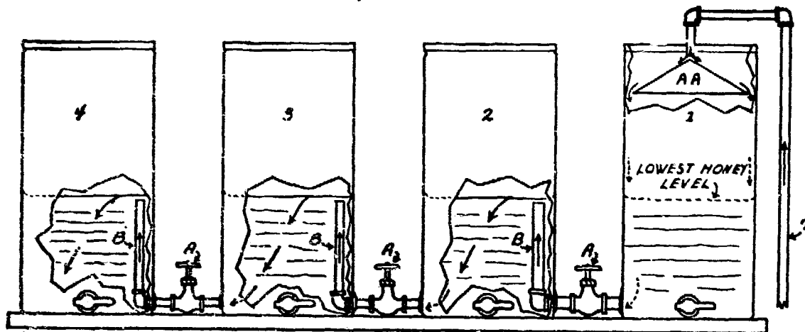
The Gardner Hook-Up of Four One-Ton Settling Honey Tanks.
