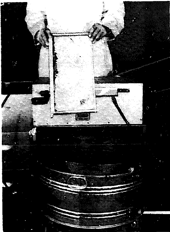
One-blade power uncapping machine. Part of the honey drains into the tub and is pumped directly into the storage tank. Note the pipe at the bottom leading to the honey pump.
