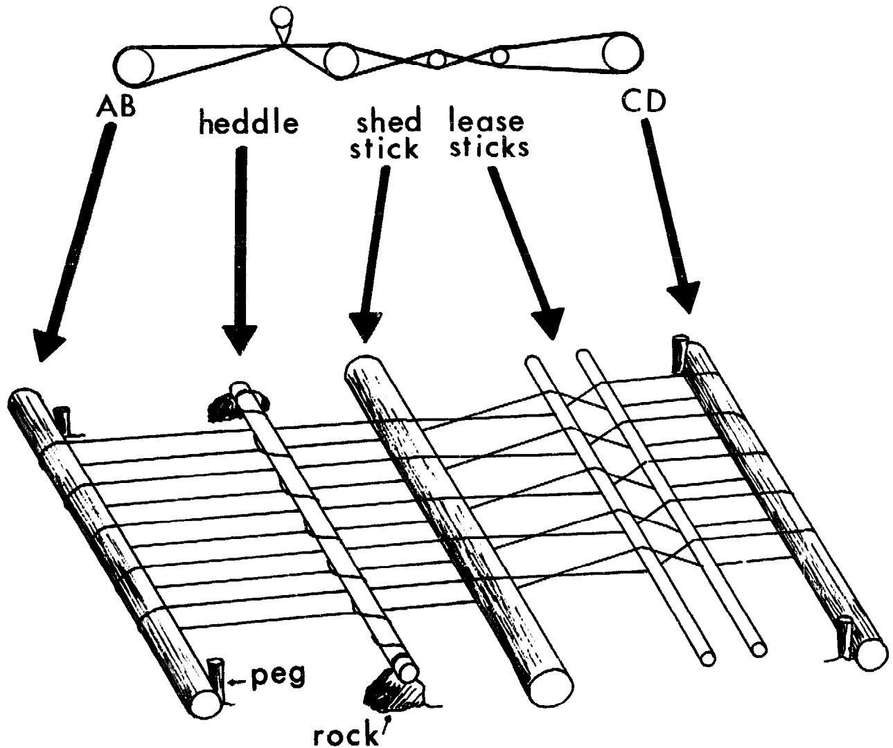
Side View (above) and Schematic view (below) - Peg Loom - showing working parts in position and pegs in place.
