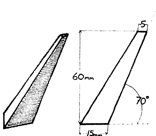
Fig. 2-141: Shape and dimension of cones
