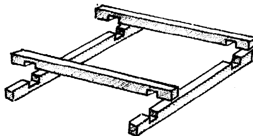
Fig. 1-26: Separable wooden frame for slab-making. The sticks have the thickness of the slab.
