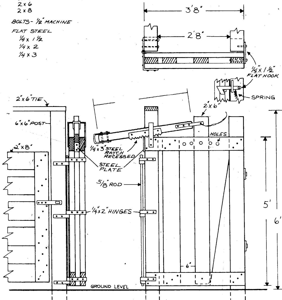
Figure 1. Headgate
