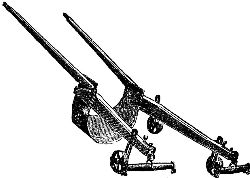
FIG. 199. The Bragg tree-digger.
