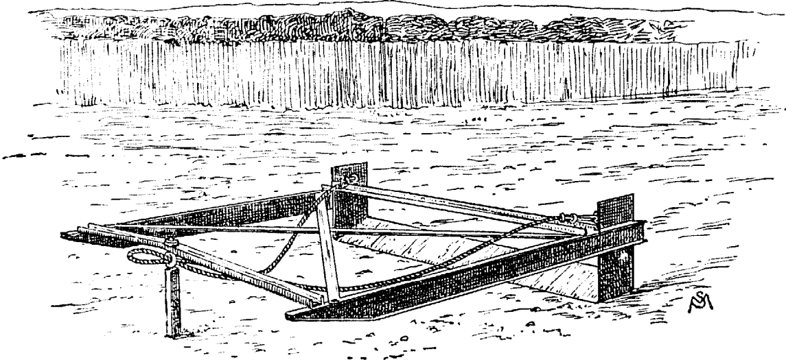
FIG. 202. Tree-digger for a forest-tree nursery.
