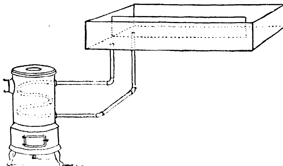
FIG. 83. Barnard's propagating-tank.
