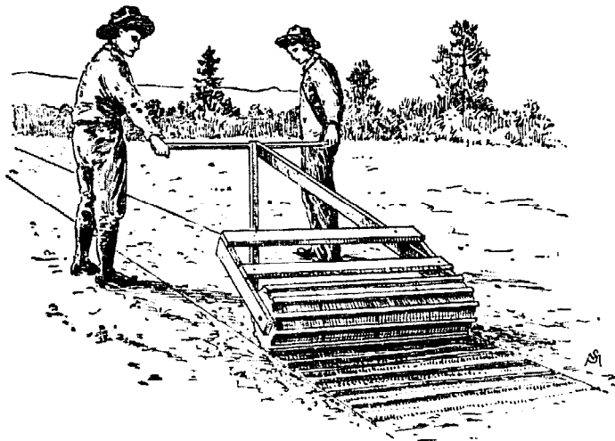
FIG. 32. Concrete marker-roller.
