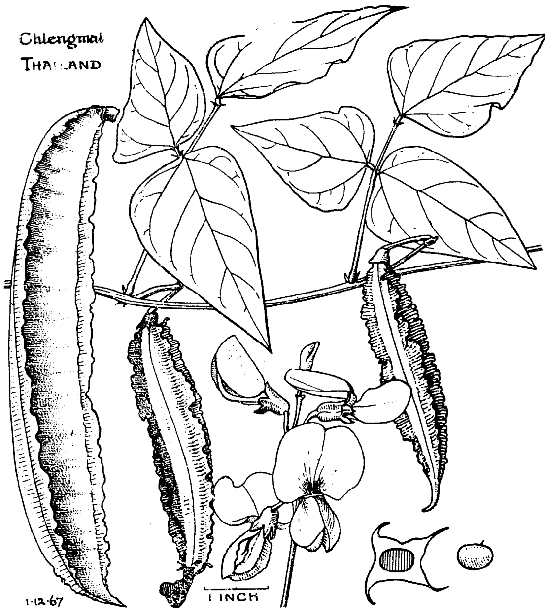
Psophocarpus tetragonolobus : winged bean. Leaves, inflorescence with pale blue flowers and buds, and young and mature pods. The insets on the right are of a cross section of an old pod and seed. (Based on a drawing by G.A.C. Herklots)
