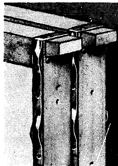
Metal-spaced frame
