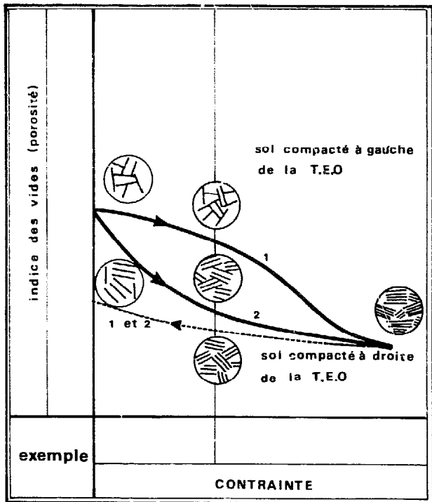
FIGURE 277 : COMPRESSION - DECOMPRESSION
