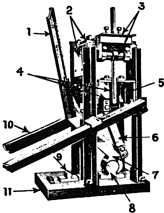
FIGURE 225 : LA PRESSE ELLSON BLOCKMASTER
