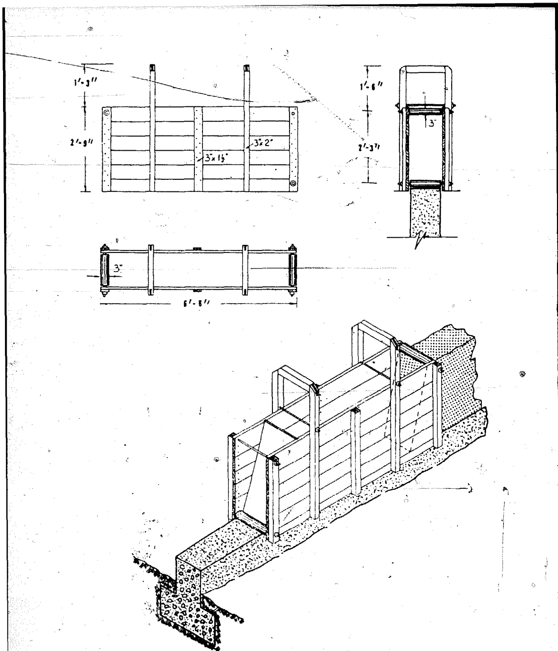
Figure 77. Form for ramming.
