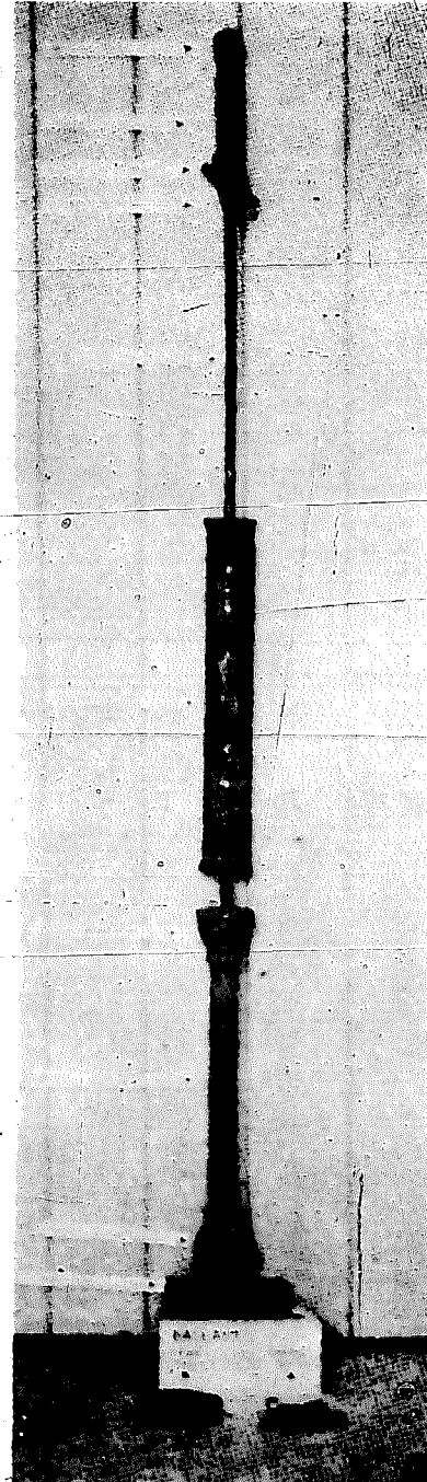
Figure 79b. Assembled sliding weight tamper.
