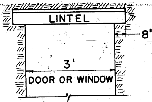
Figure 95. Wood lintel.
