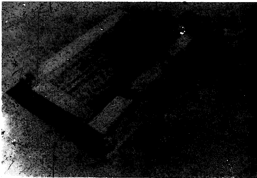
Figure 67a. This 2" x 4" wood nailer block, of the same dimensions as an adobe block, is inserted in place of the adobe block around windows and doors to offer an excellent, rigid hanger for the window or door frame.
