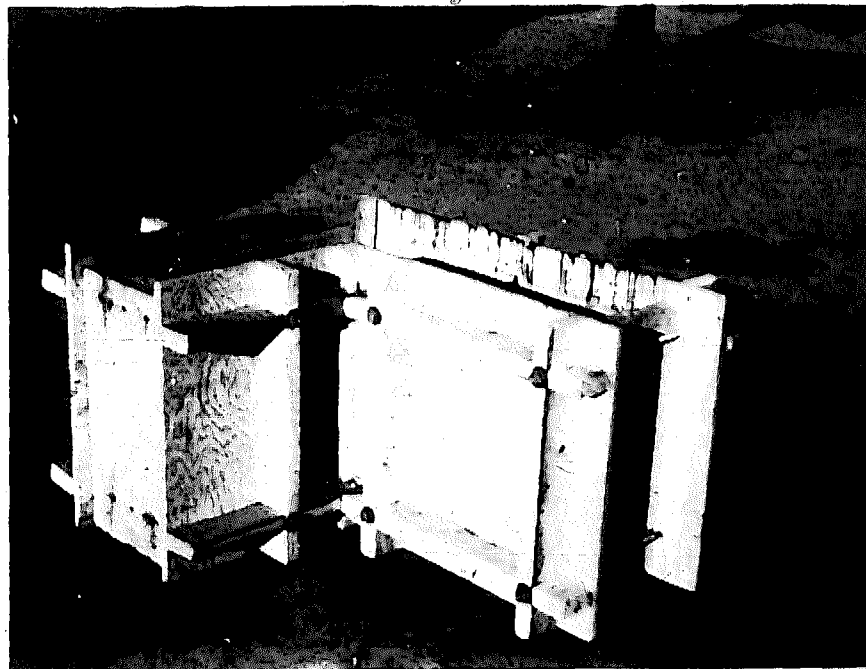
Figure 74. Plywood corner form for rammed earth walls.
