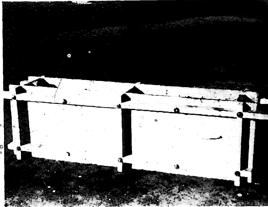
Figure 73. Straight form for rammed earth walls.
