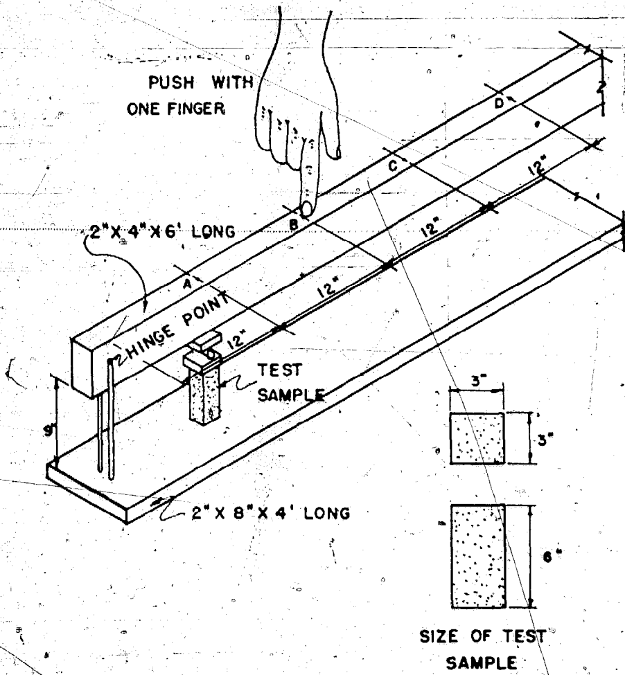
Figure 94. Simple lever tester for soils.
