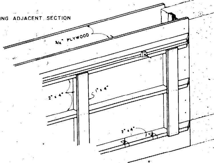
Figure 76. This is a special form that was designed to use the metal tie strips shown in Figure 75.
