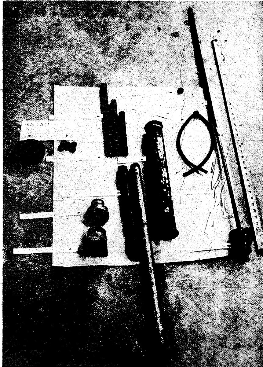
Figure 79c. Disassembled sliding weight tamper.
